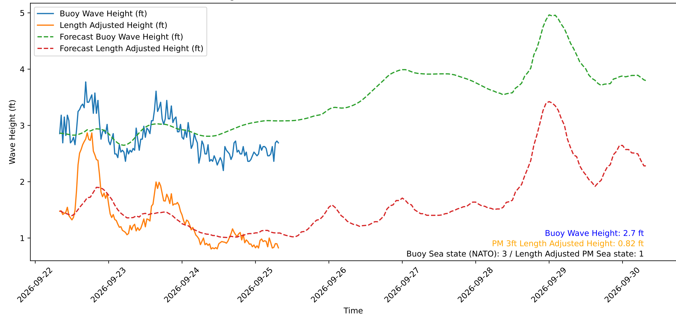
Wave Heights over Time for Oceanside Harbor at 2026-09-25 08:00:30
