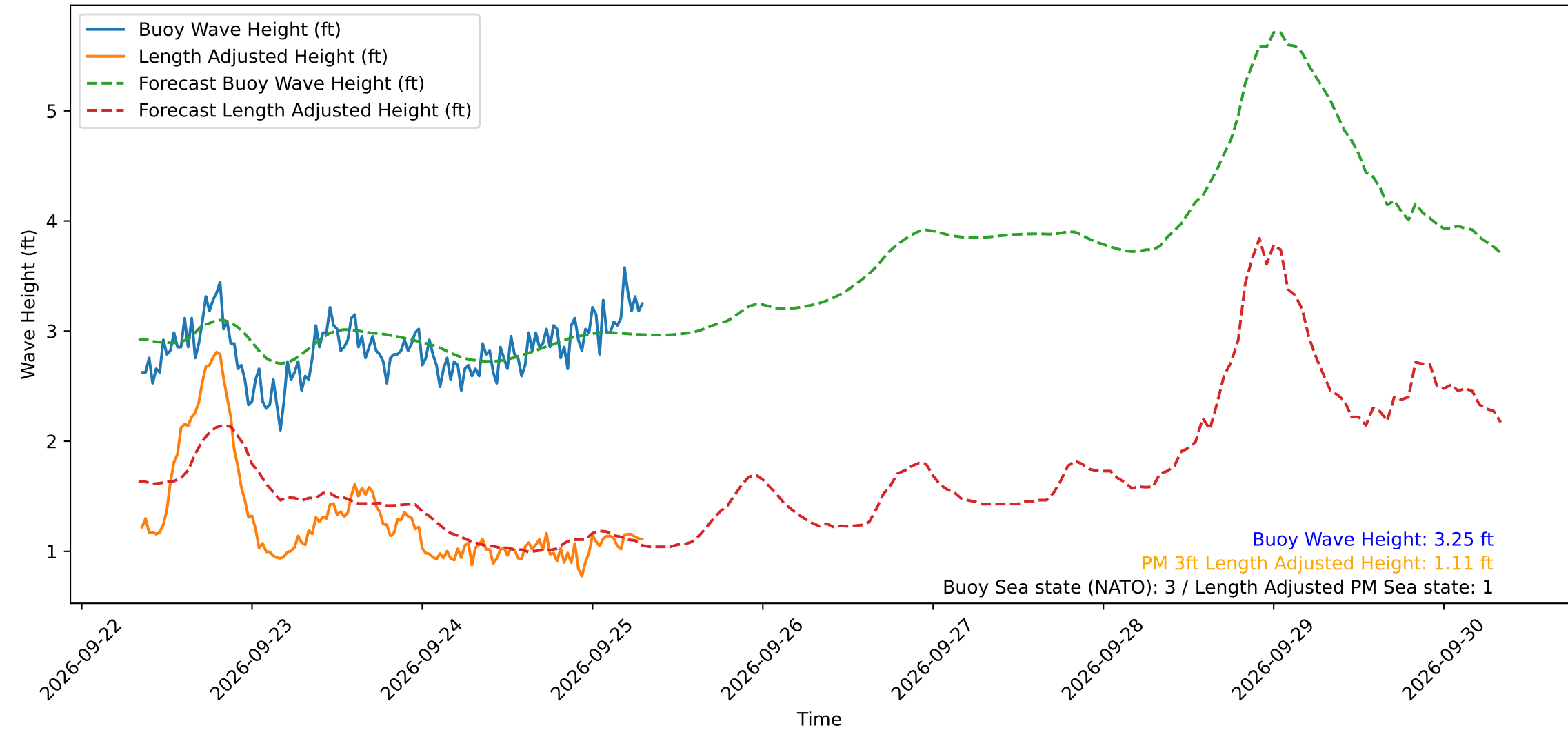
Wave Heights over Time for Green Beach at 2026-09-25 08:01:12
