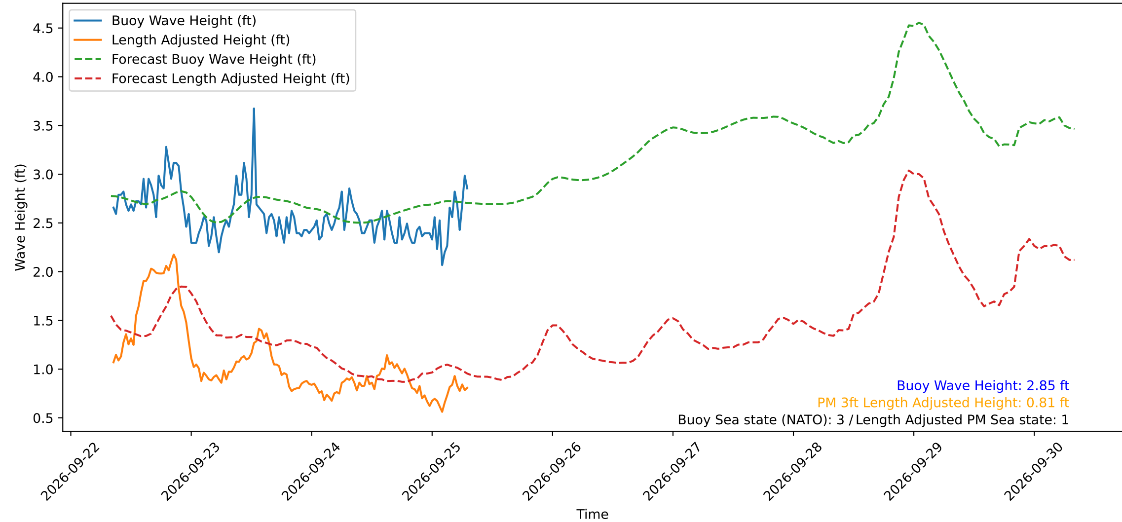
Wave Heights over Time for Red Beach at 2026-09-25 08:00:49
