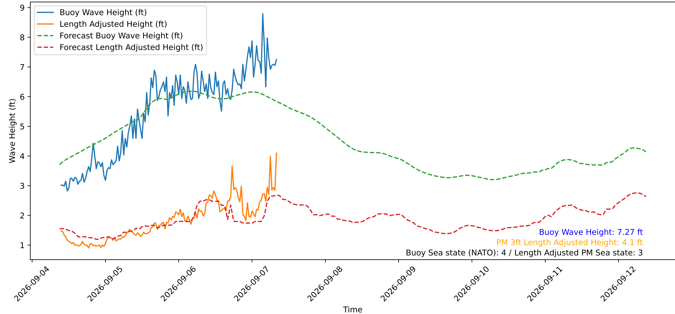
Wave Heights over Time for Green Beach at 2026-09-07 09:01:13
