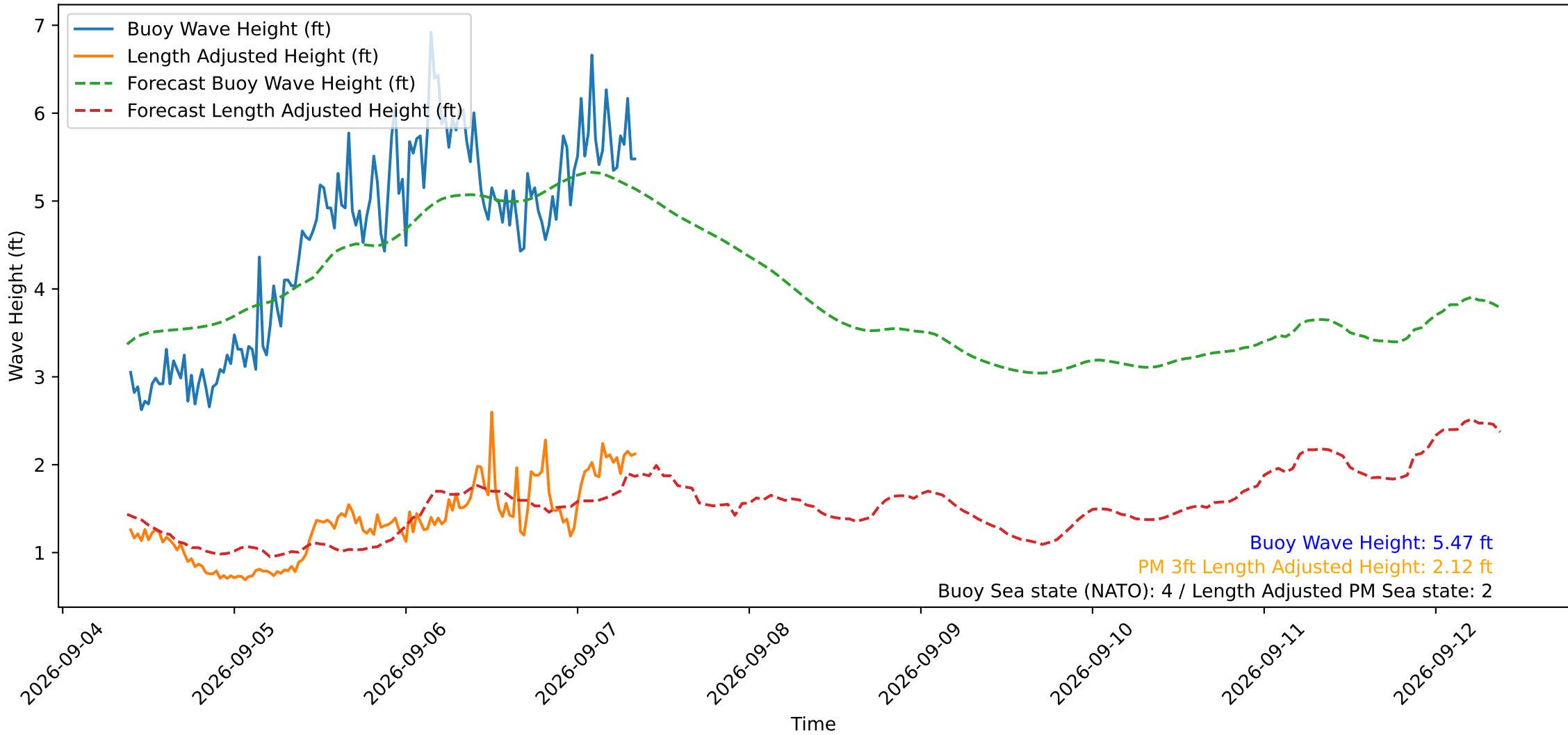
Wave Heights over Time for Red Beach at 2026-09-07 09:00:49
