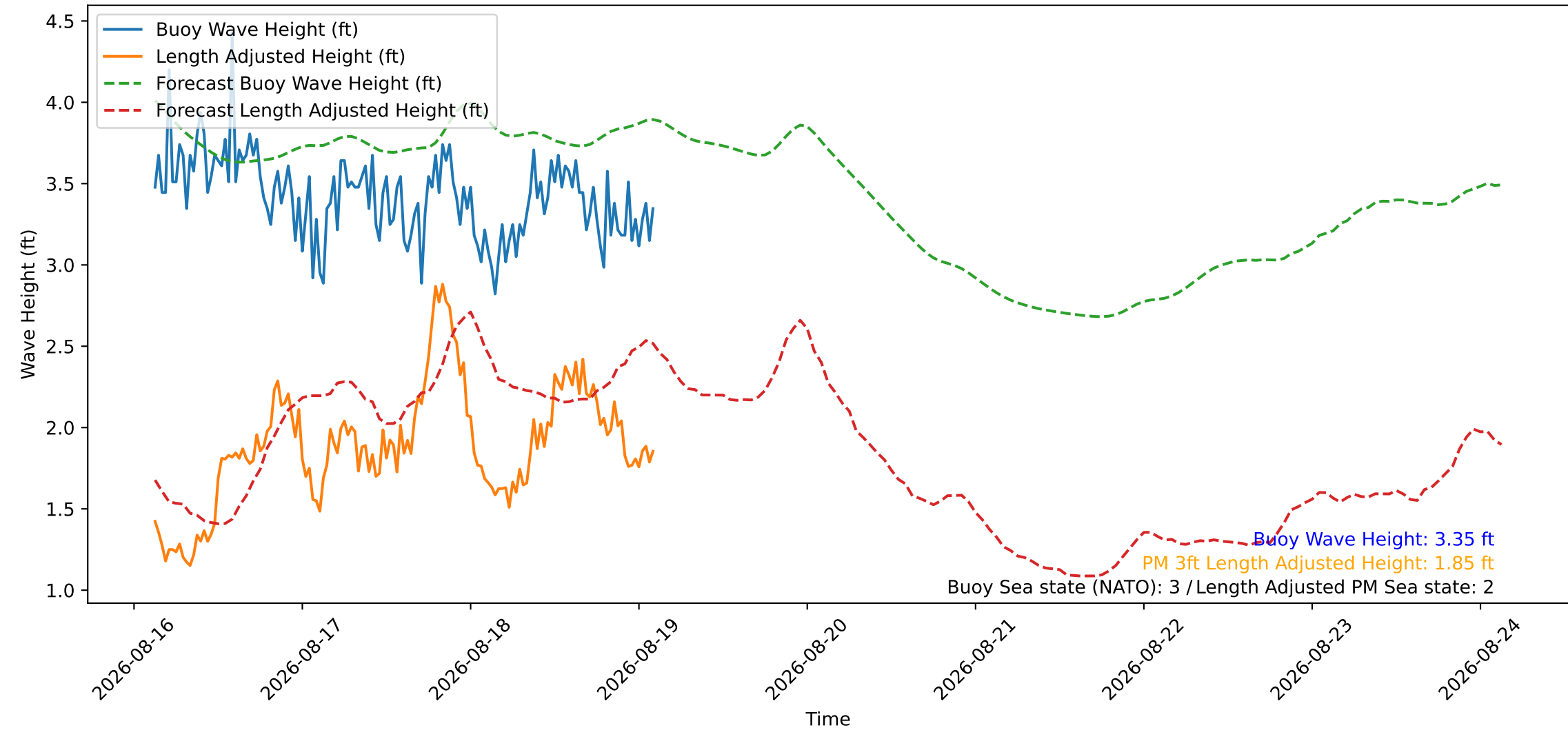
Wave Heights over Time for Oceanside Harbor at 2026-08-19 02:50:26
