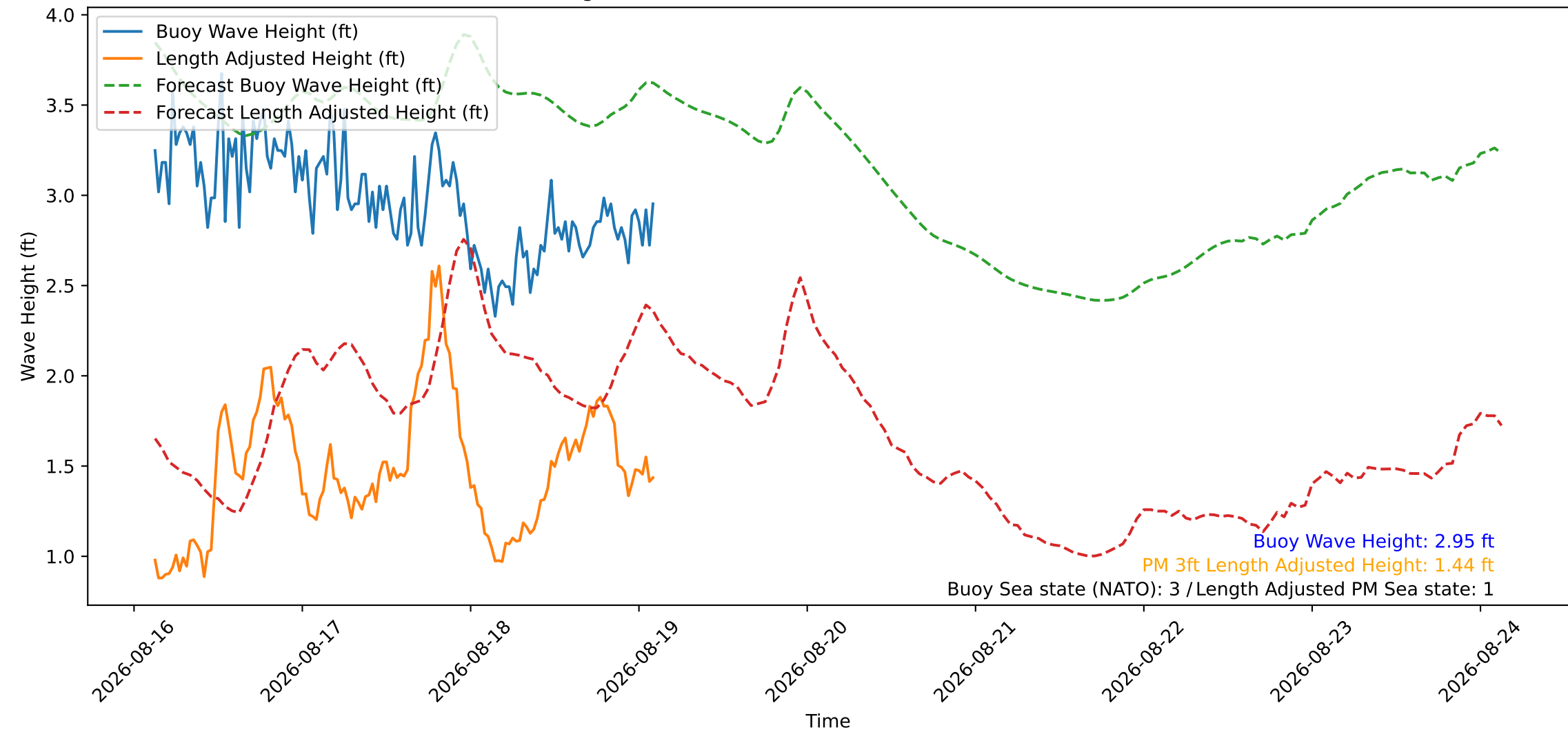
Wave Heights over Time for Red Beach at 2026-08-19 02:50:47
