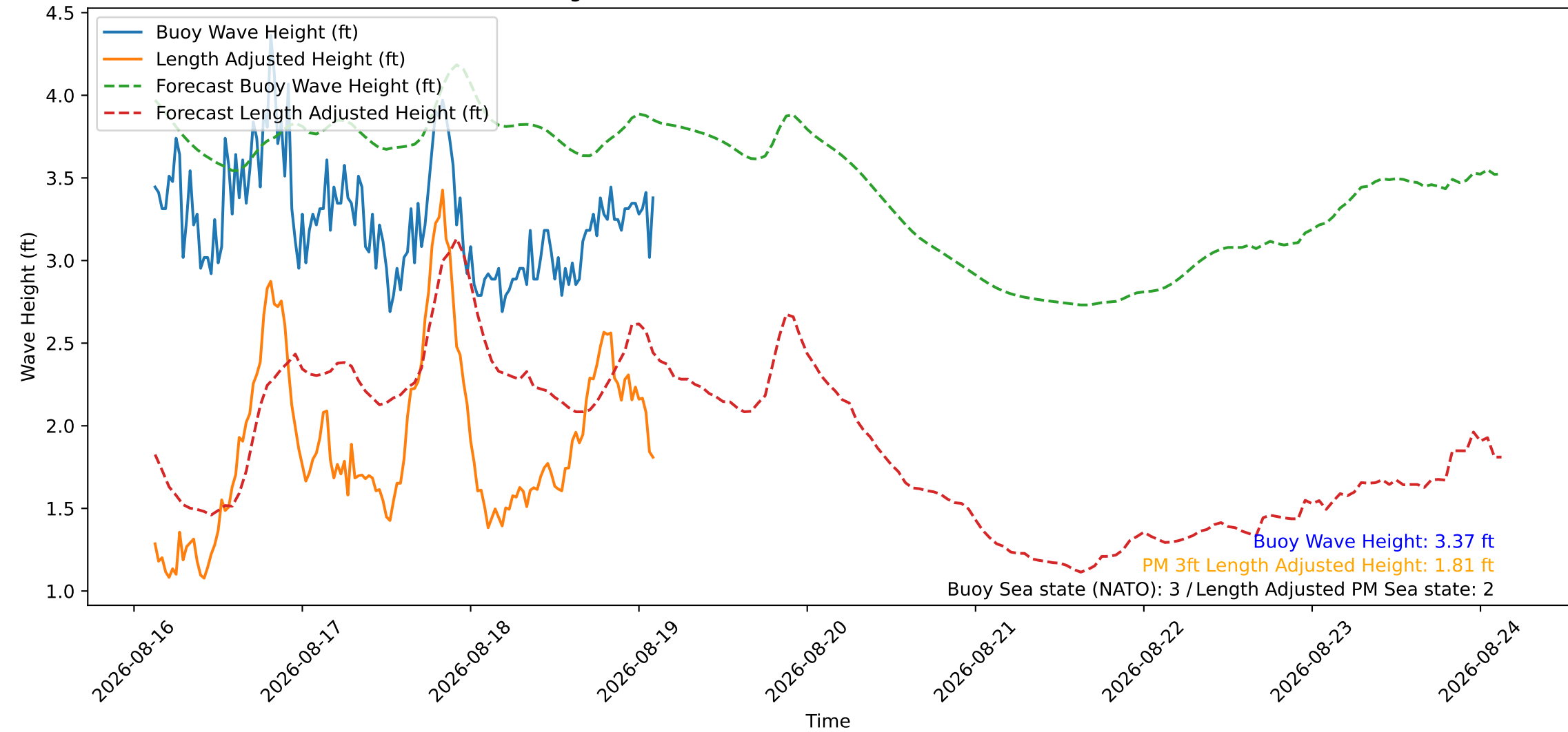
Wave Heights over Time for Green Beach at 2026-08-19 02:51:11
