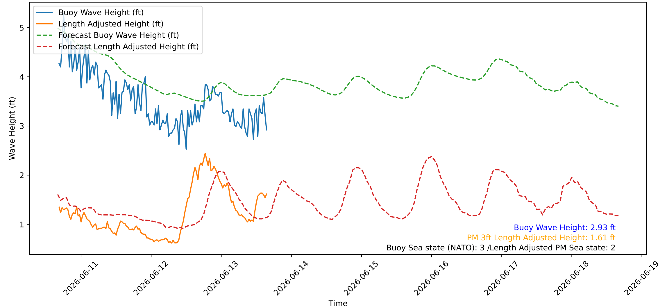
Wave Heights over Time for Red Beach at 2026-06-13 16:10:45
