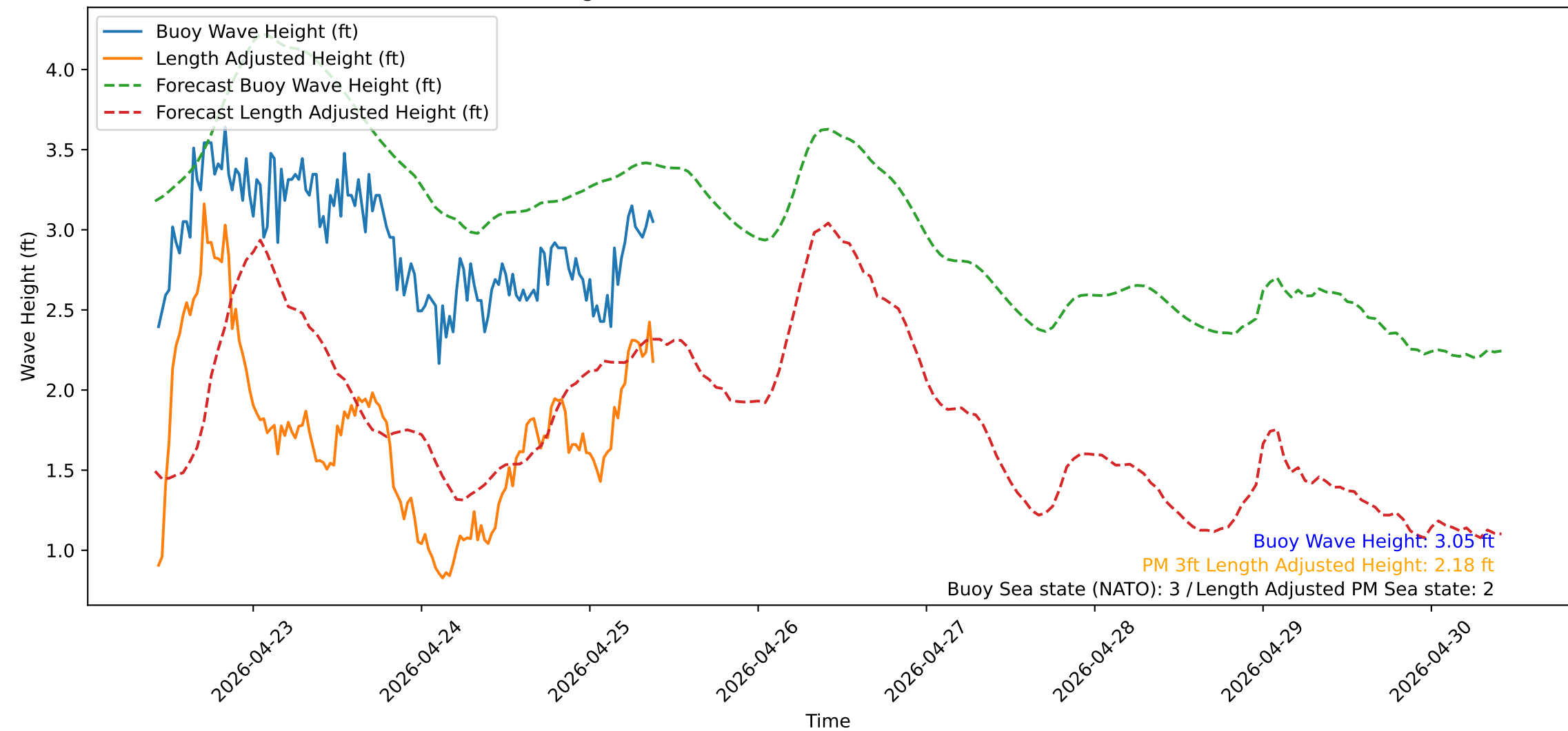
Wave Heights over Time for Red Beach at 2026-04-25 10:00:50
