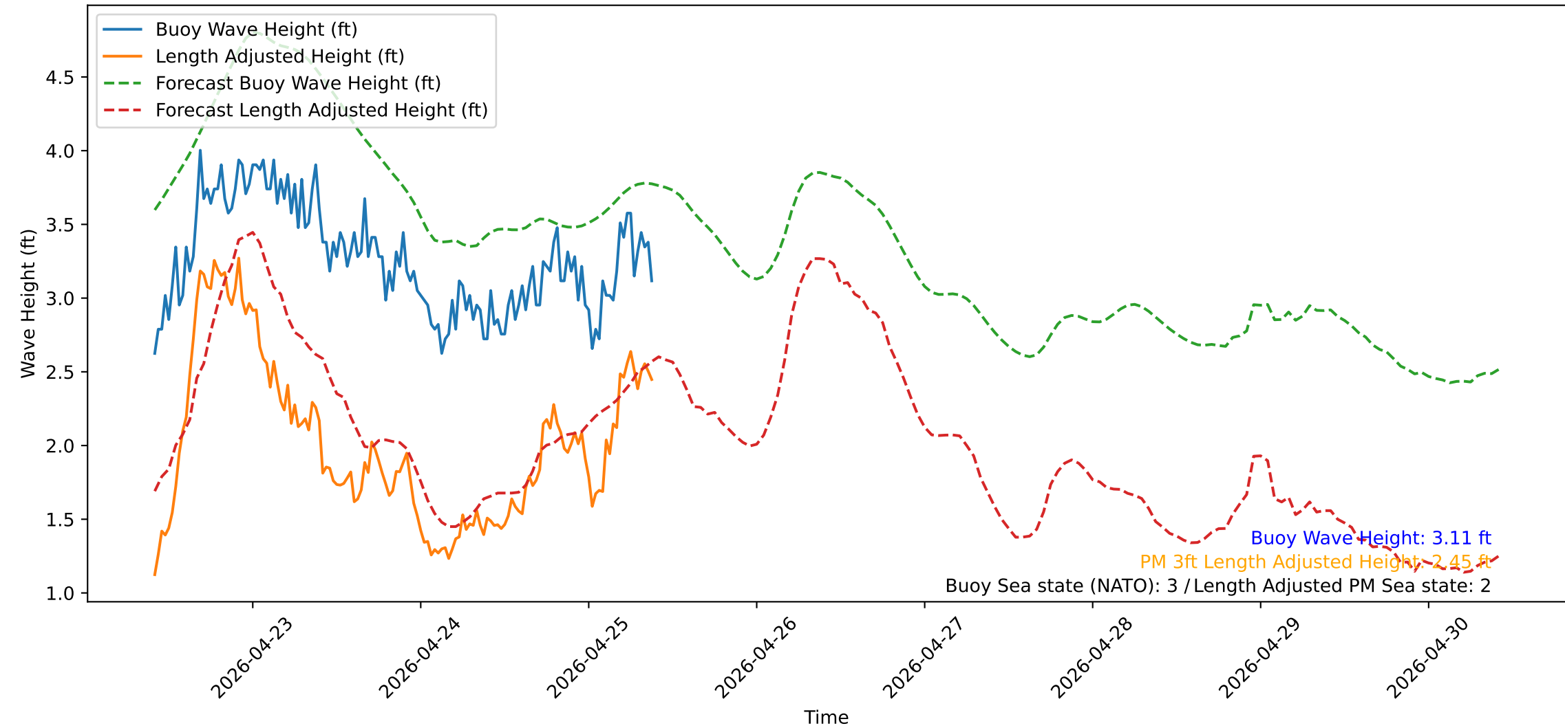
Wave Heights over Time for Green Beach at 2026-04-25 10:01:12
