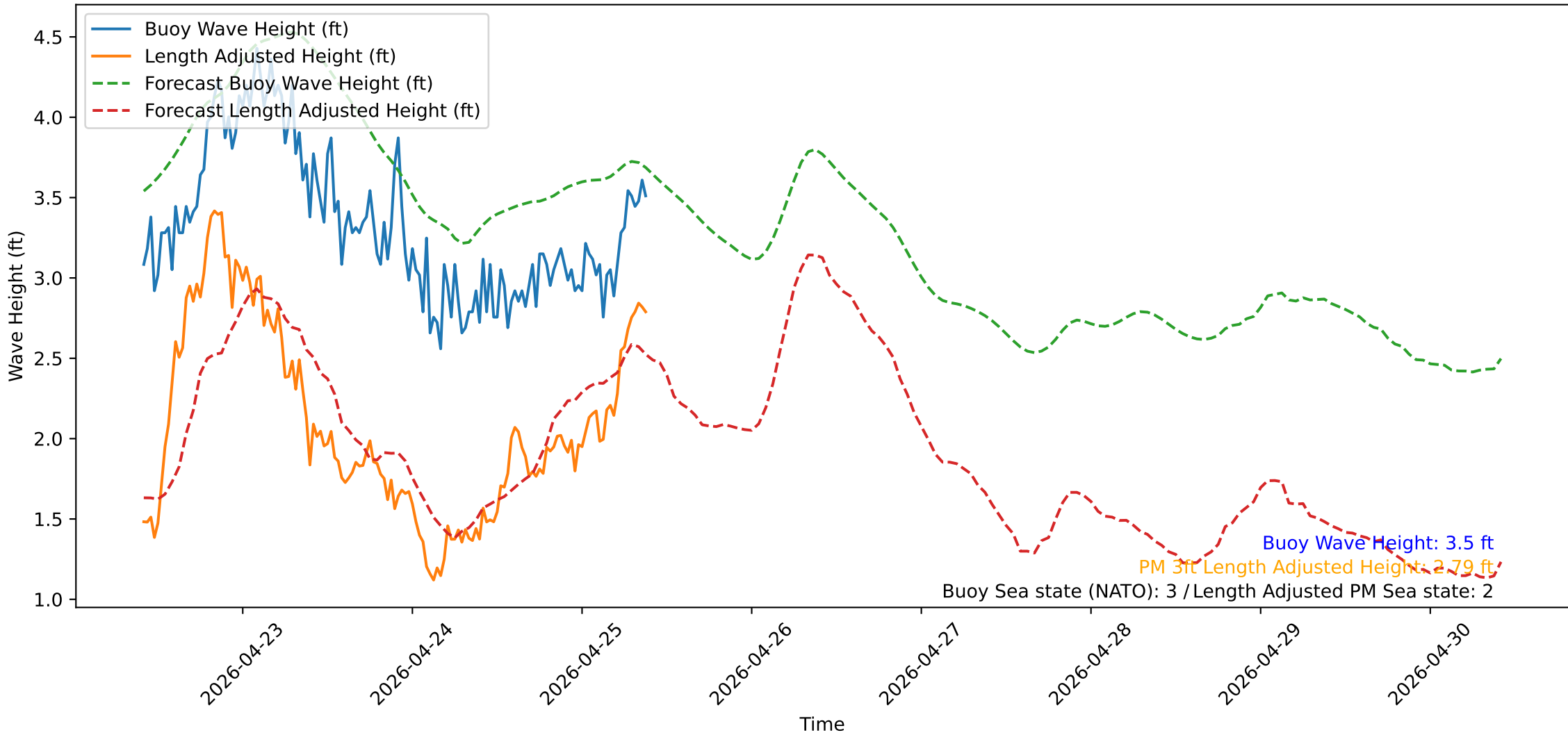
Wave Heights over Time for Oceanside Harbor at 2026-04-25 10:00:31
