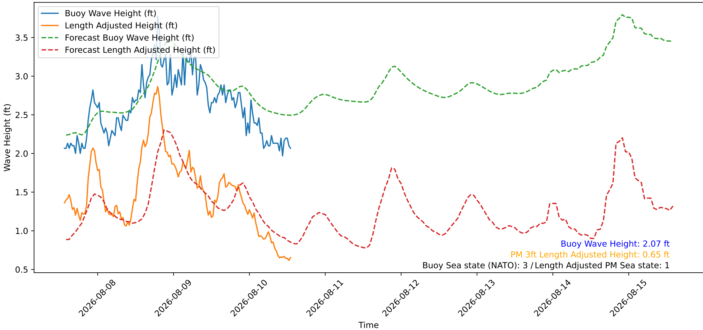
Wave Heights over Time for Green Beach at 2026-08-10 13:41:08
