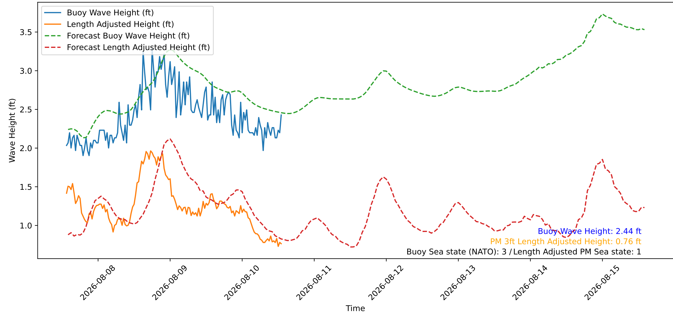
Wave Heights over Time for Oceanside Harbor at 2026-08-10 13:40:26
