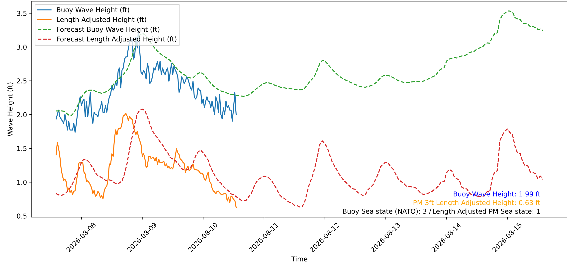
Wave Heights over Time for Red Beach at 2026-08-10 13:40:45
