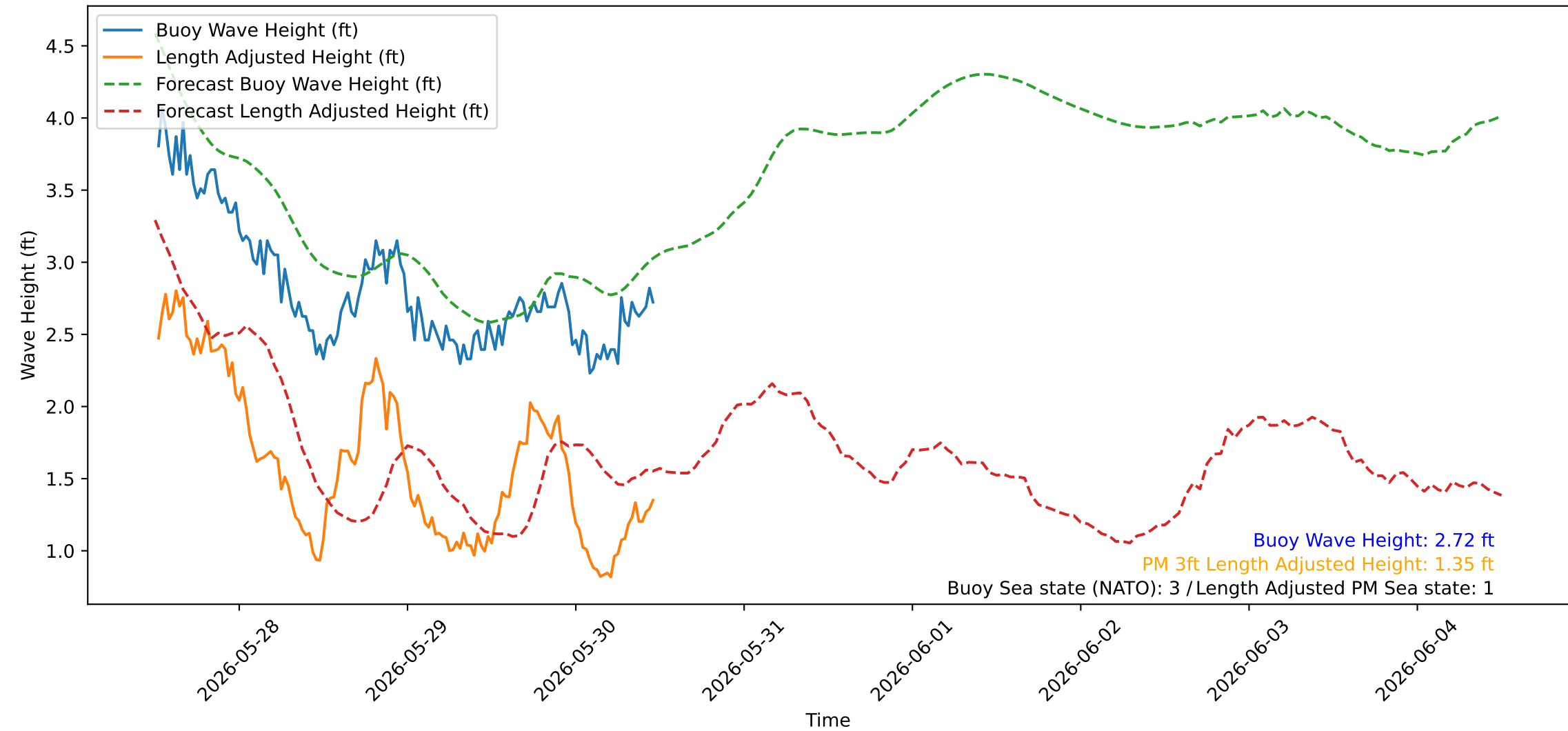
Wave Heights over Time for Red Beach at 2026-05-30 12:00:42
