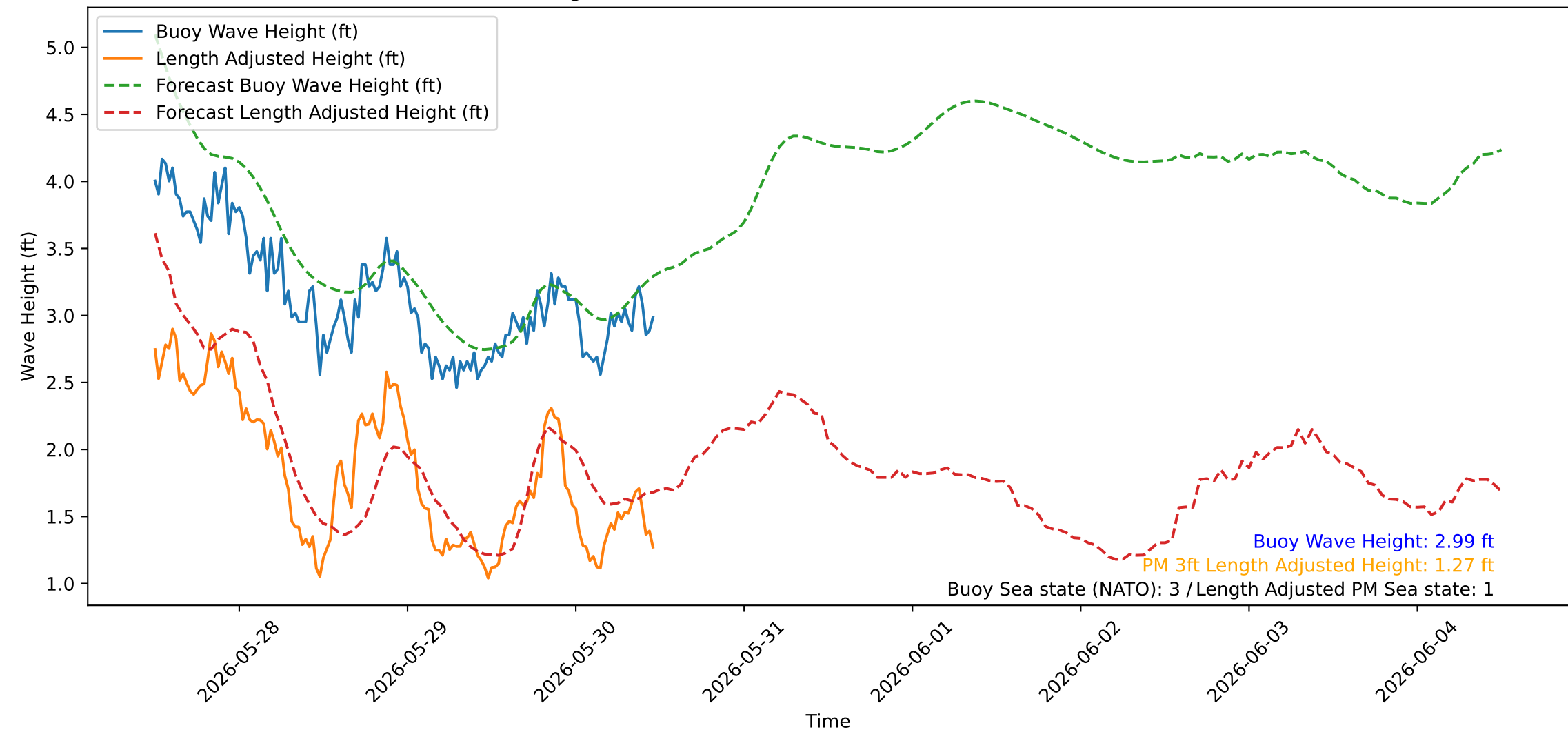
Wave Heights over Time for Green Beach at 2026-05-30 12:01:05
