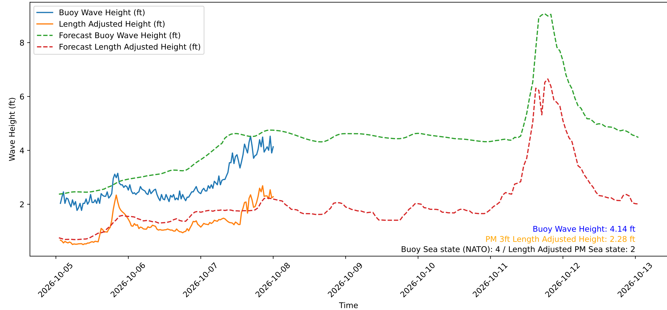
Wave Heights over Time for Green Beach at 2026-10-08 01:01:11
