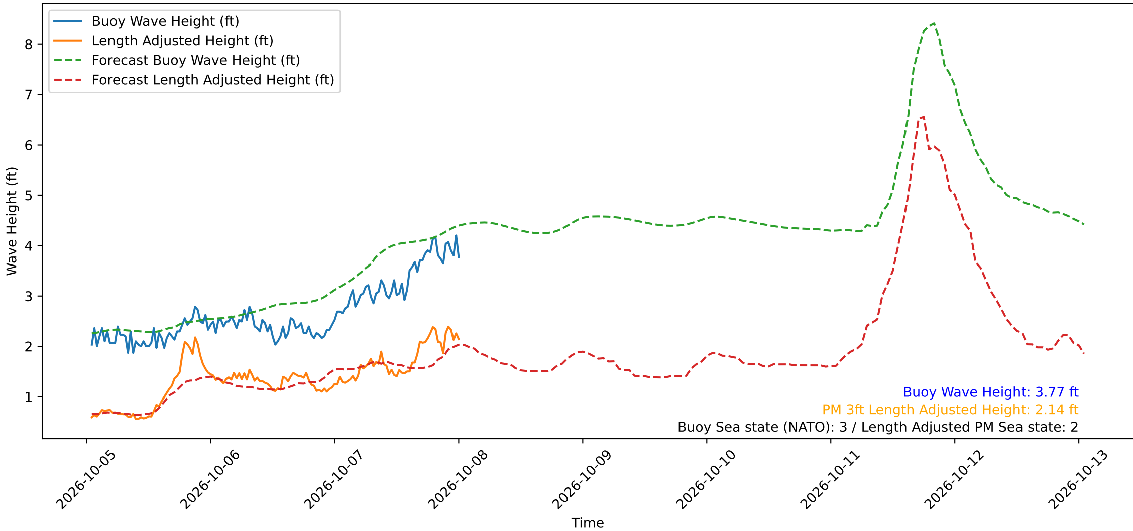
Wave Heights over Time for Oceanside Harbor at 2026-10-08 01:00:30
