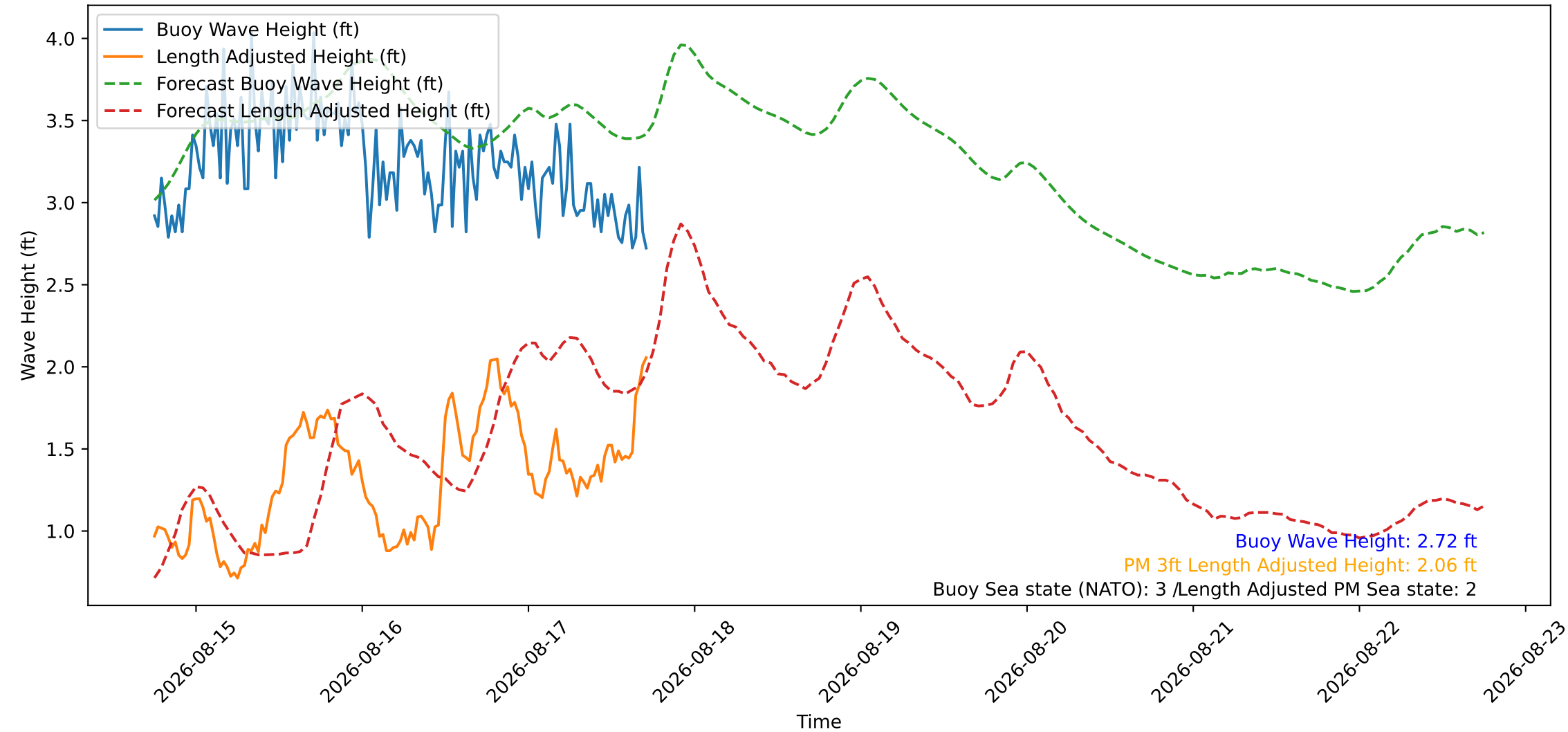
Wave Heights over Time for Red Beach at 2026-08-17 17:50:48
