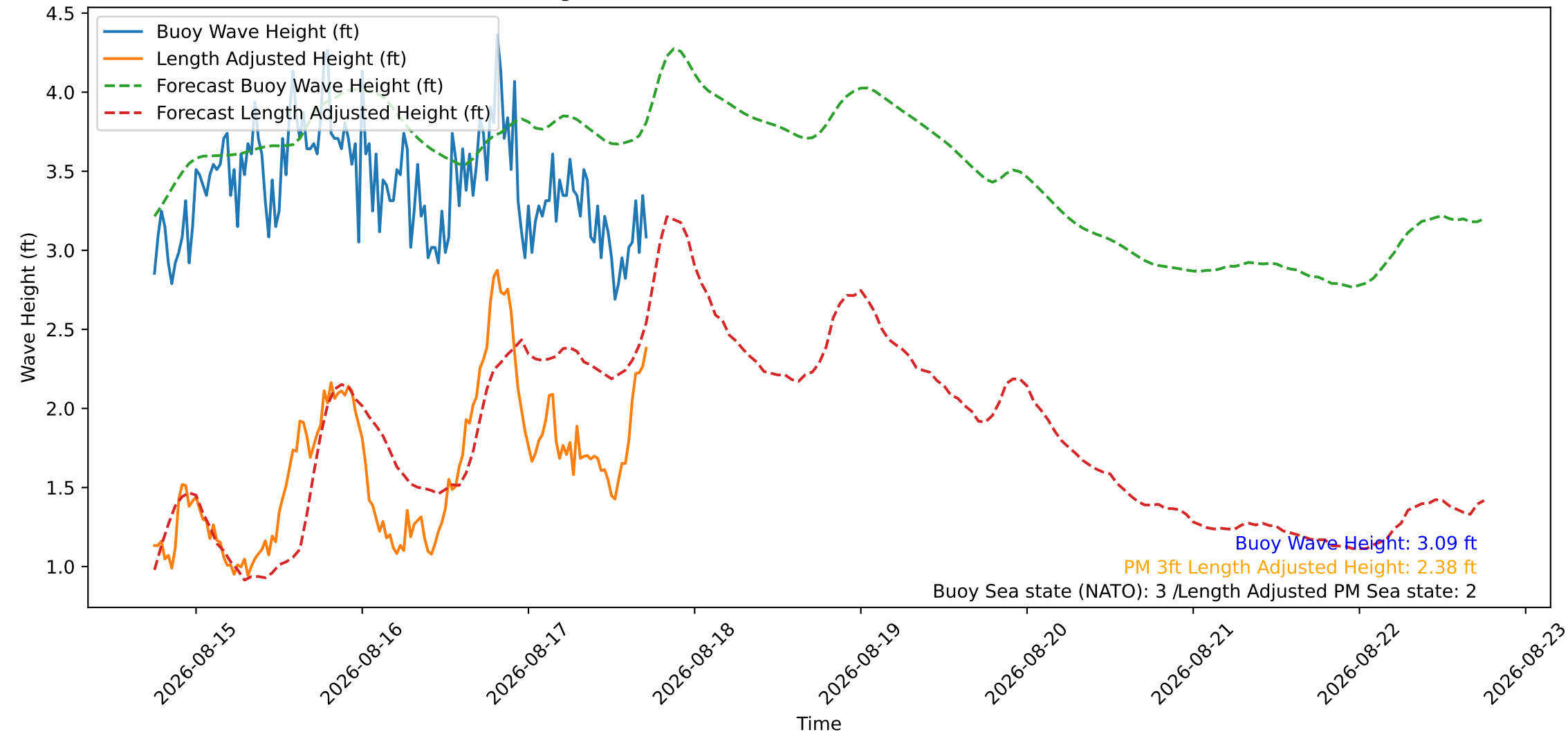
Wave Heights over Time for Green Beach at 2026-08-17 17:51:12
