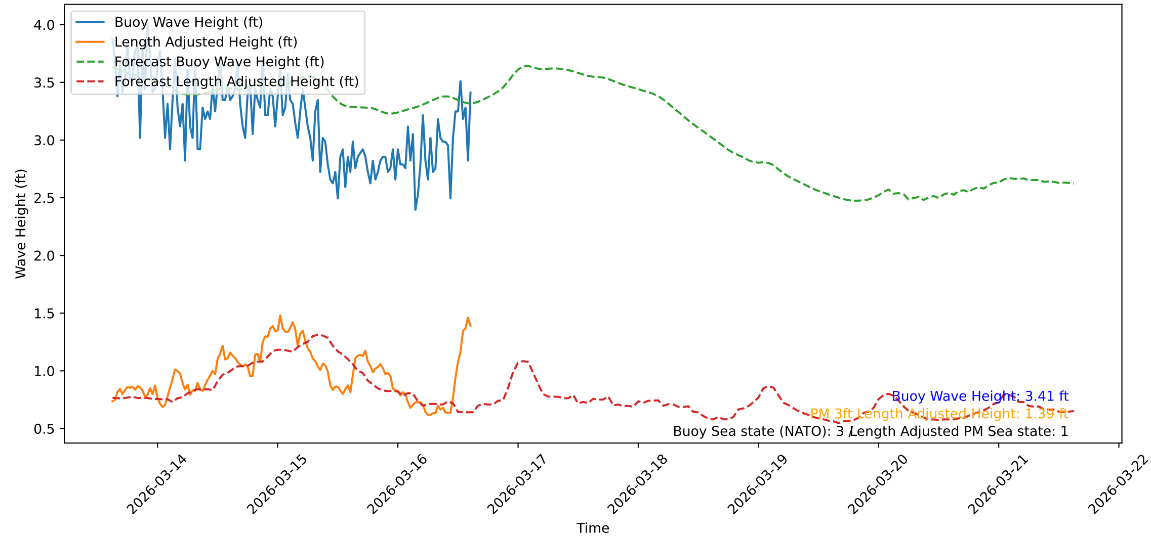
Wave Heights over Time for Oceanside Harbor at 2026-03-16 15:10:59
