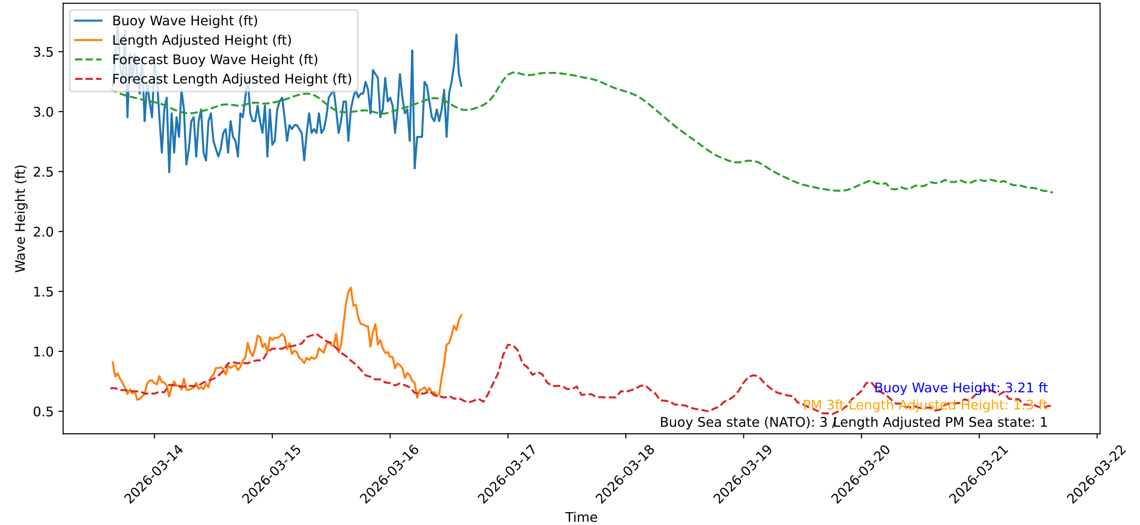
Wave Heights over Time for Red Beach at 2026-03-16 15:11:21
