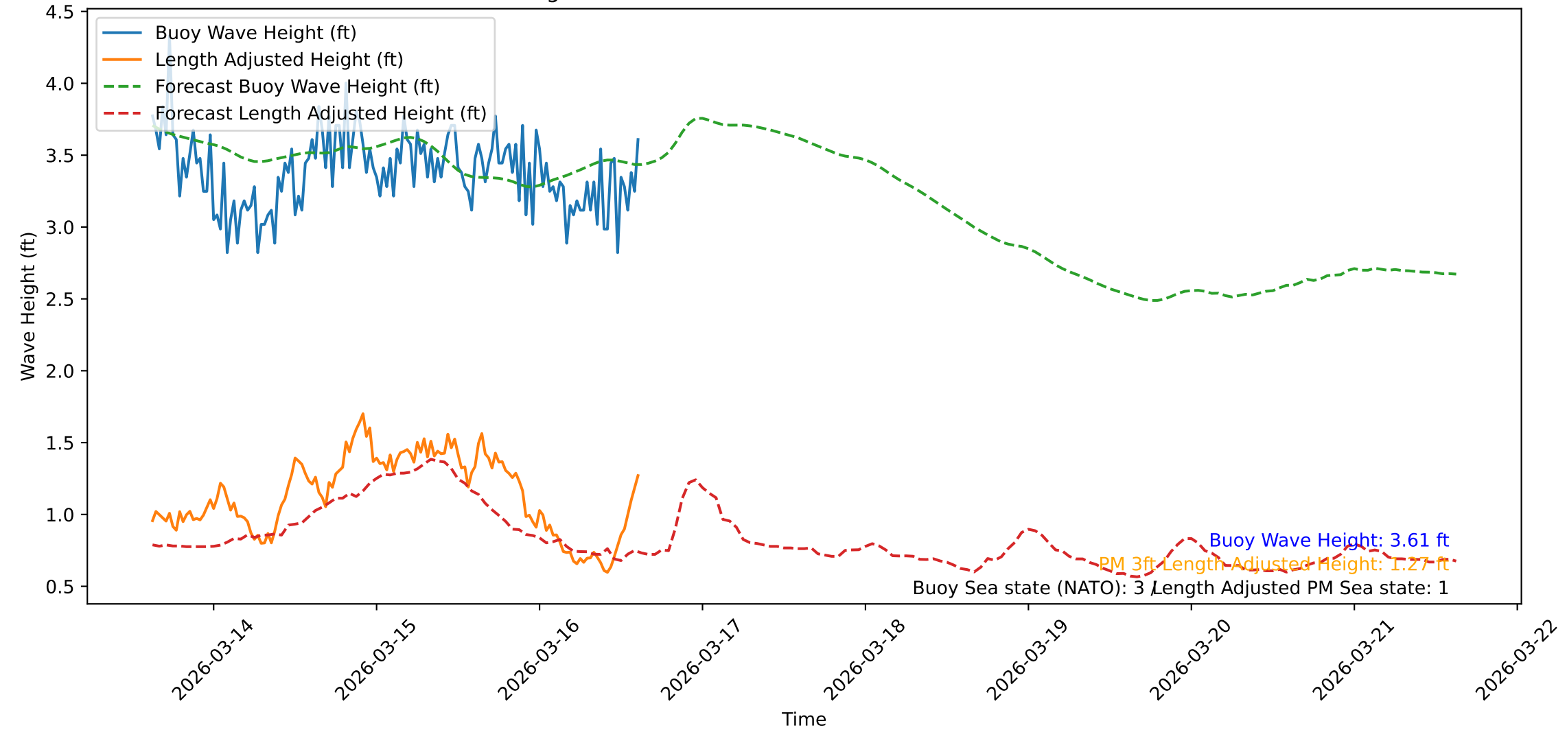
Wave Heights over Time for Green Beach at 2026-03-16 15:11:55
