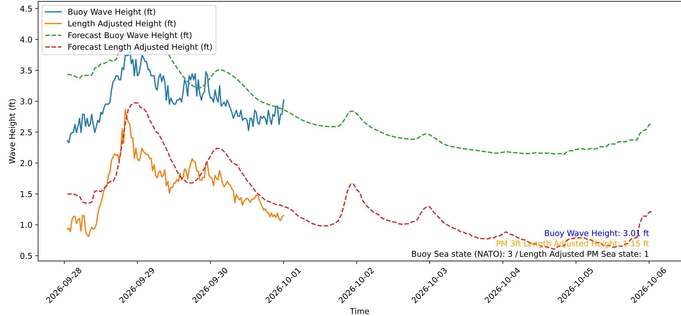
Wave Heights over Time for Red Beach at 2026-10-01 00:50:50
