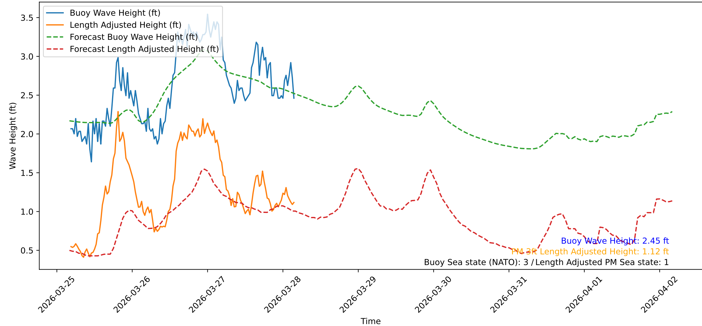
Wave Heights over Time for Green Beach at 2026-03-28 04:21:10
