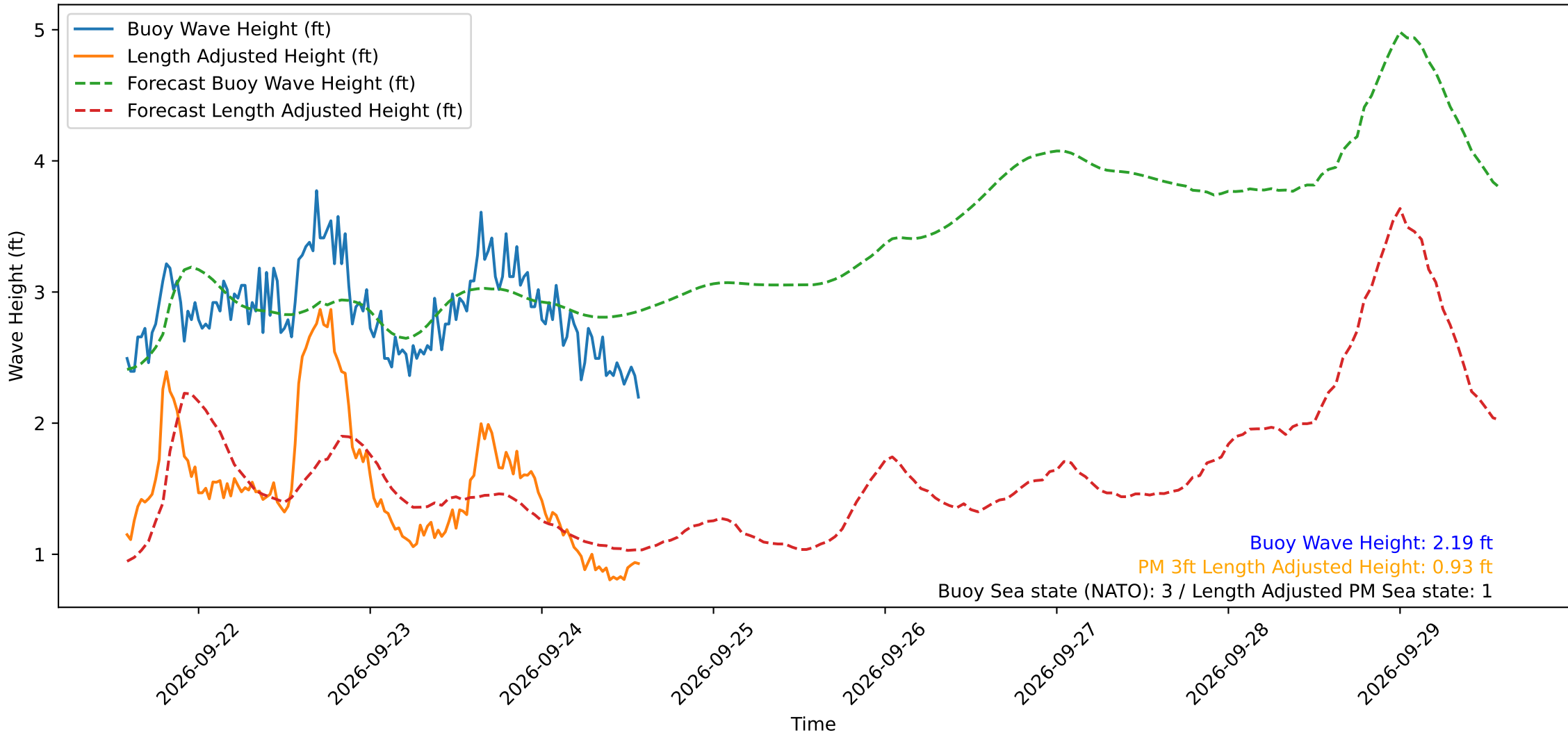
Wave Heights over Time for Oceanside Harbor at 2026-09-24 14:10:30
