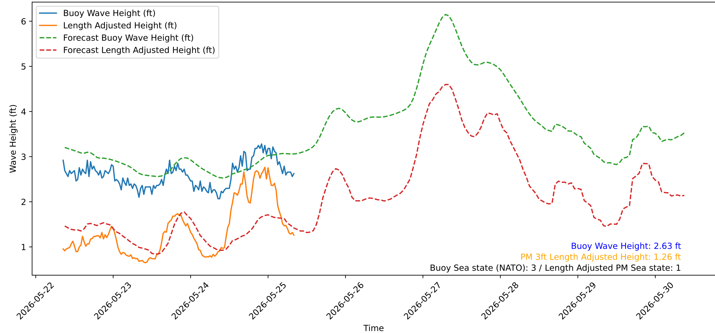
Wave Heights over Time for Green Beach at 2026-05-25 08:41:12
