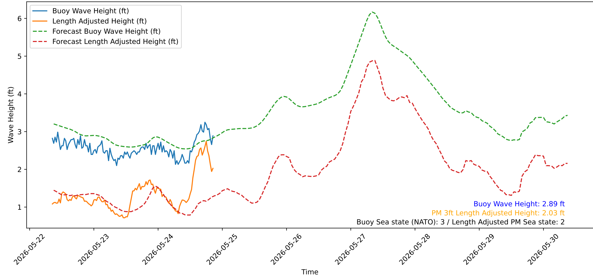
Wave Heights over Time for Oceanside Harbor at 2026-05-25 08:40:31
