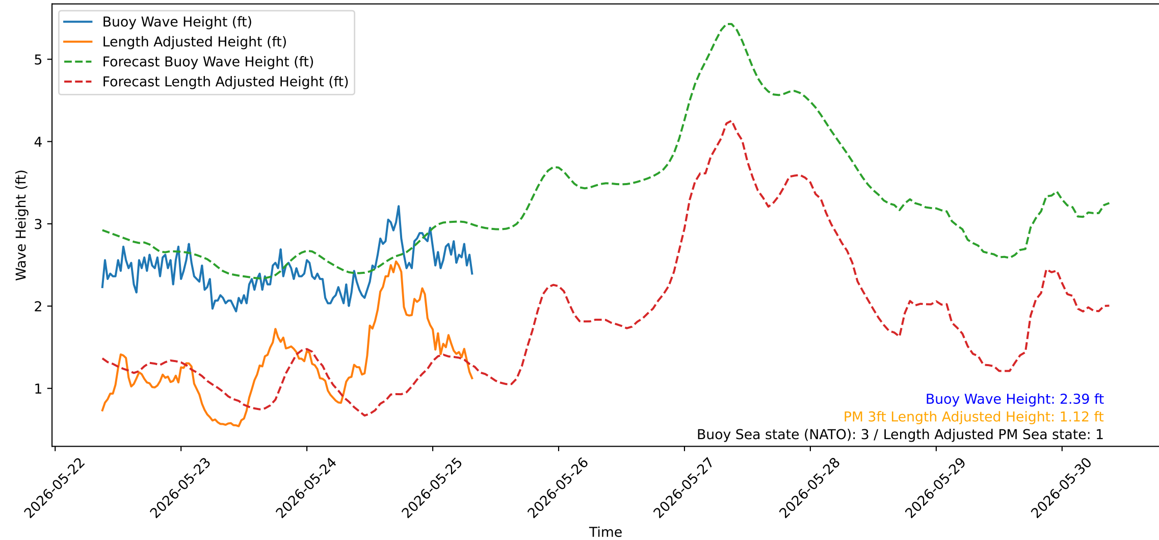
Wave Heights over Time for Red Beach at 2026-05-25 08:40:50
