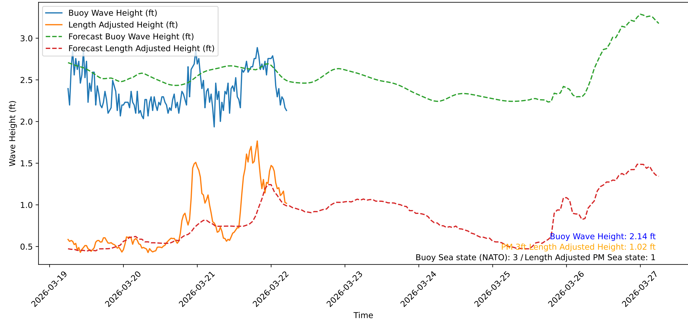
Wave Heights over Time for Green Beach at 2026-03-22 06:01:09
