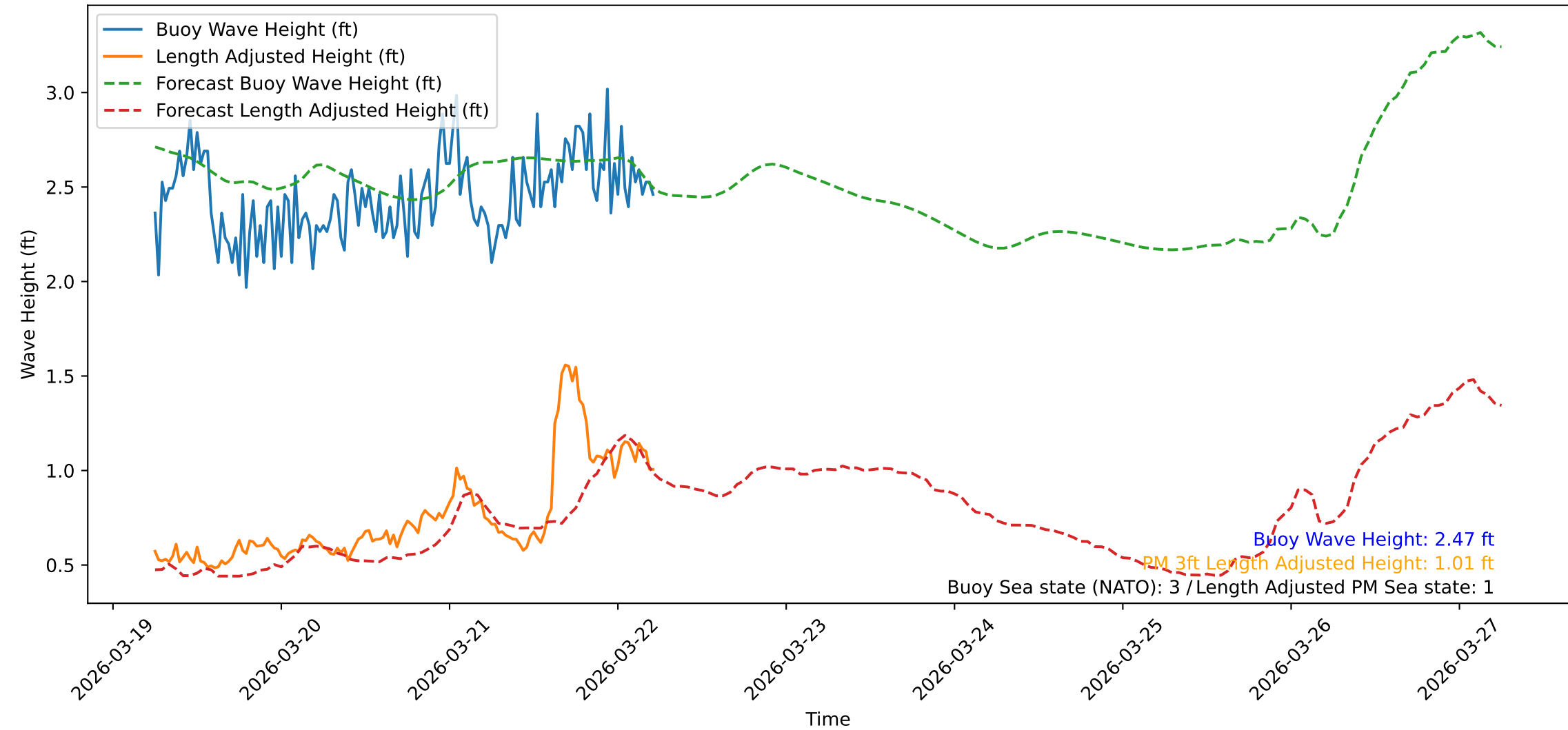
Wave Heights over Time for Oceanside Harbor at 2026-03-22 06:00:31
