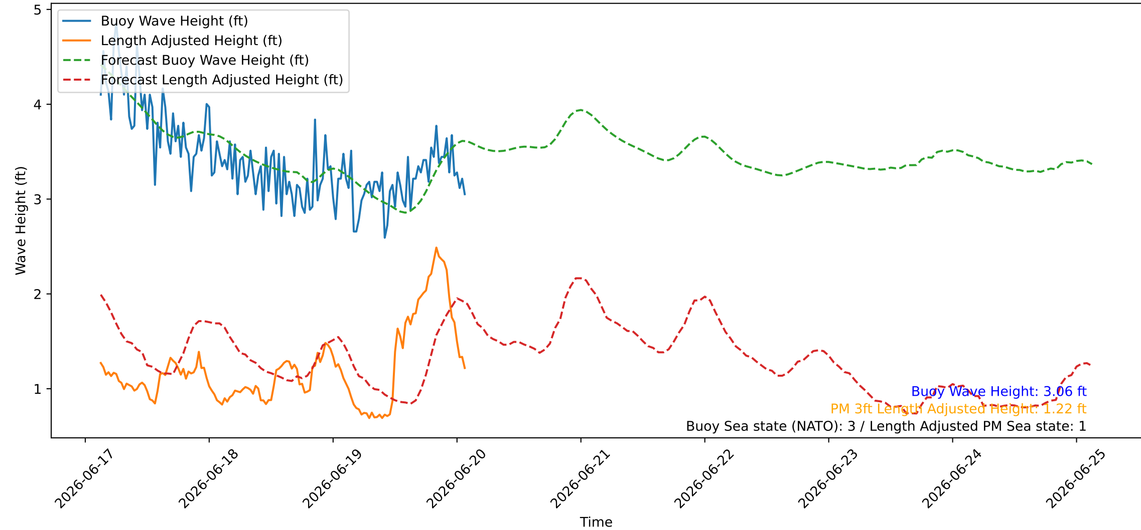
Wave Heights over Time for Red Beach at 2026-06-20 02:30:44
