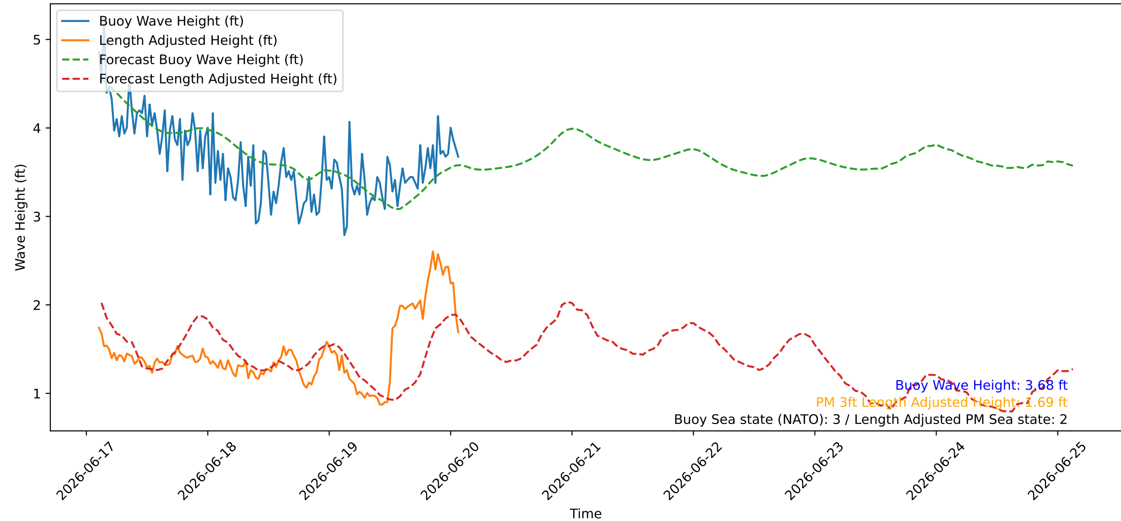
Wave Heights over Time for Oceanside Harbor at 2026-06-20 02:30:26
