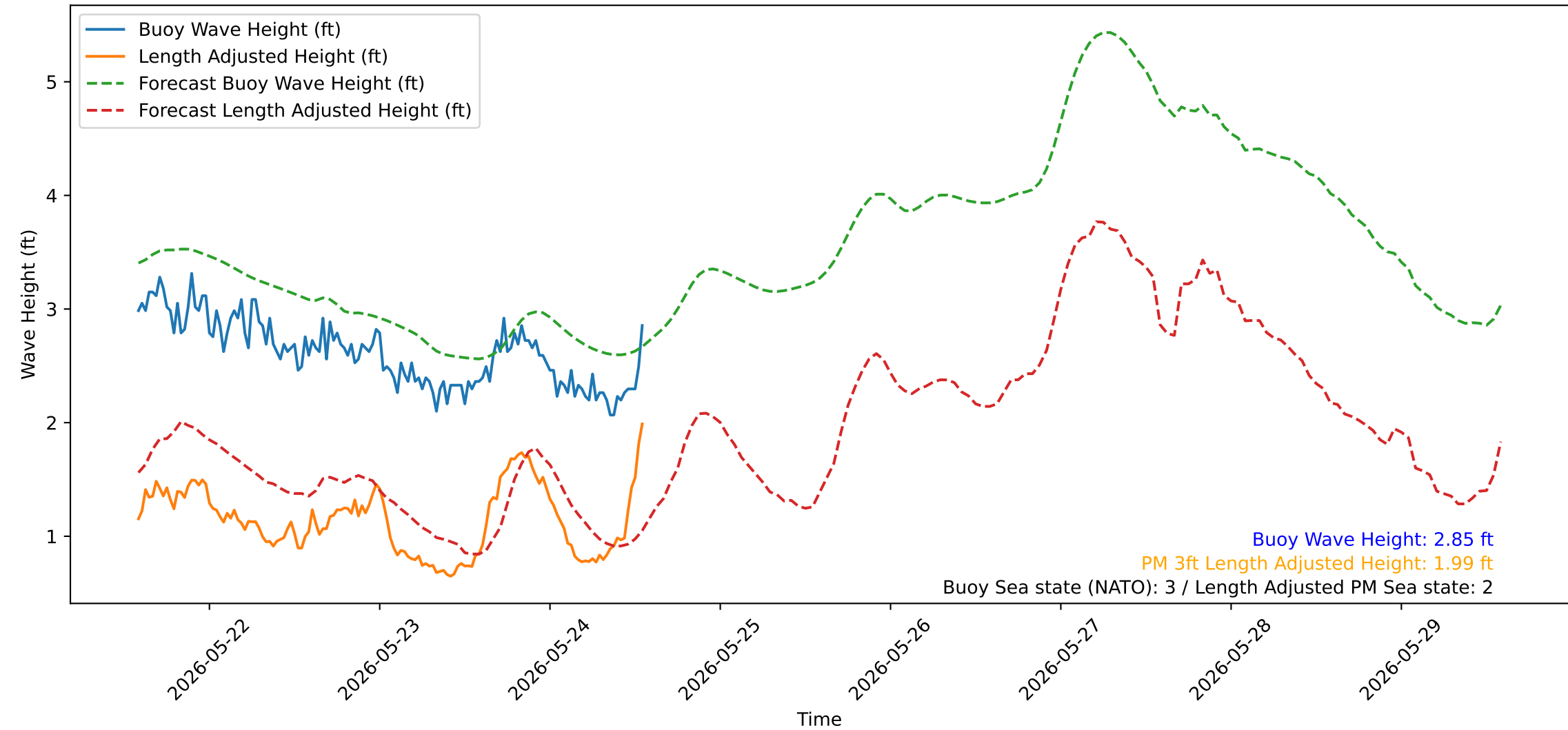
Wave Heights over Time for Green Beach at 2026-05-24 13:51:16
