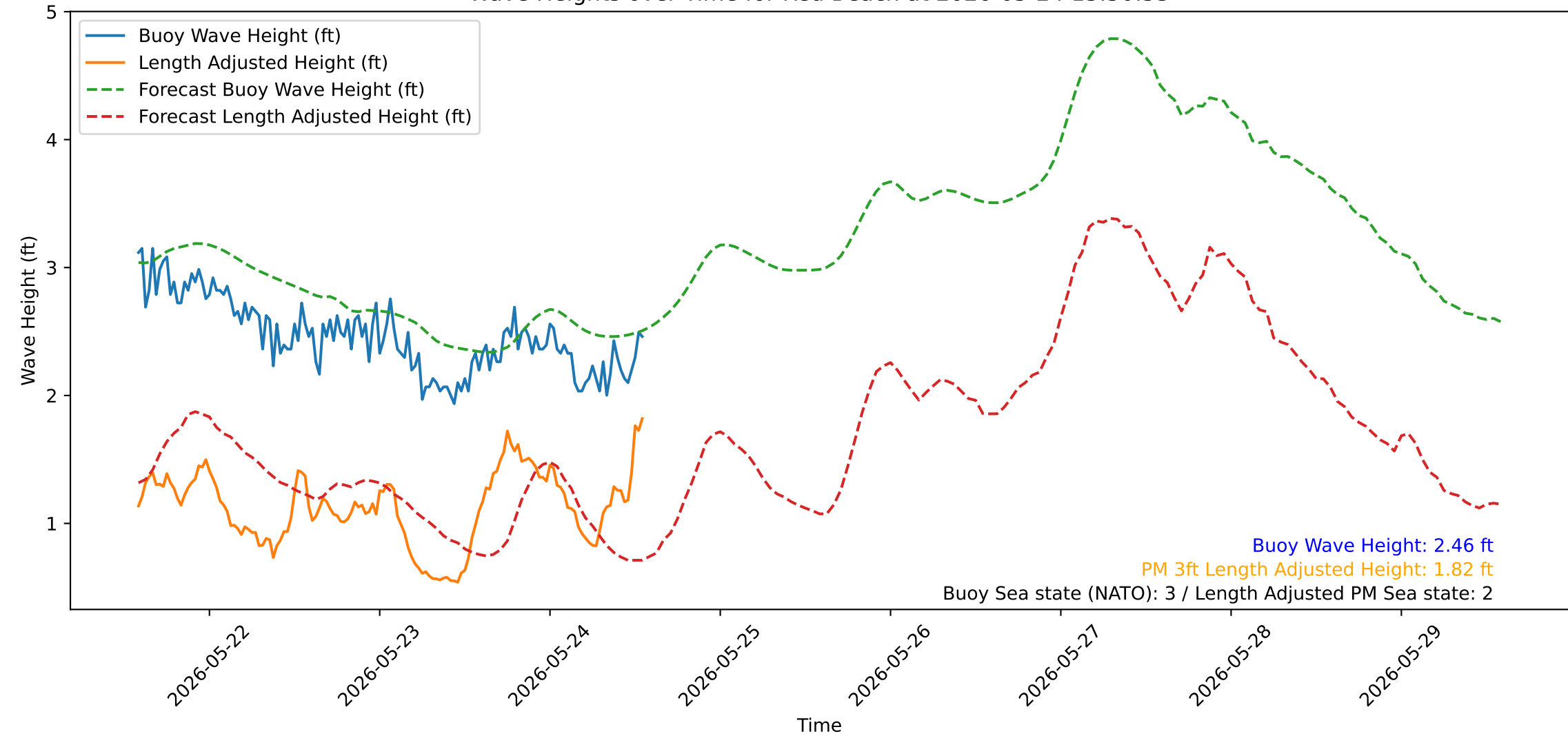
Wave Heights over Time for Red Beach at 2026-05-24 13:50:53
