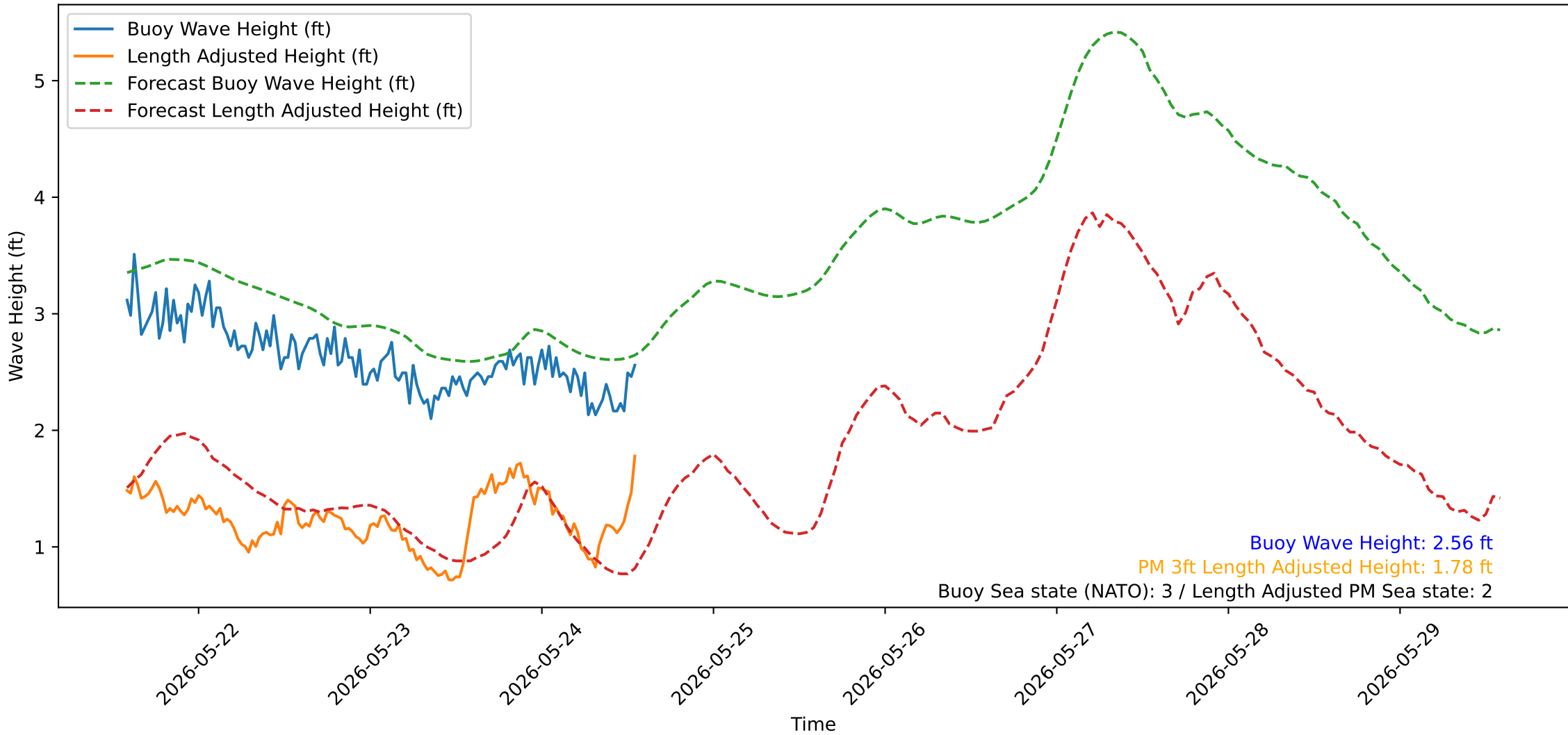
Wave Heights over Time for Oceanside Harbor at 2026-05-24 13:50:32
