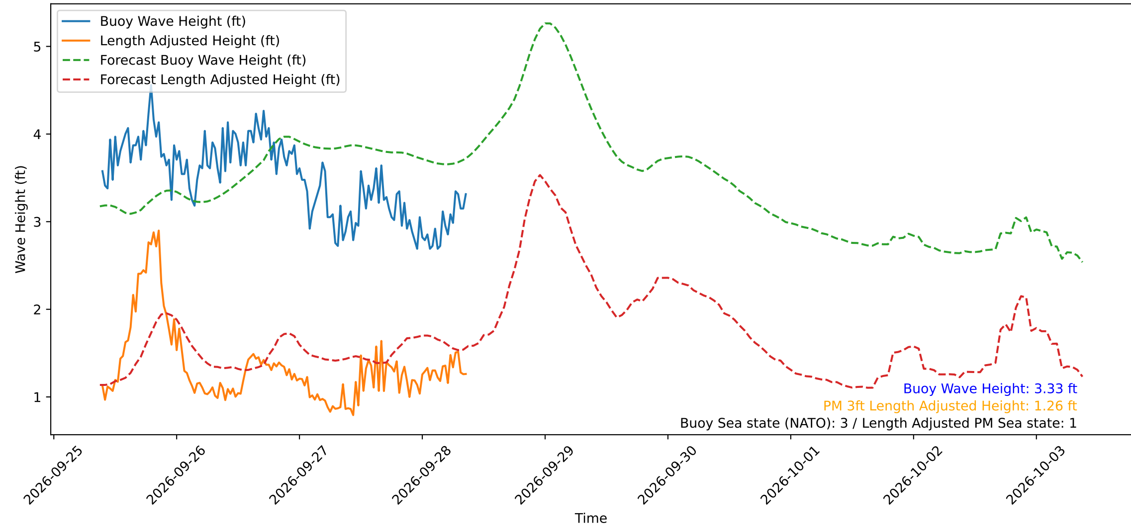
Wave Heights over Time for Green Beach at 2026-09-28 09:11:12
