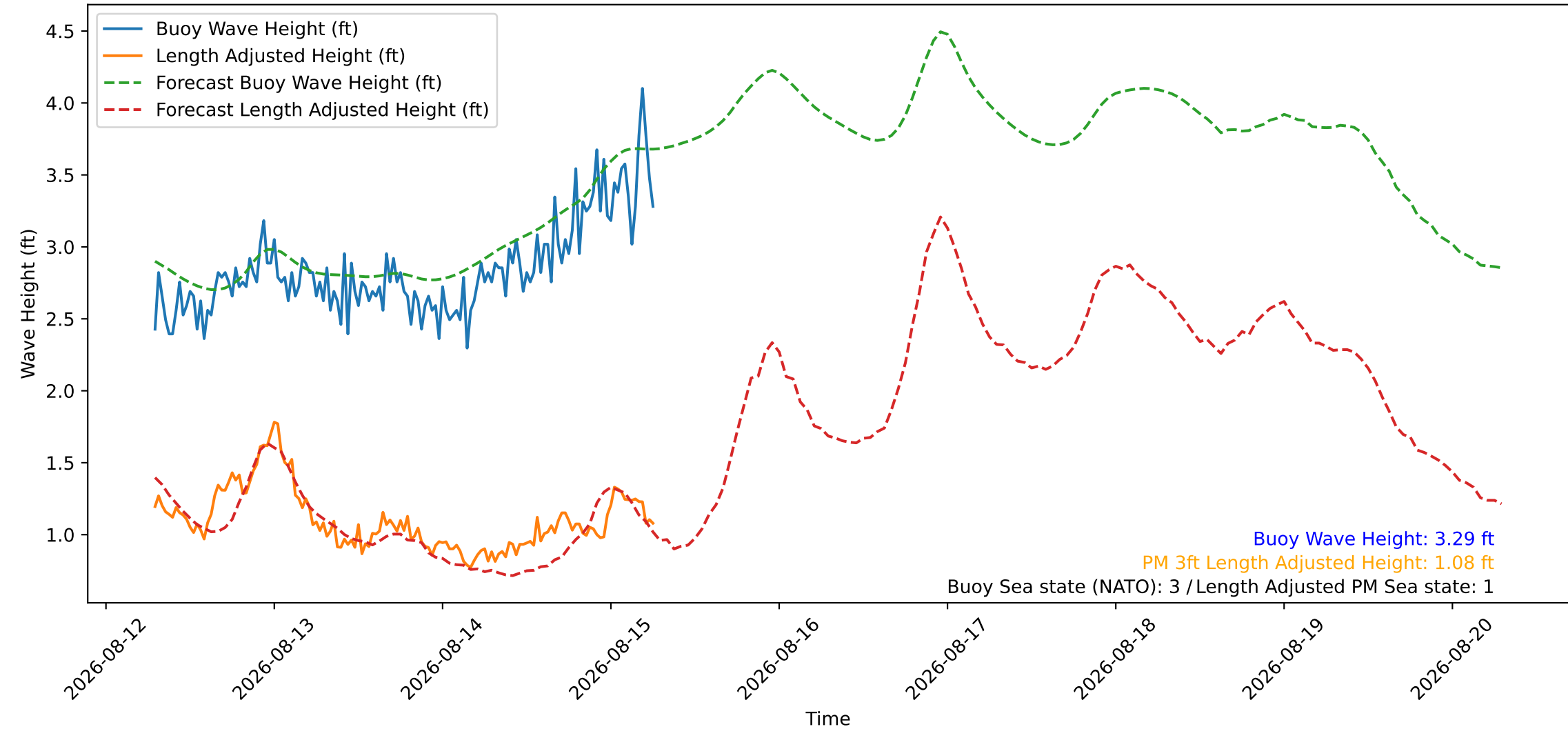
Wave Heights over Time for Oceanside Harbor at 2026-08-15 07:10:26
