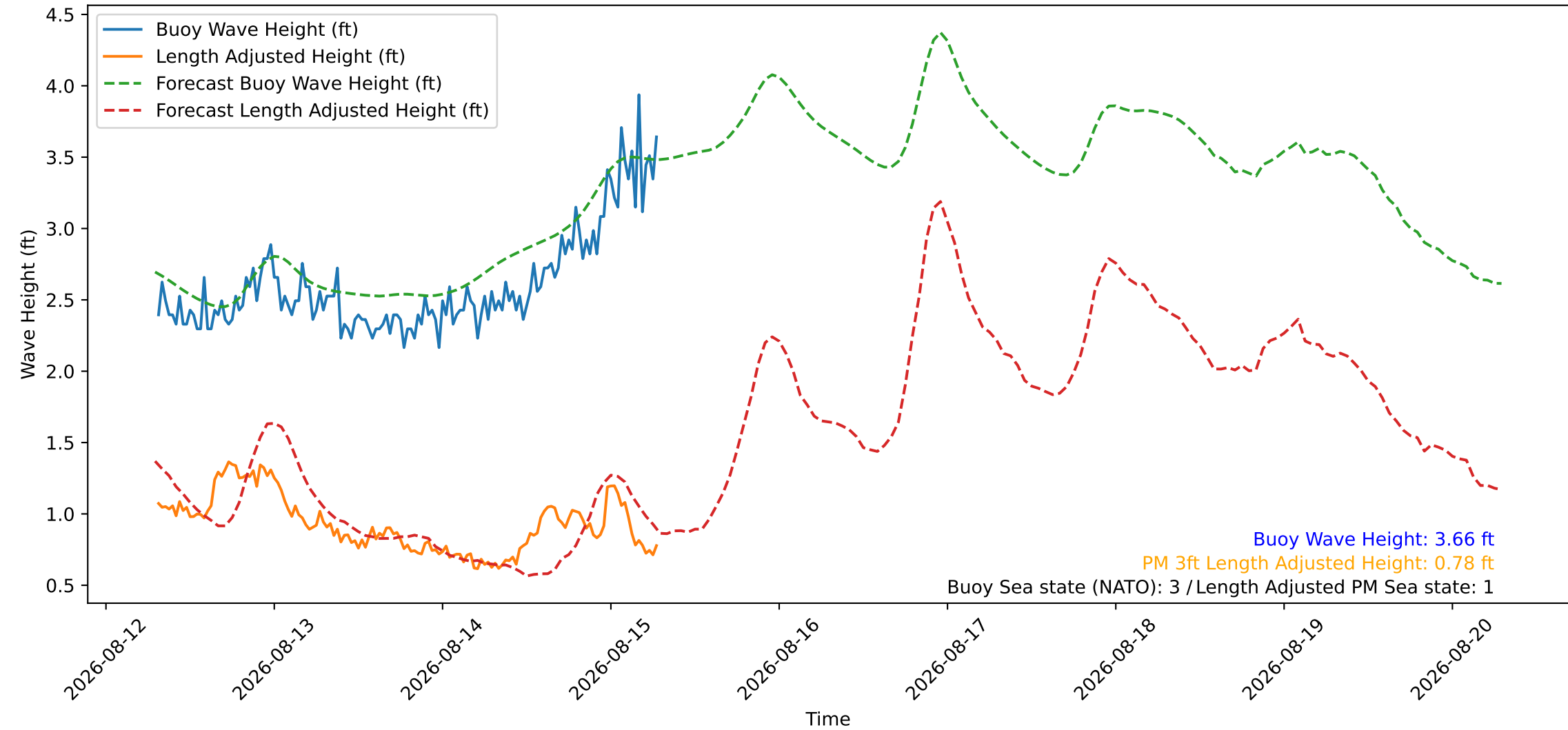
Wave Heights over Time for Red Beach at 2026-08-15 07:10:45
