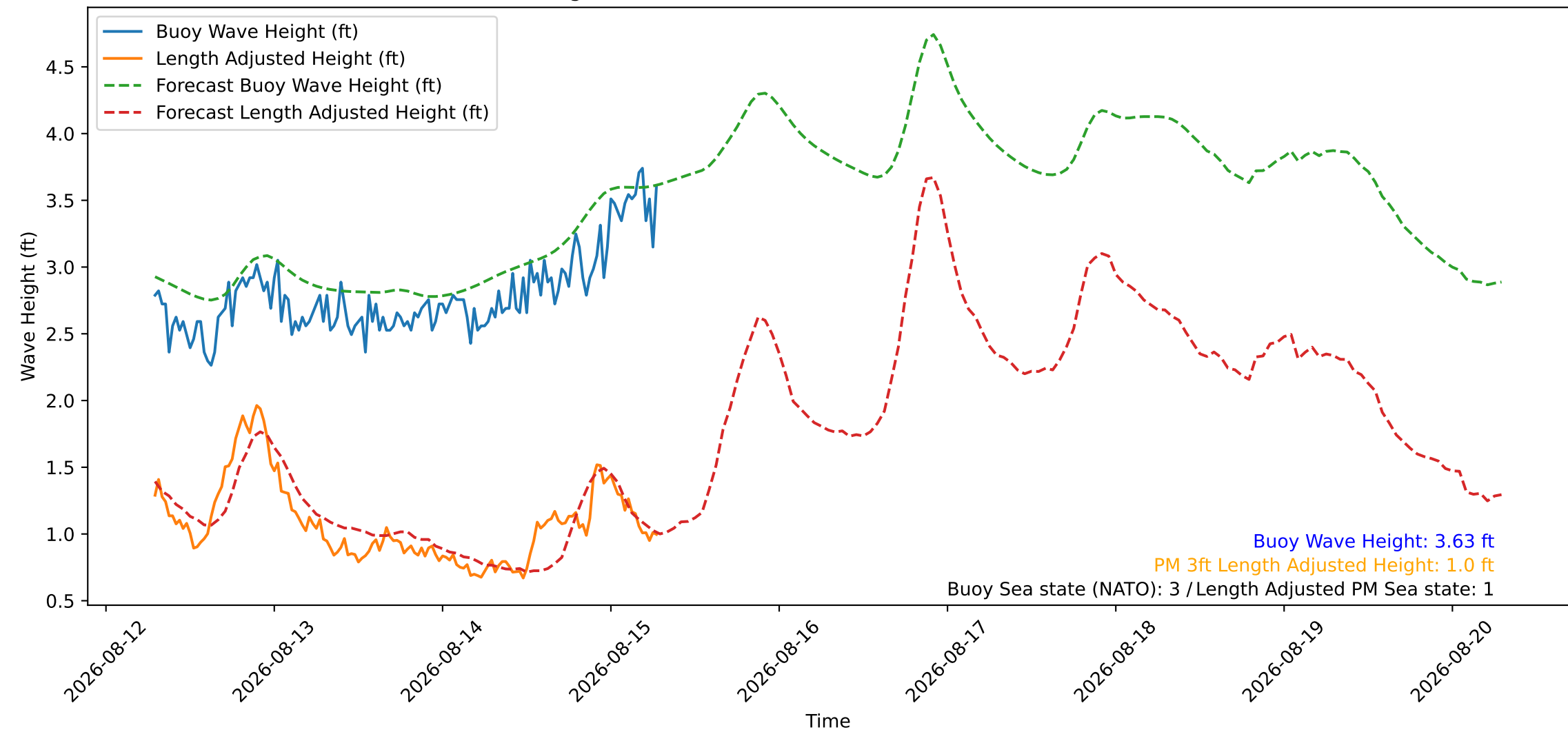
Wave Heights over Time for Green Beach at 2026-08-15 07:11:07
