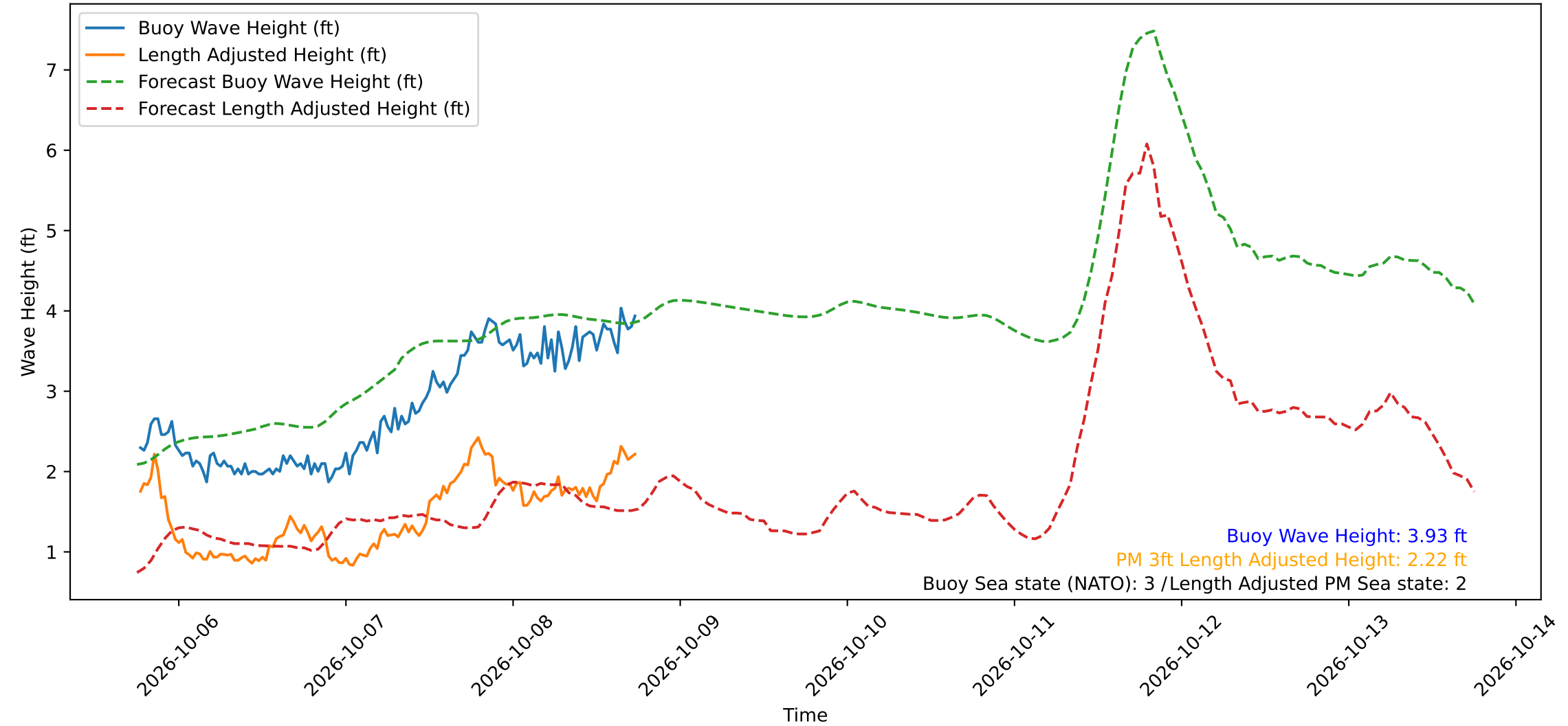
Wave Heights over Time for Red Beach at 2026-10-08 18:20:51
