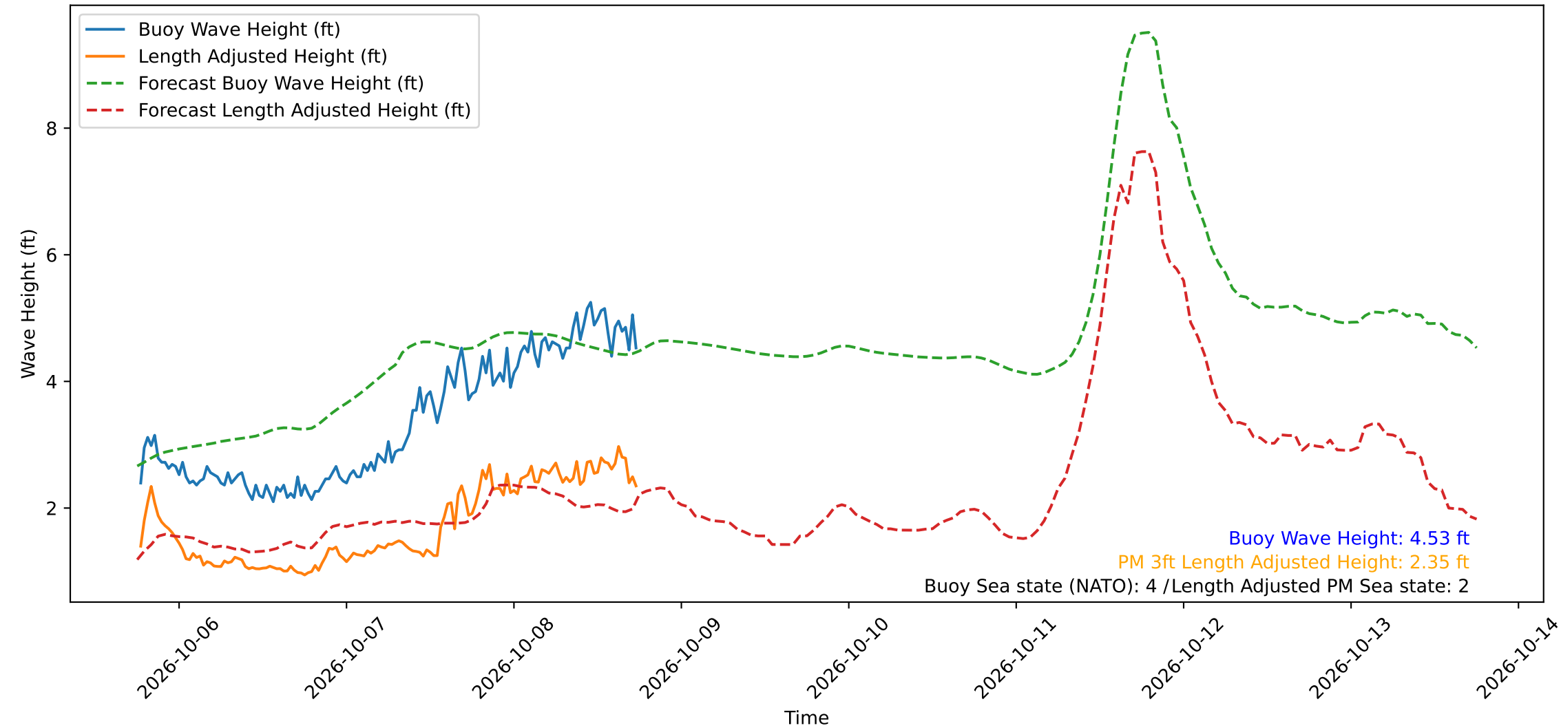
Wave Heights over Time for Green Beach at 2026-10-08 18:21:14
