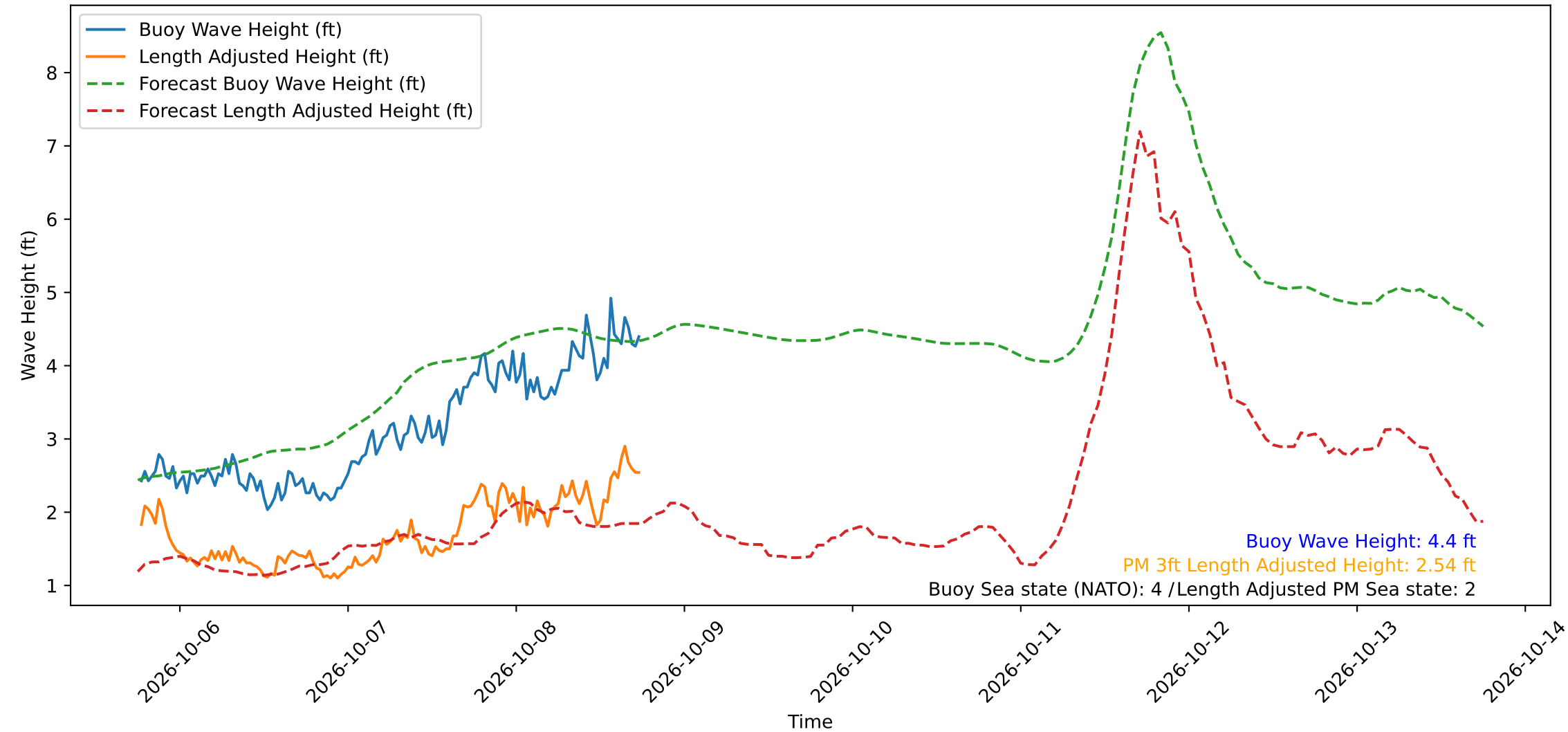
Wave Heights over Time for Oceanside Harbor at 2026-10-08 18:20:30
