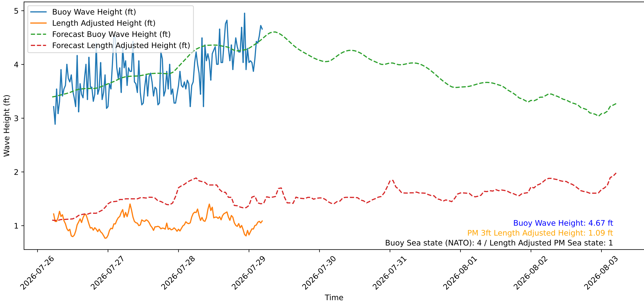
Wave Heights over Time for Red Beach at 2026-07-29 05:10:46
