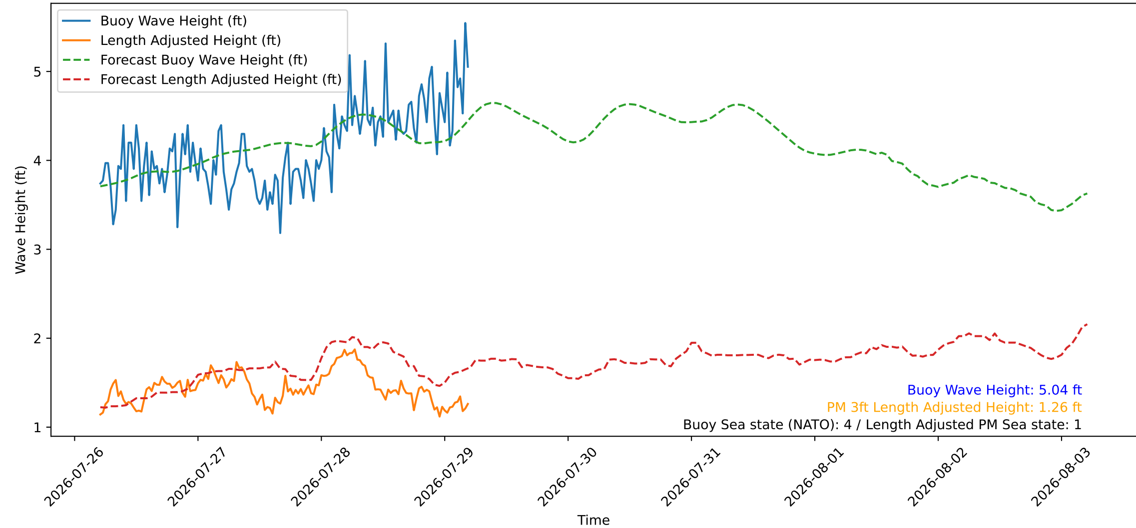
Wave Heights over Time for Oceanside Harbor at 2026-07-29 05:10:27
