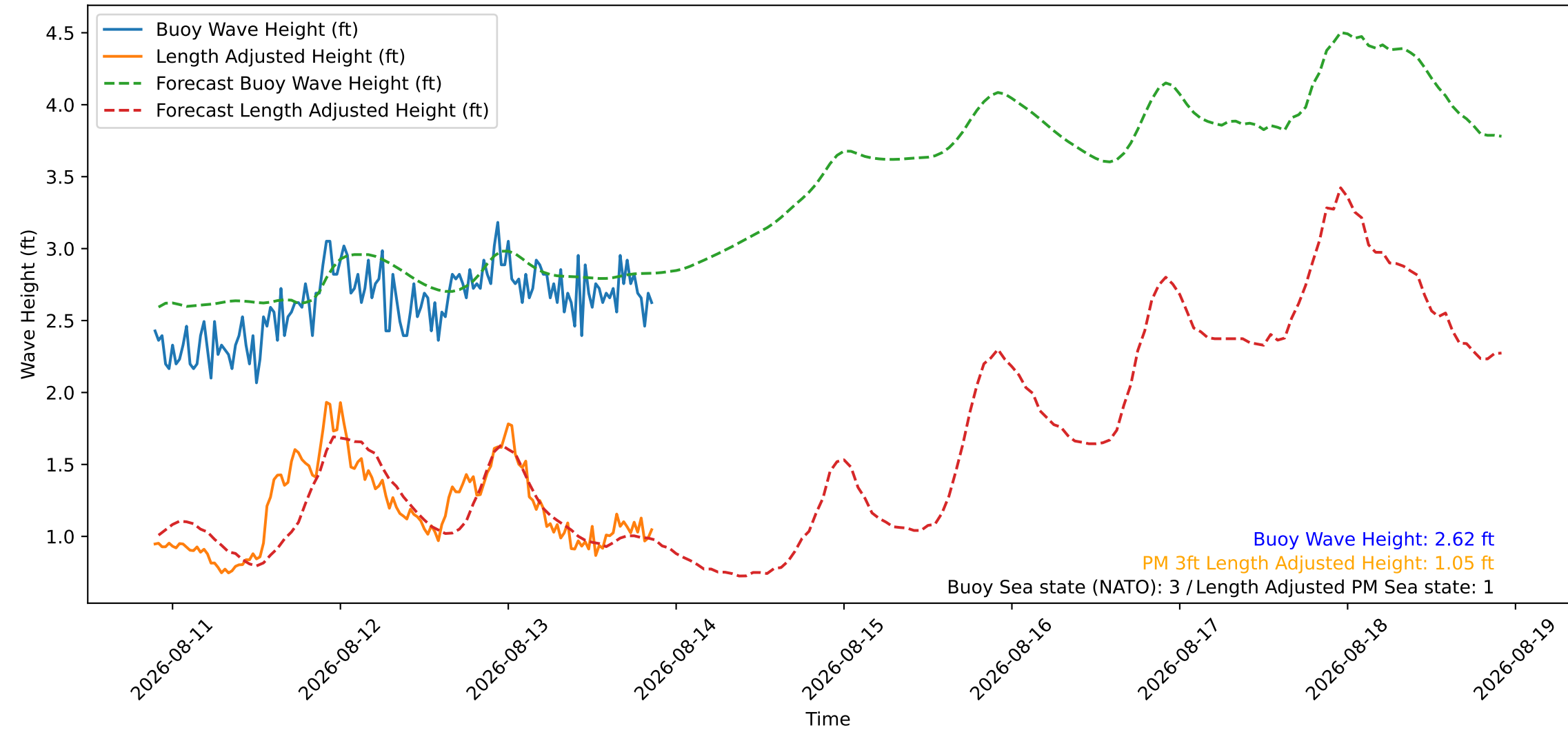
Wave Heights over Time for Oceanside Harbor at 2026-08-13 21:30:27
