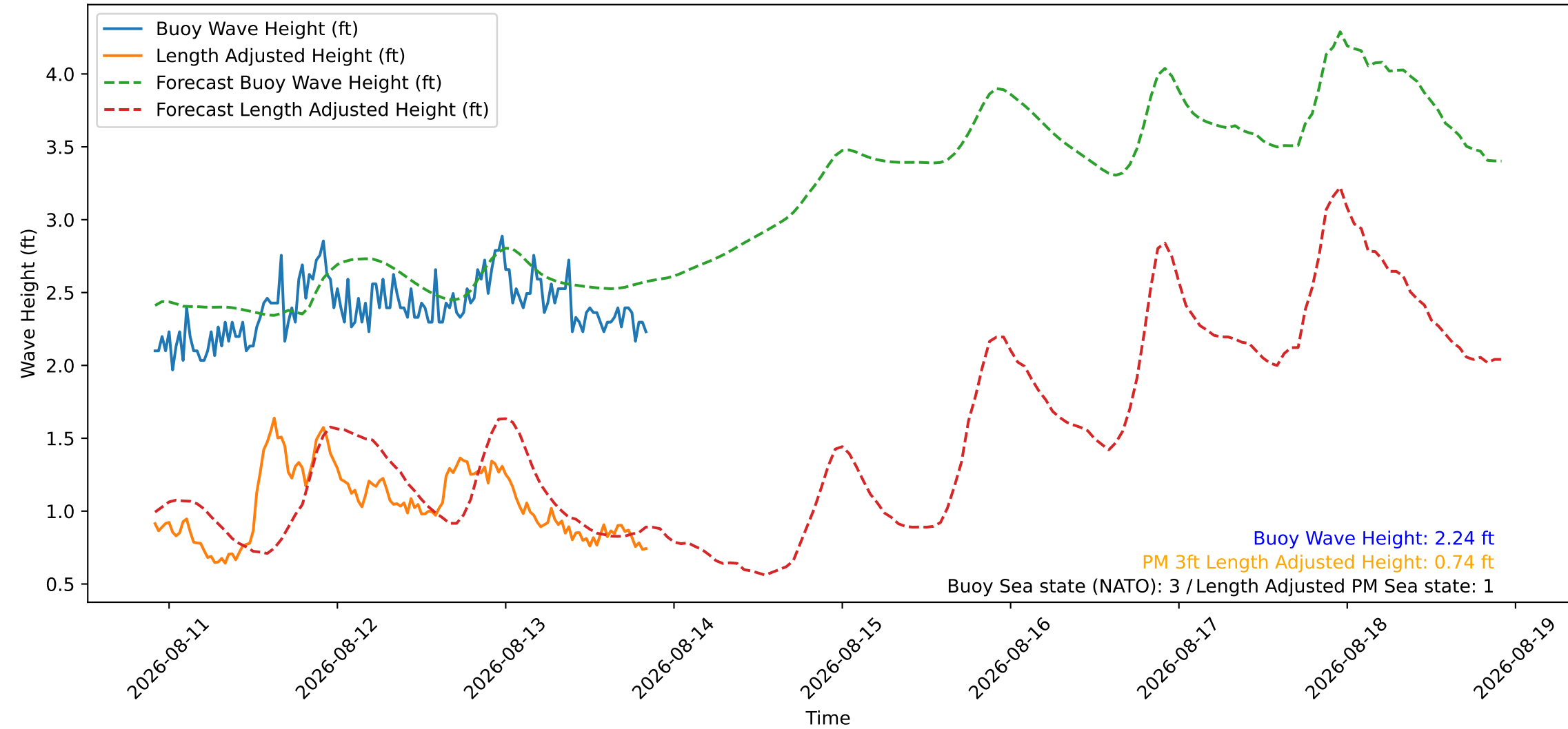
Wave Heights over Time for Red Beach at 2026-08-13 21:30:47
