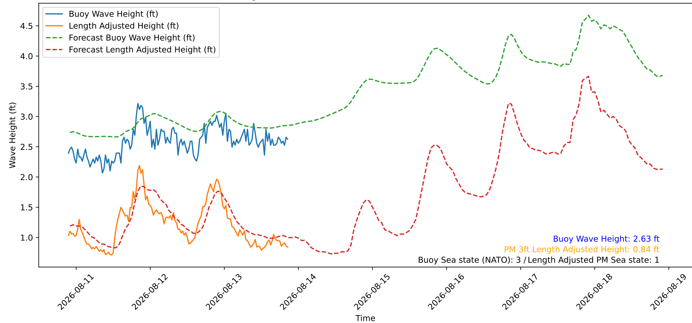
Wave Heights over Time for Green Beach at 2026-08-13 21:31:09
