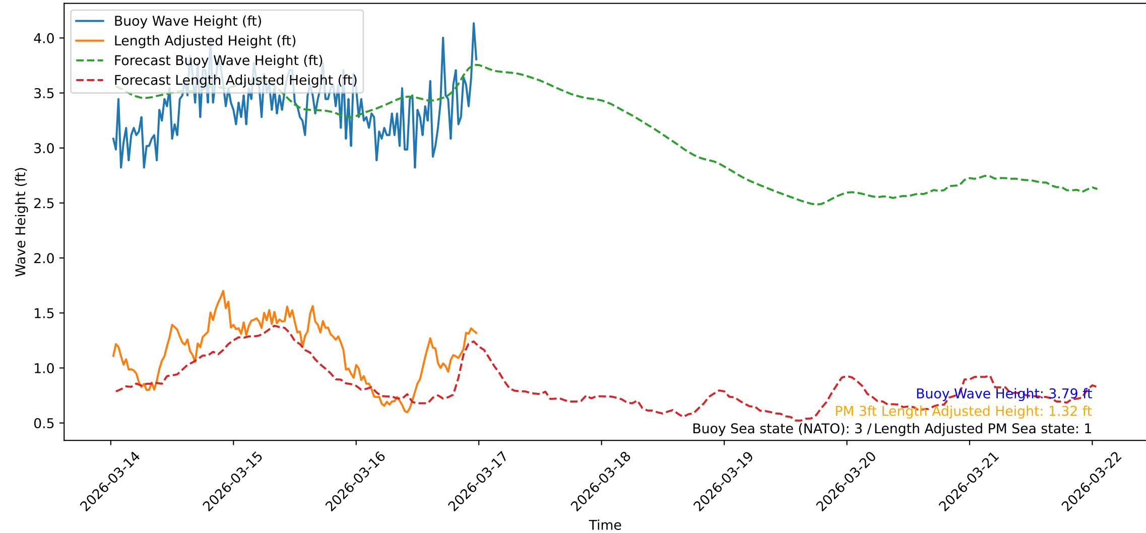
Wave Heights over Time for Green Beach at 2026-03-17 00:31:36
