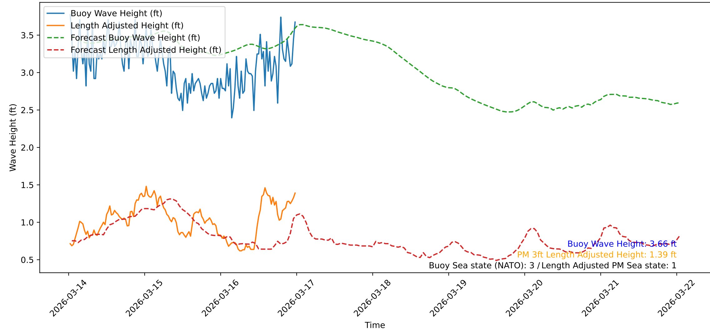
Wave Heights over Time for Oceanside Harbor at 2026-03-17 00:30:42
