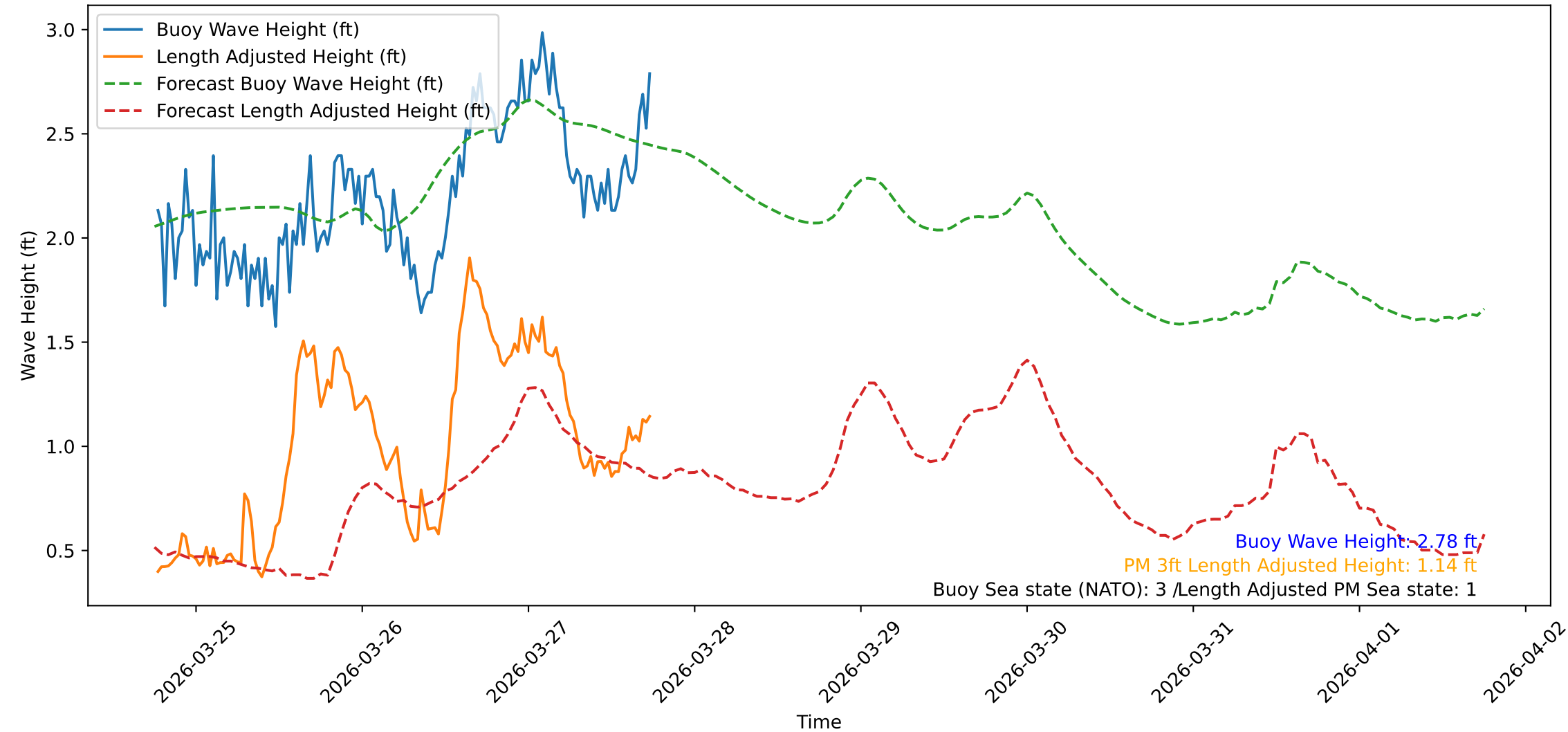
Wave Heights over Time for Red Beach at 2026-03-27 18:10:47
