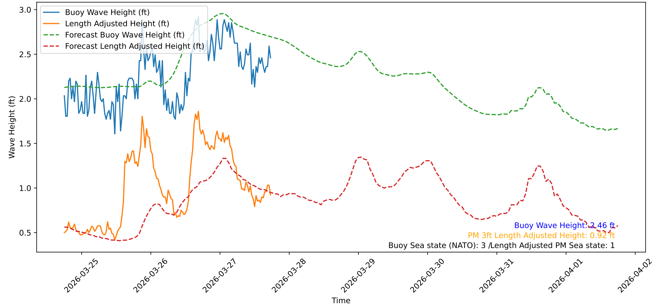
Wave Heights over Time for Oceanside Harbor at 2026-03-27 18:10:31
