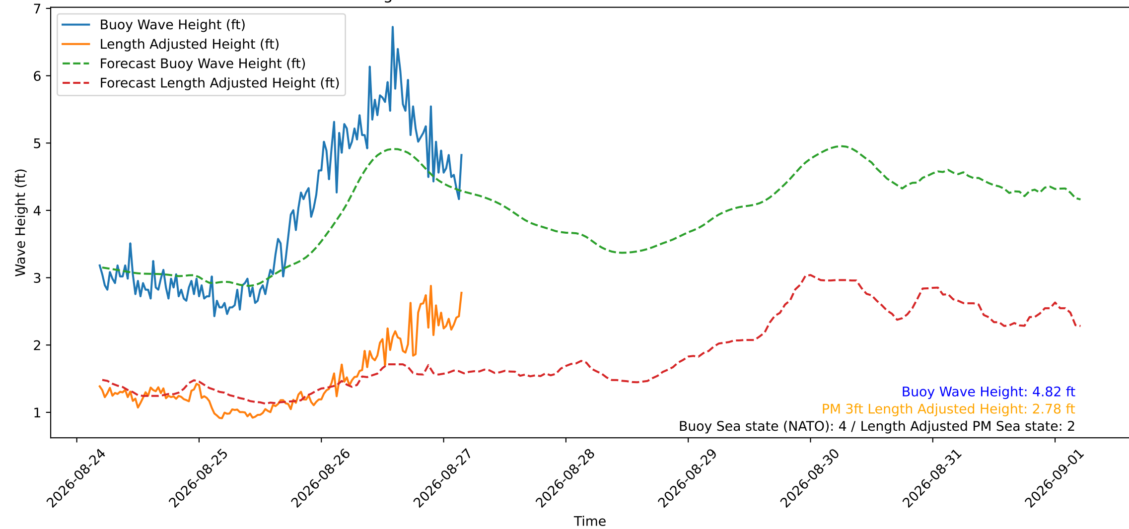
Wave Heights over Time for Oceanside Harbor at 2026-08-27 04:30:29
