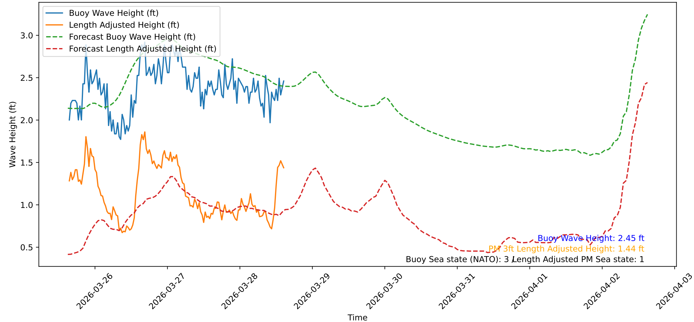
Wave Heights over Time for Oceanside Harbor at 2026-03-28 15:20:32
