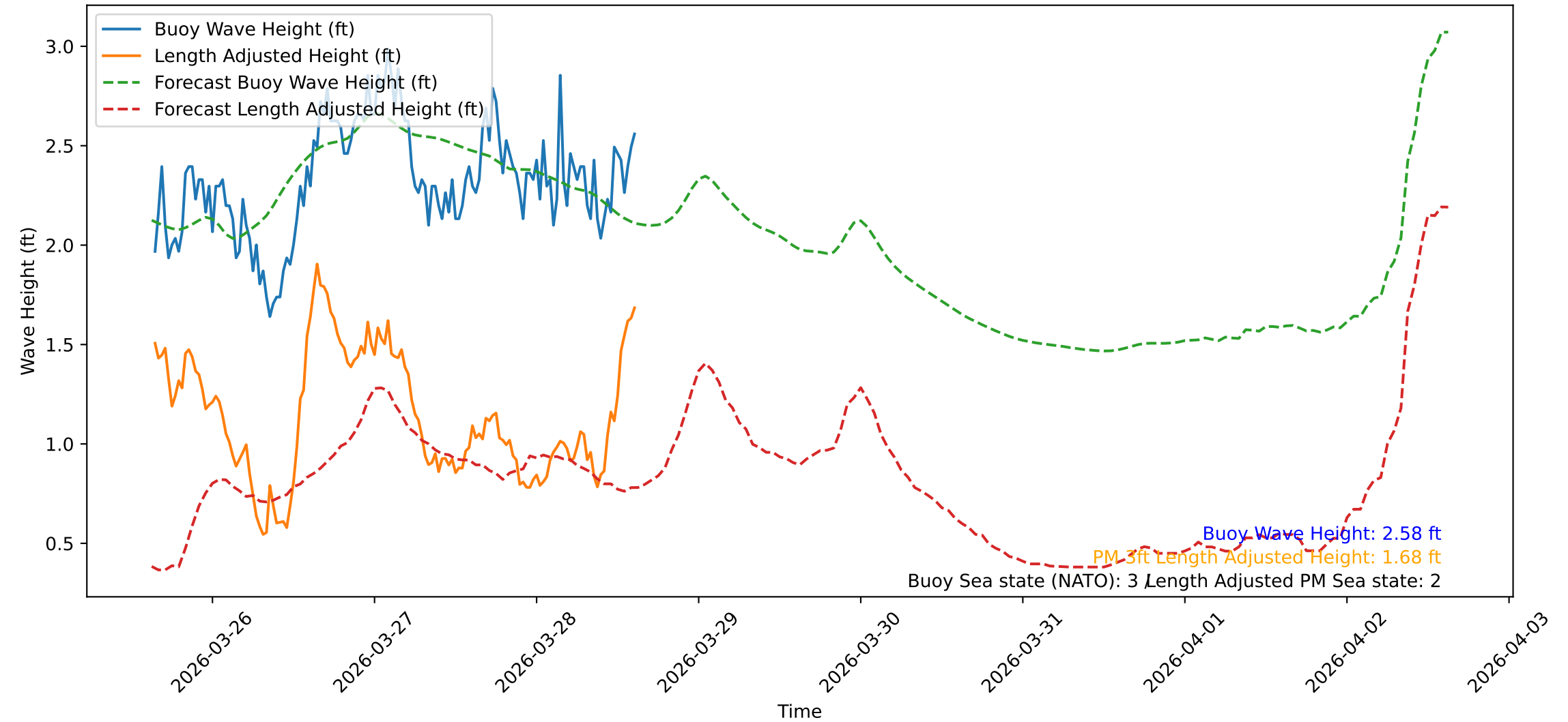
Wave Heights over Time for Red Beach at 2026-03-28 15:20:47
