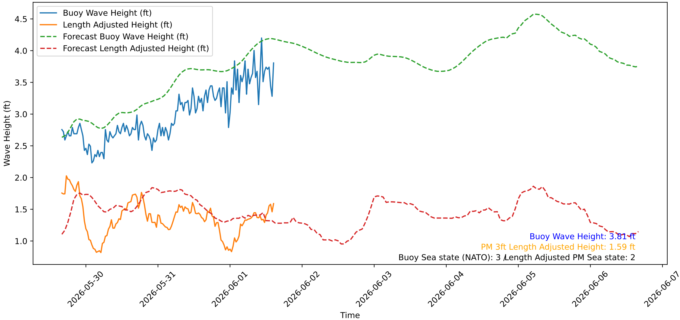
Wave Heights over Time for Red Beach at 2026-06-01 15:30:45
