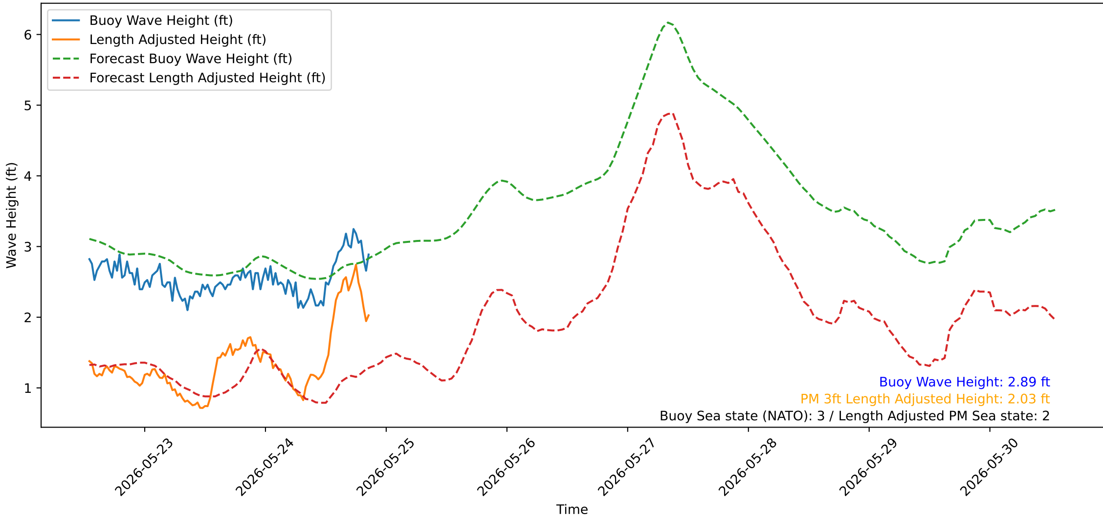
Wave Heights over Time for Oceanside Harbor at 2026-05-25 12:50:30
