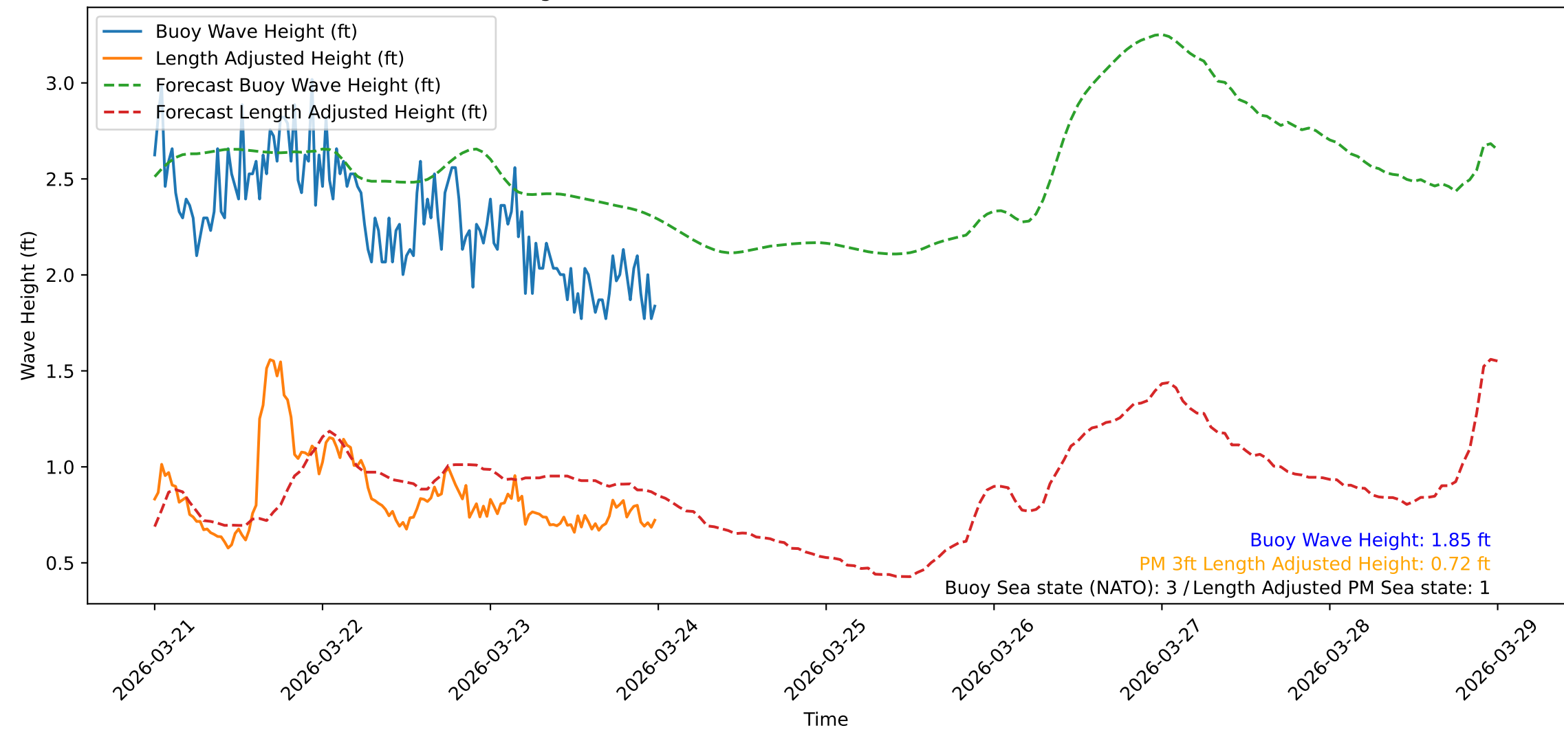
Wave Heights over Time for Oceanside Harbor at 2026-03-24 00:10:31
