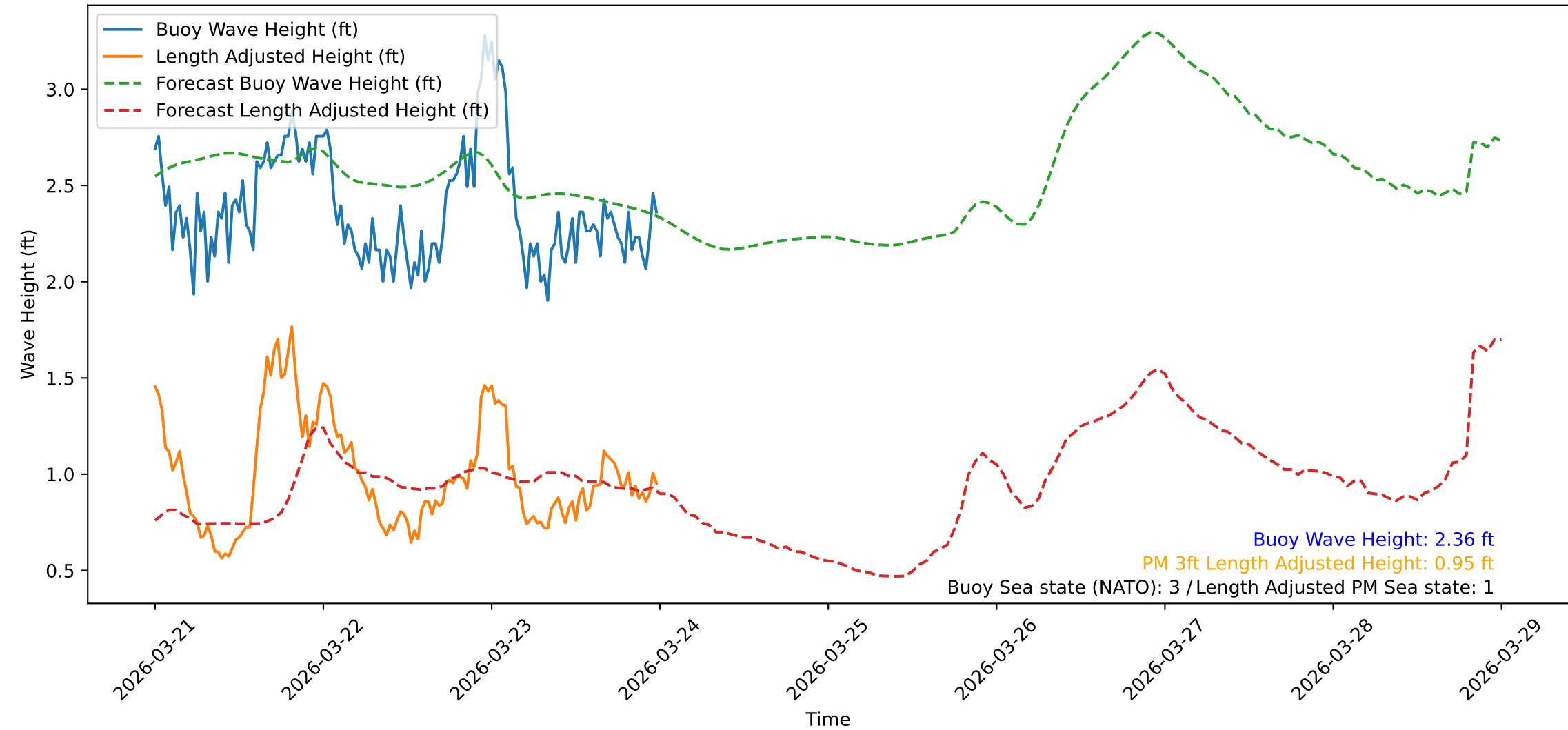
Wave Heights over Time for Green Beach at 2026-03-24 00:11:10
