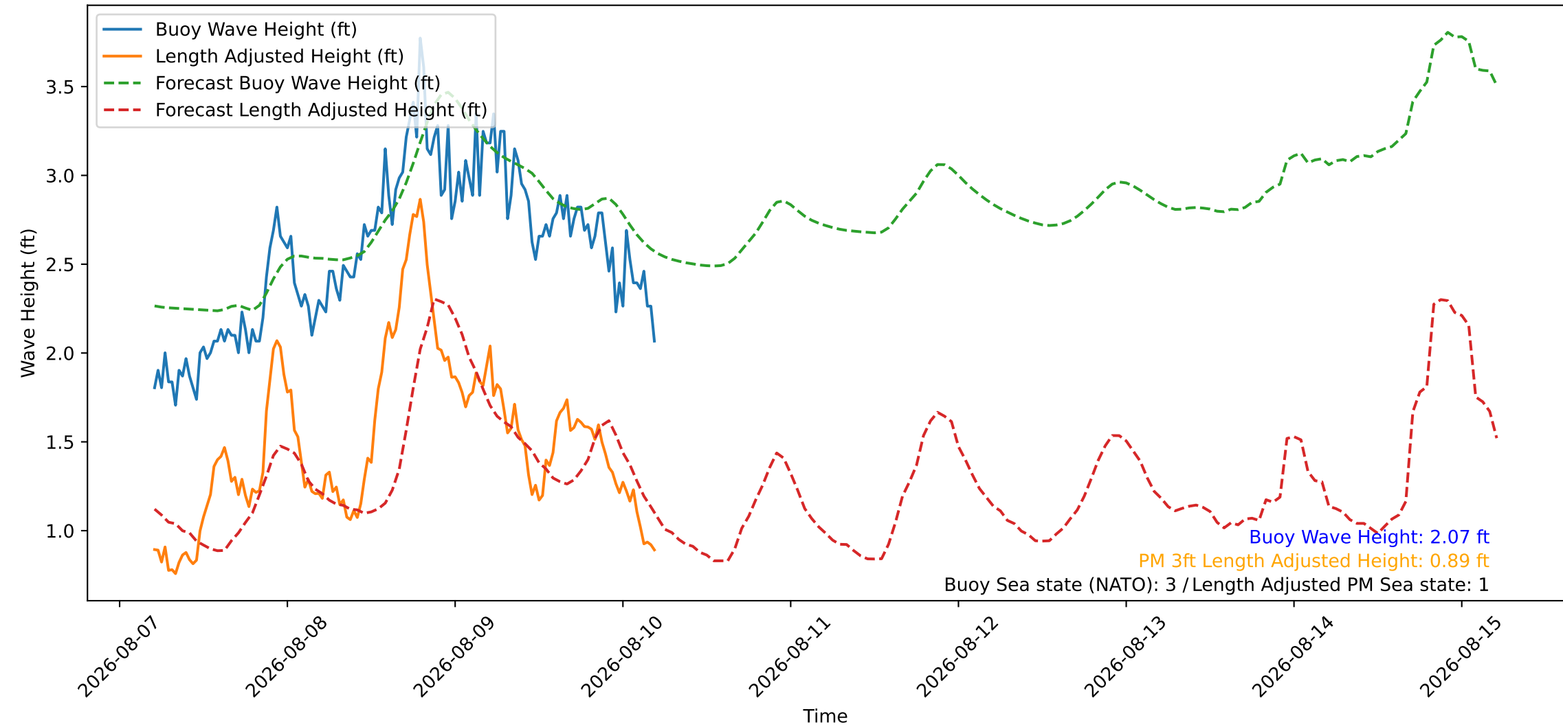
Wave Heights over Time for Green Beach at 2026-08-10 05:11:09
