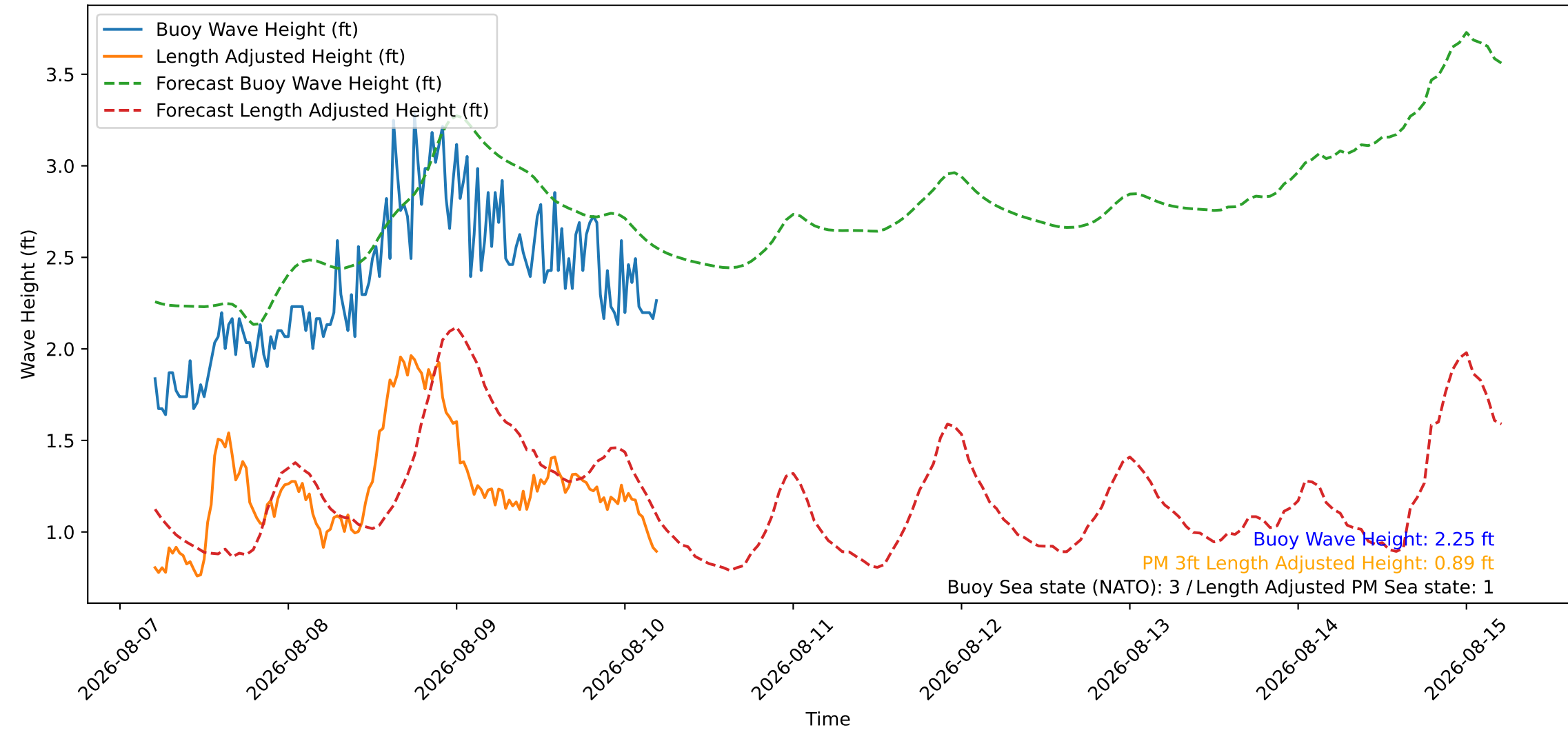
Wave Heights over Time for Oceanside Harbor at 2026-08-10 05:10:27
