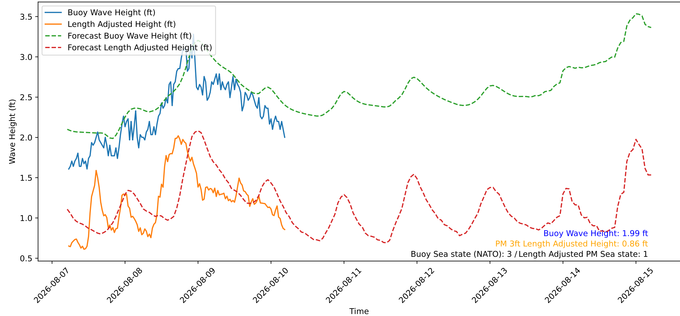
Wave Heights over Time for Red Beach at 2026-08-10 05:10:46
