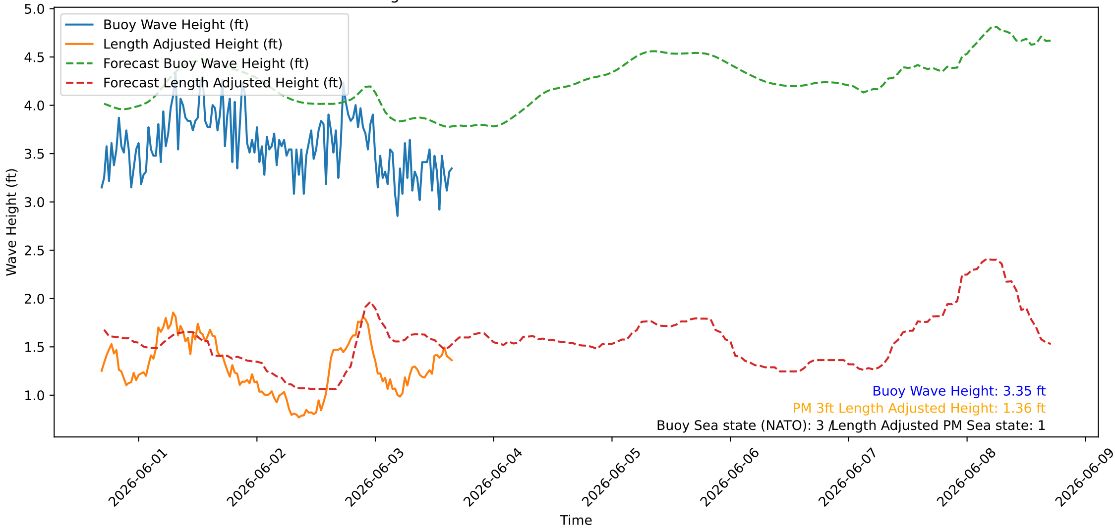
Wave Heights over Time for Green Beach at 2026-06-03 16:41:09
