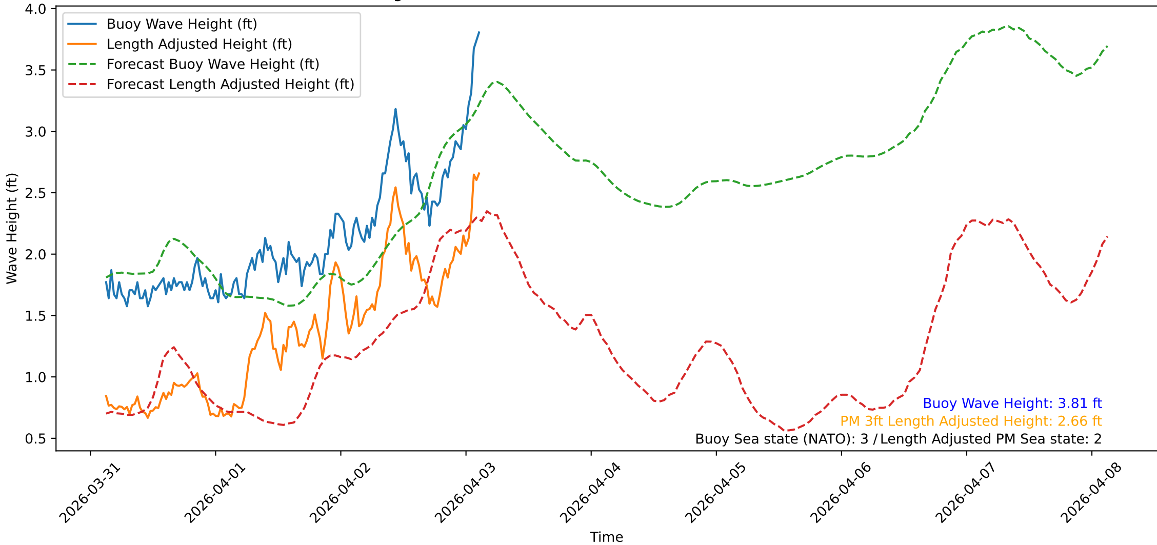
Wave Heights over Time for Oceanside Harbor at 2026-04-03 03:00:31
