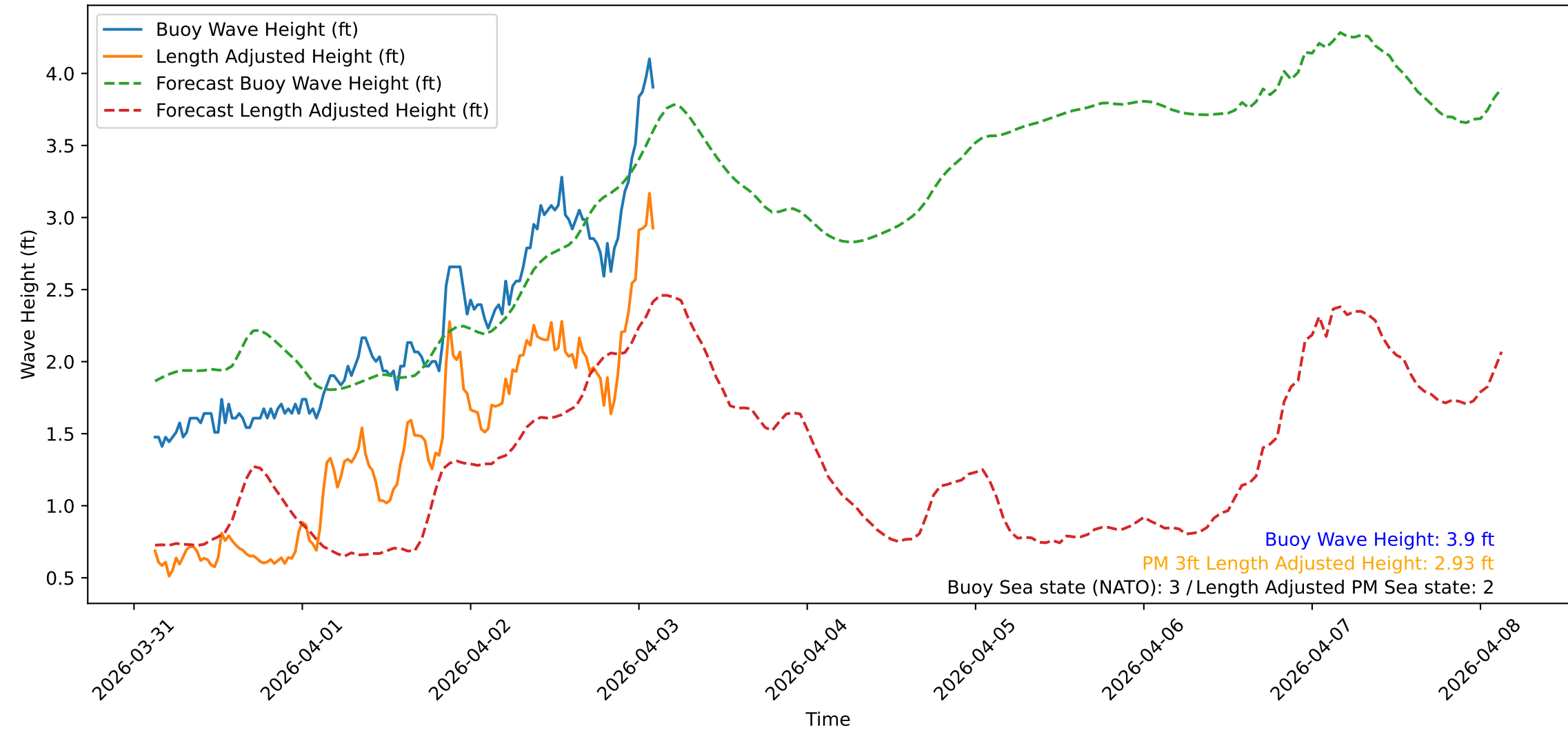
Wave Heights over Time for Green Beach at 2026-04-03 03:01:09
