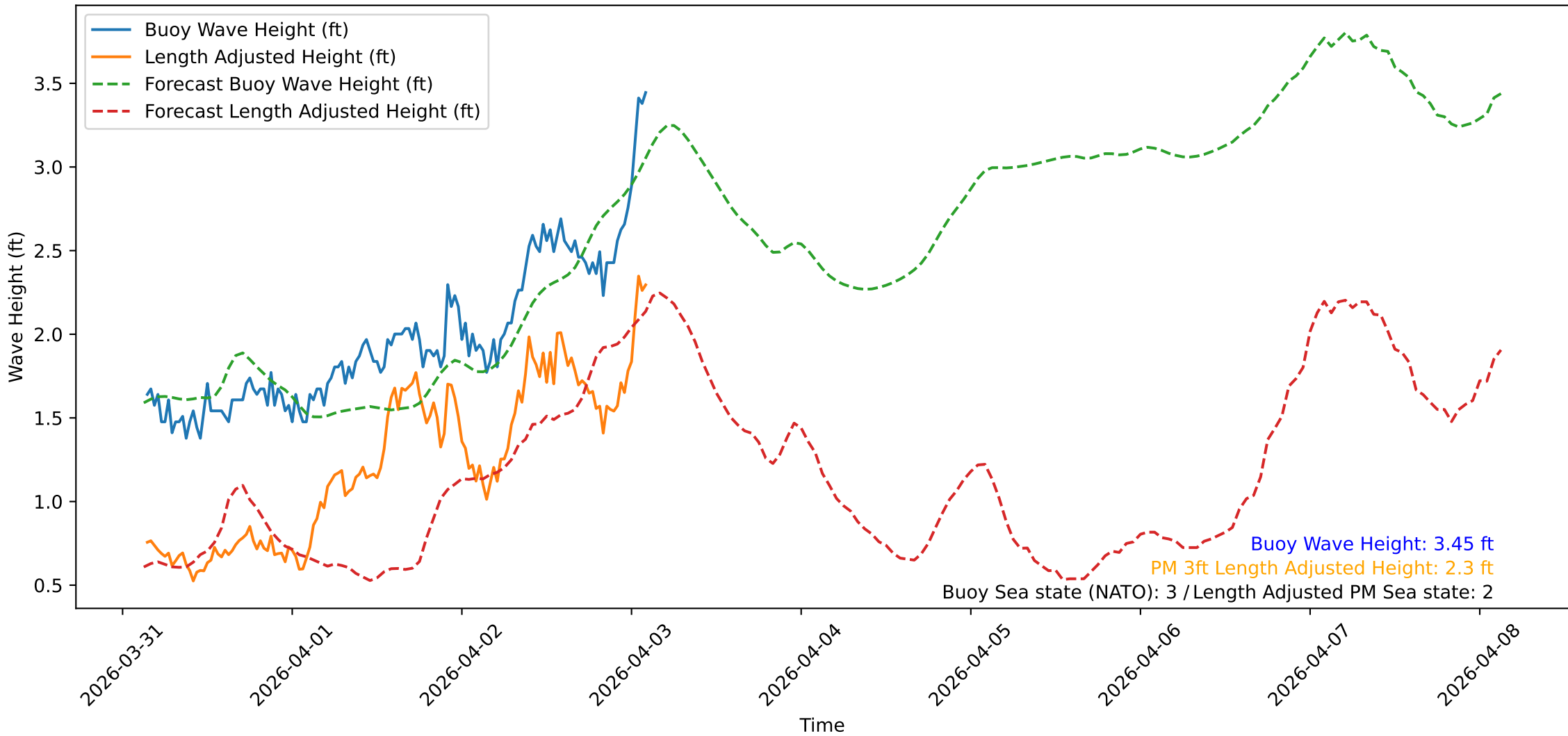
Wave Heights over Time for Red Beach at 2026-04-03 03:00:47
