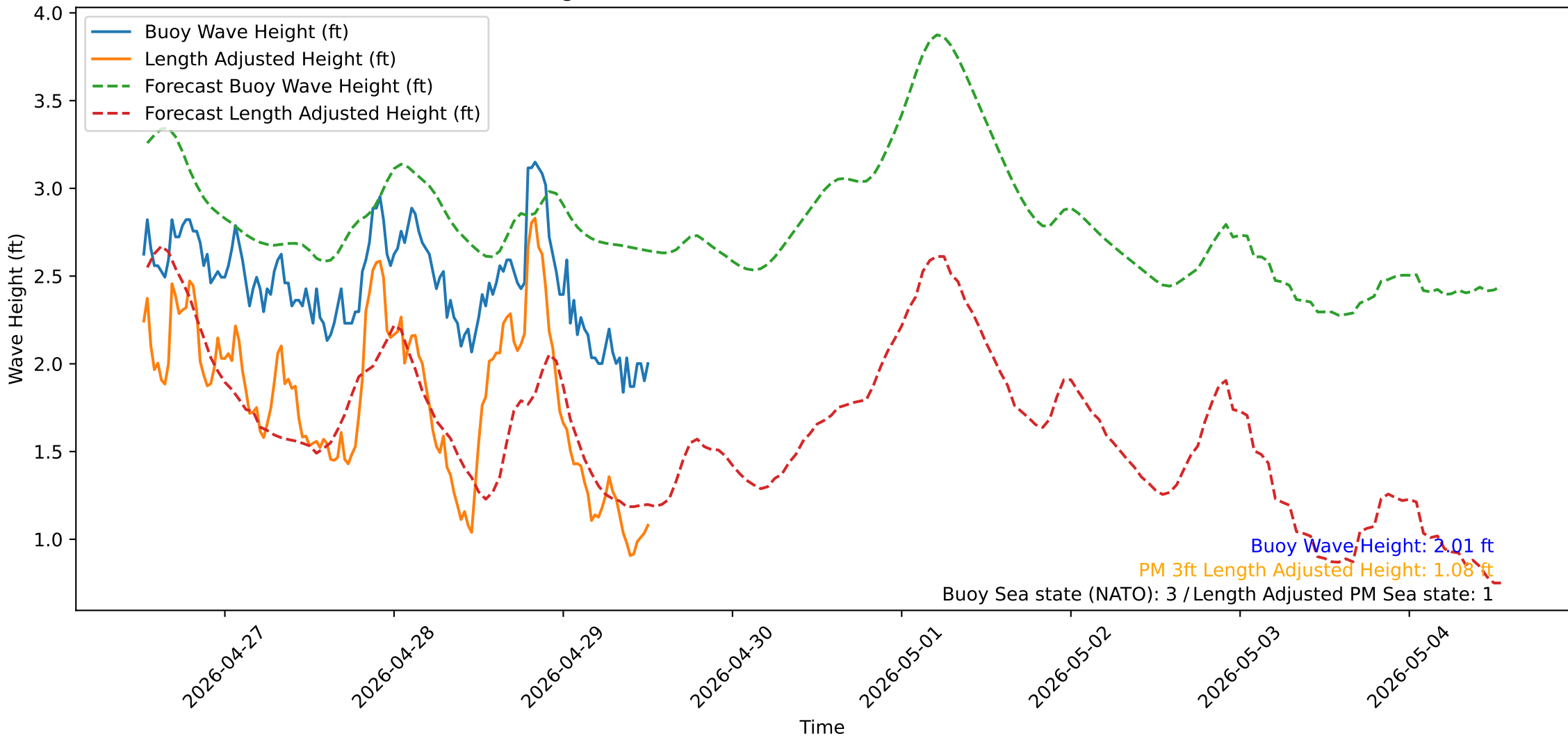
Wave Heights over Time for Green Beach at 2026-04-29 12:41:16
