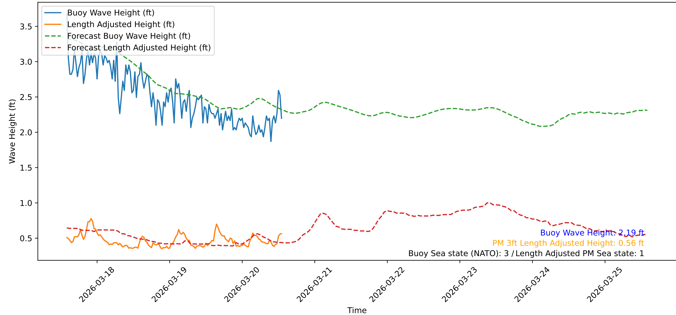
Wave Heights over Time for Red Beach at 2026-03-20 13:40:49
