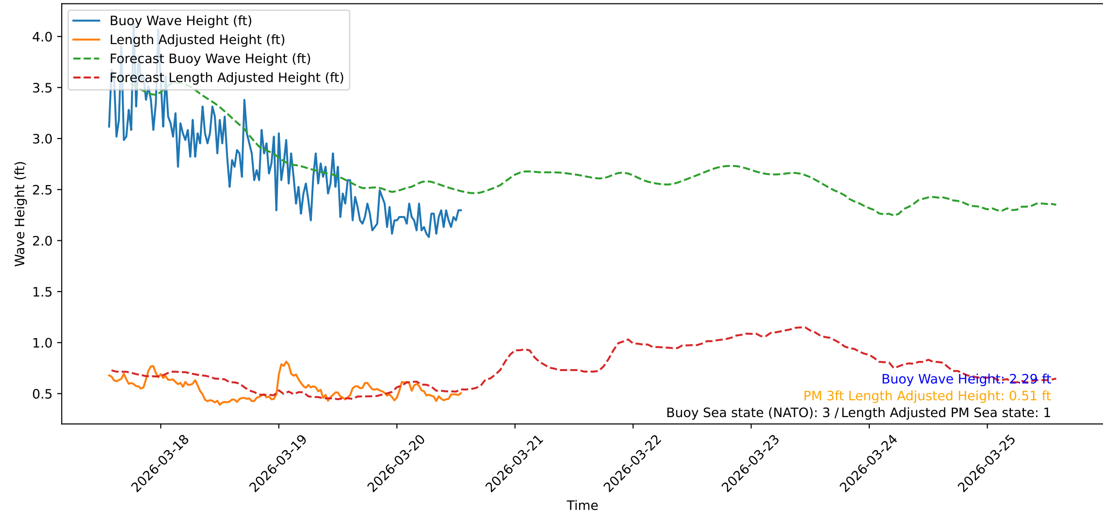
Wave Heights over Time for Green Beach at 2026-03-20 13:41:12
