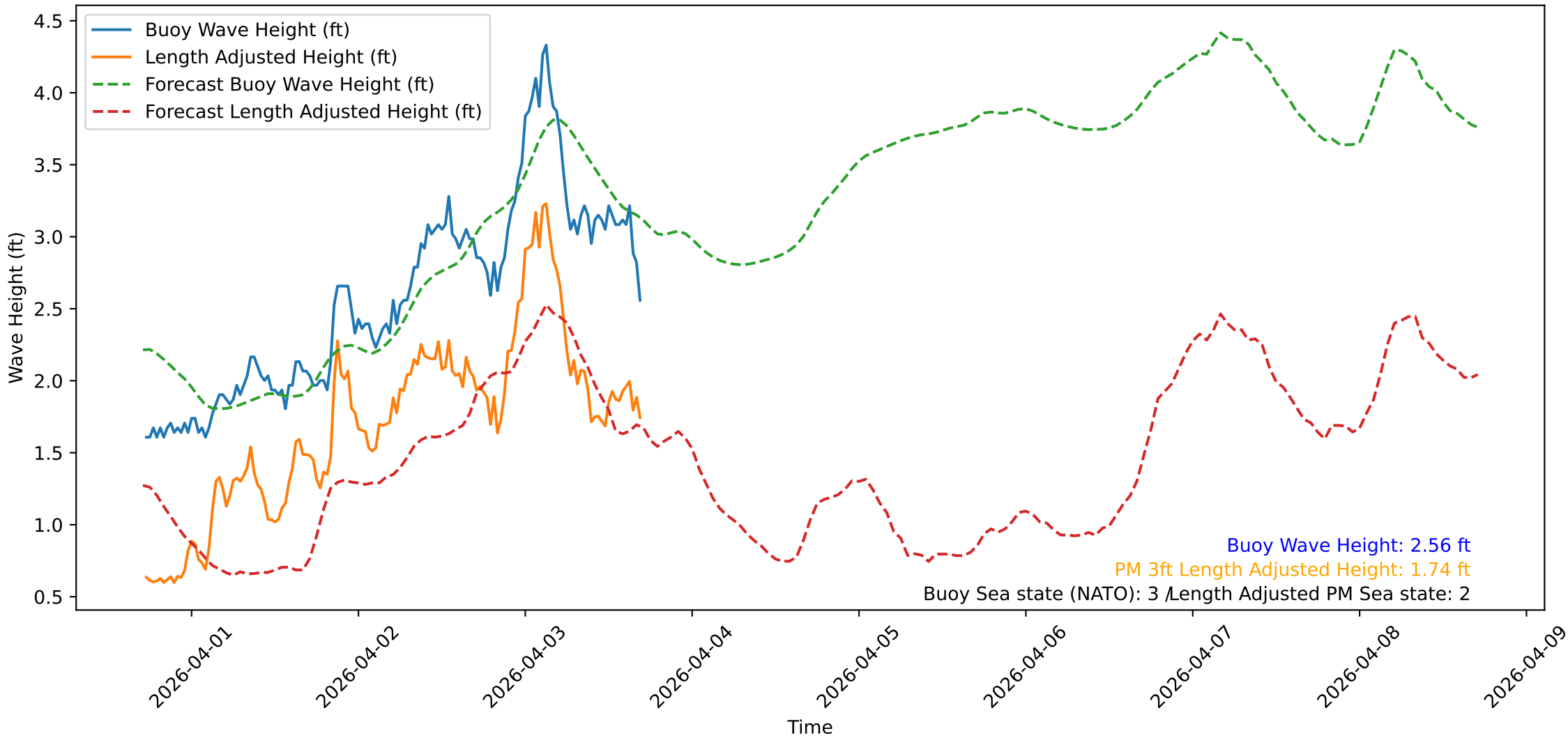
Wave Heights over Time for Green Beach at 2026-04-03 17:21:11
