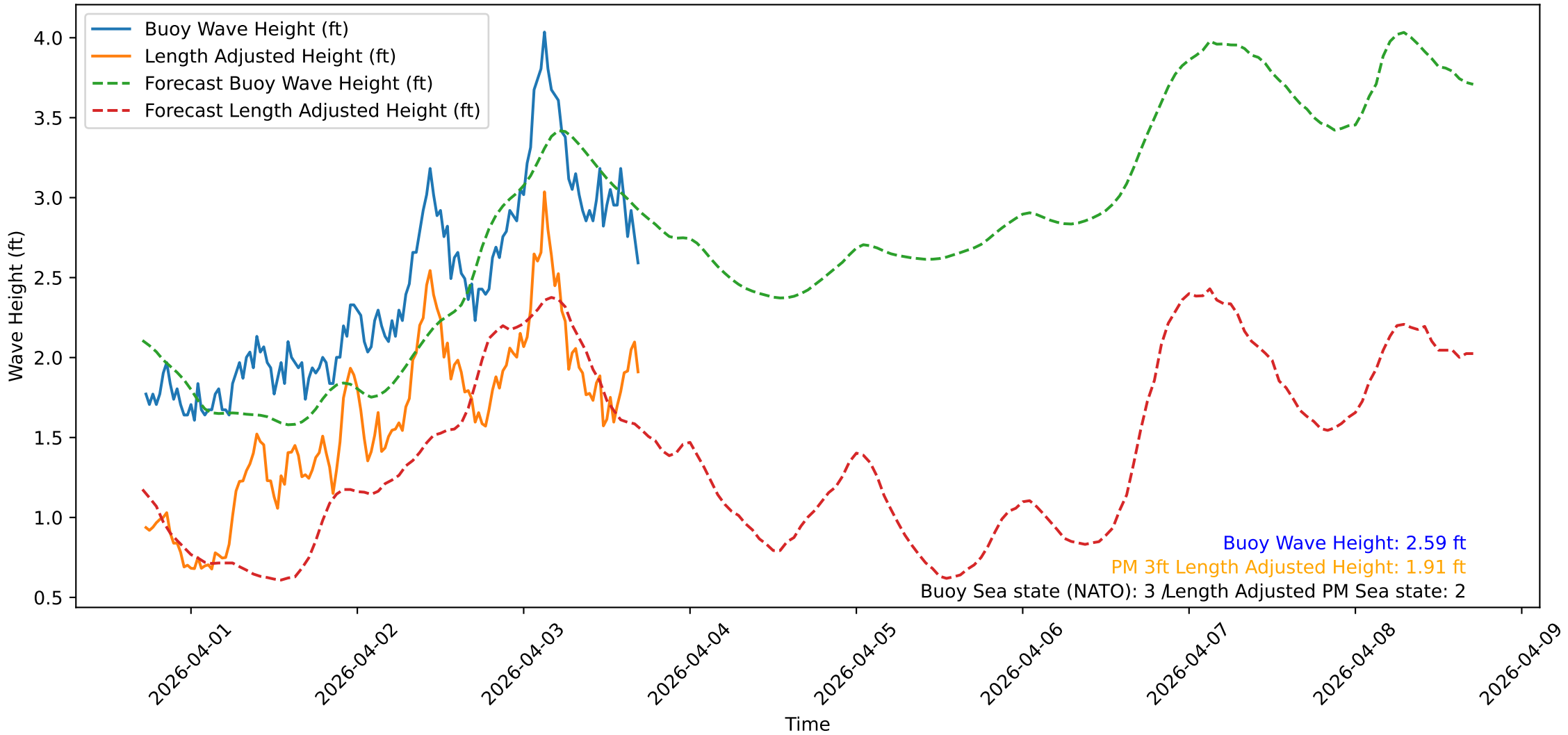
Wave Heights over Time for Oceanside Harbor at 2026-04-03 17:20:32
