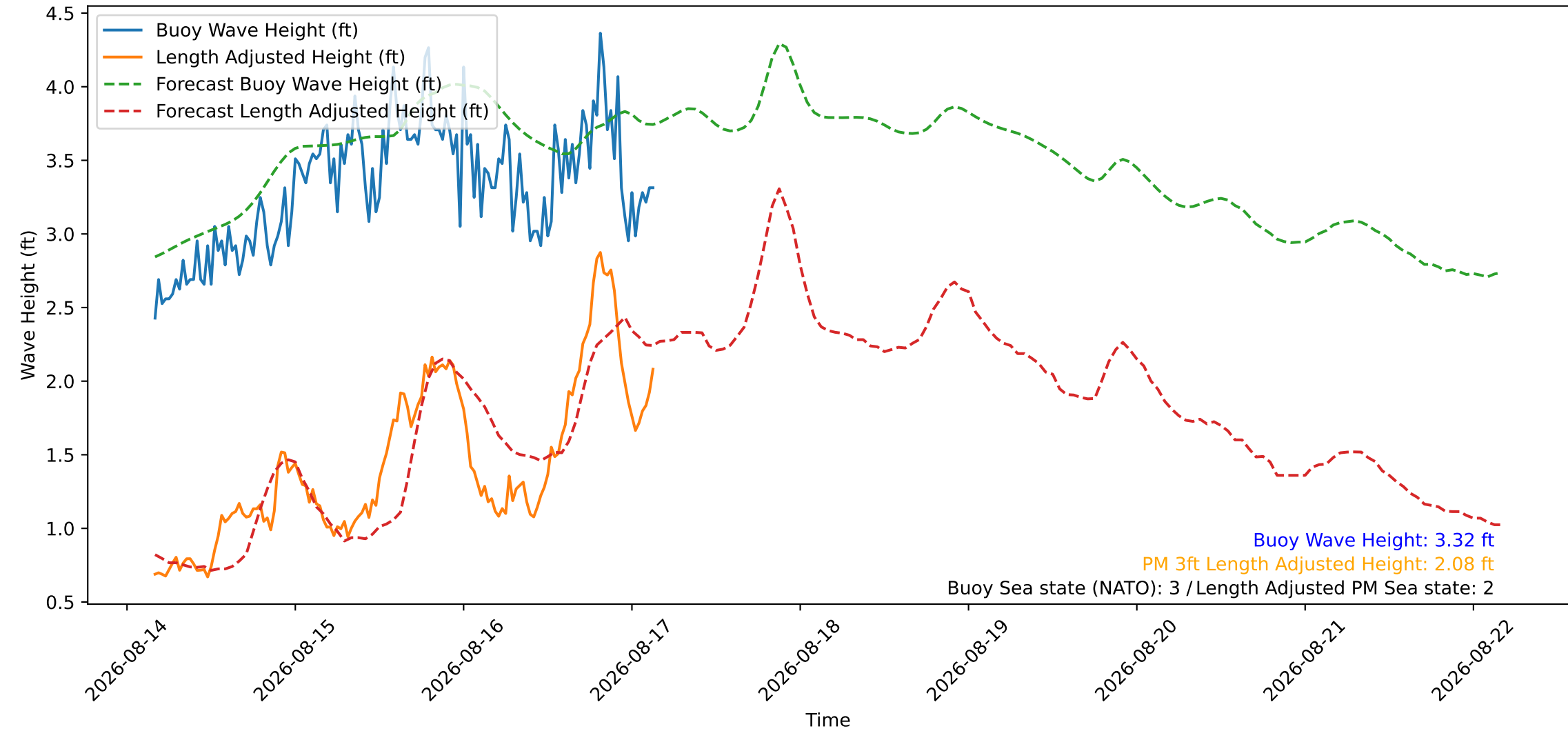
Wave Heights over Time for Green Beach at 2026-08-17 03:41:09
