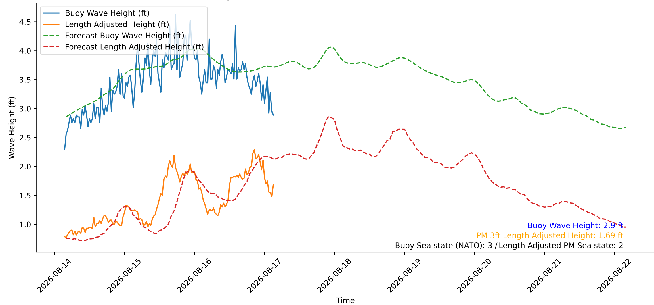
Wave Heights over Time for Oceanside Harbor at 2026-08-17 03:40:27
