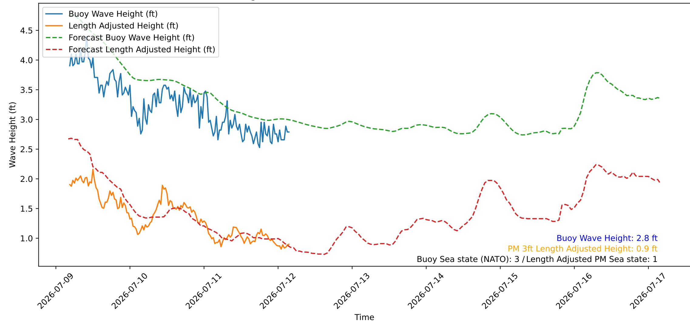
Wave Heights over Time for Green Beach at 2026-07-12 04:21:09
