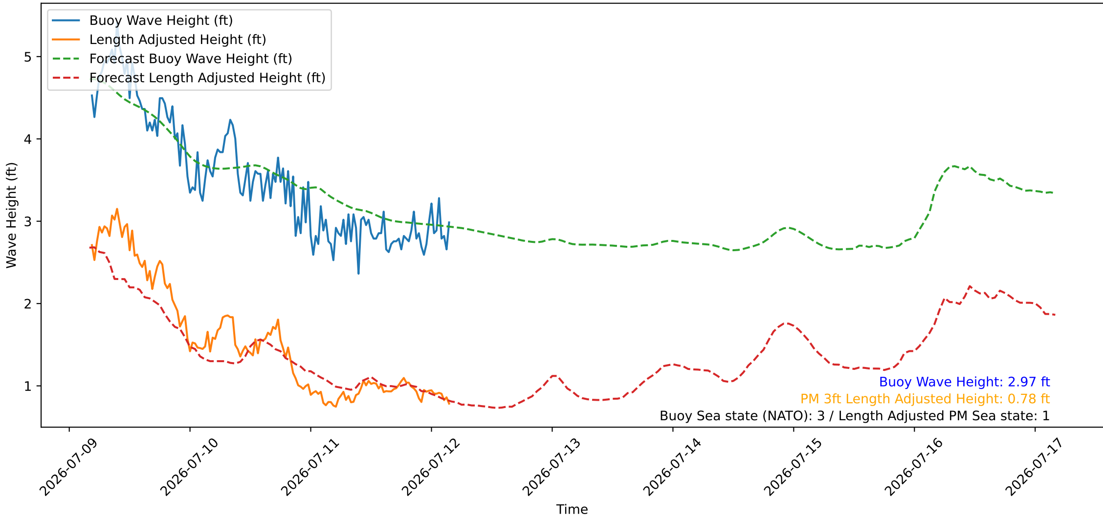
Wave Heights over Time for Oceanside Harbor at 2026-07-12 04:20:26
