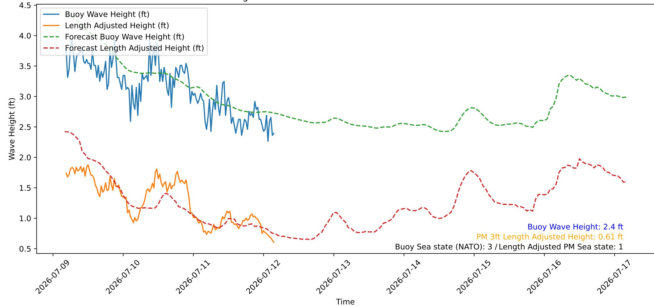
Wave Heights over Time for Red Beach at 2026-07-12 04:20:47
