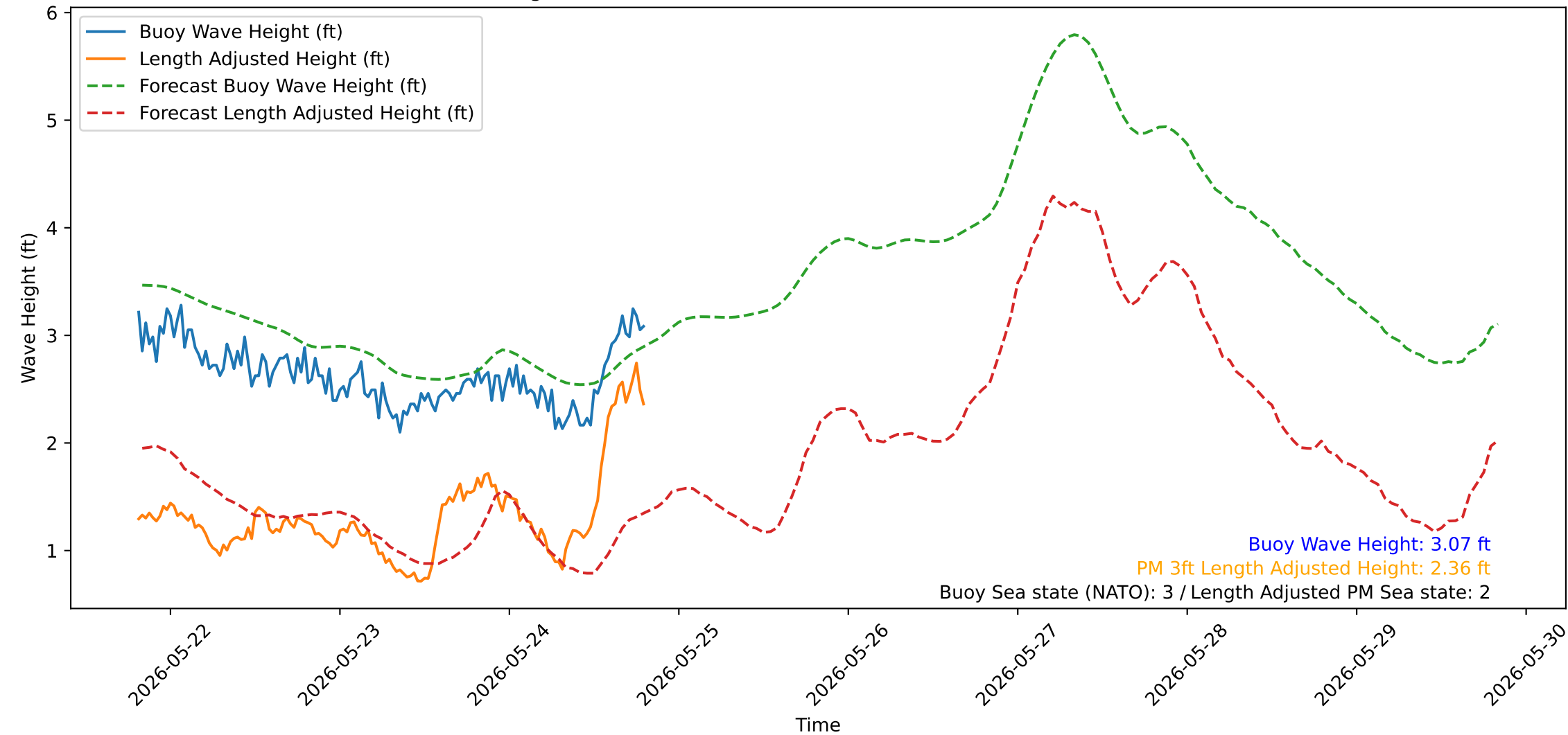
Wave Heights over Time for Oceanside Harbor at 2026-05-24 19:40:31
