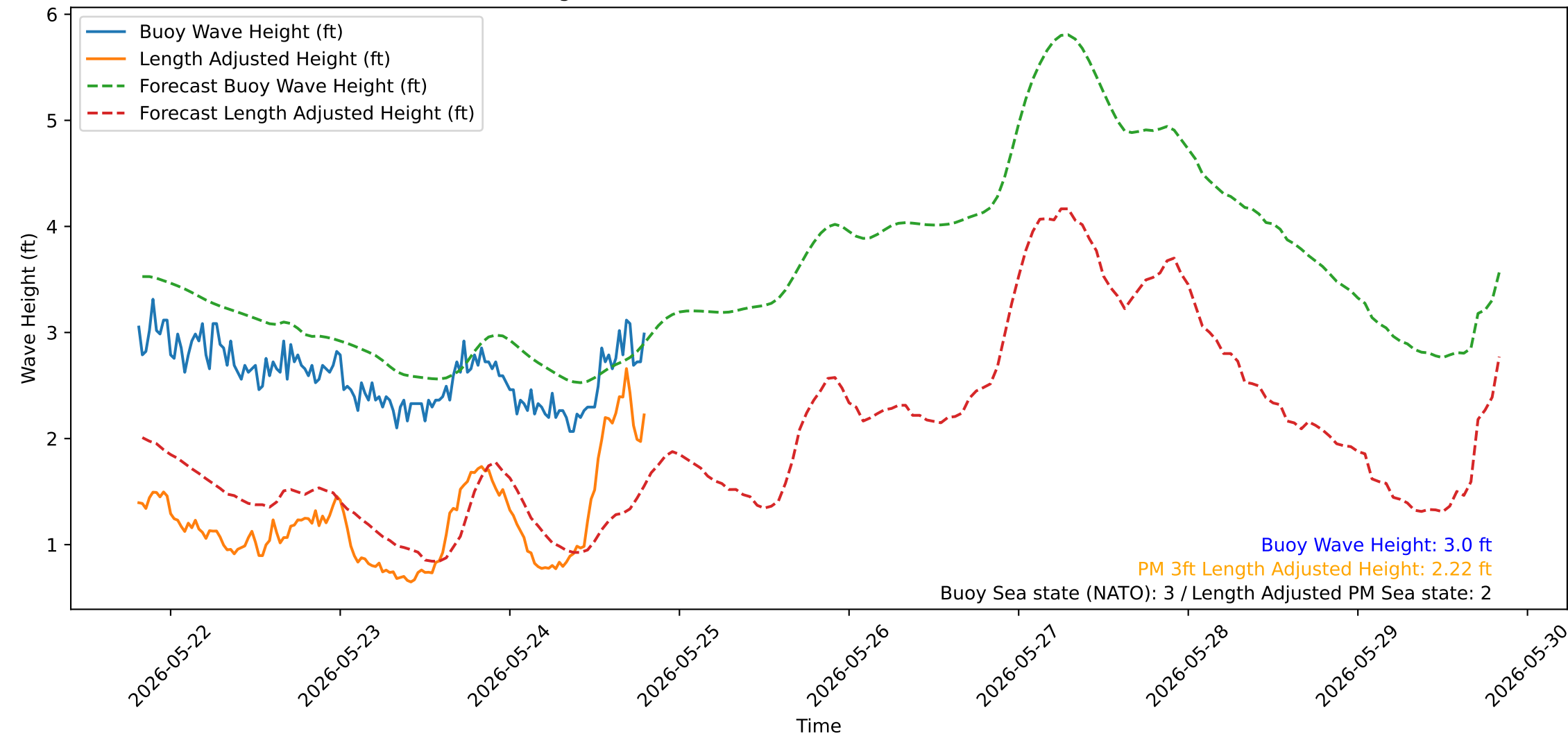
Wave Heights over Time for Green Beach at 2026-05-24 19:41:14
