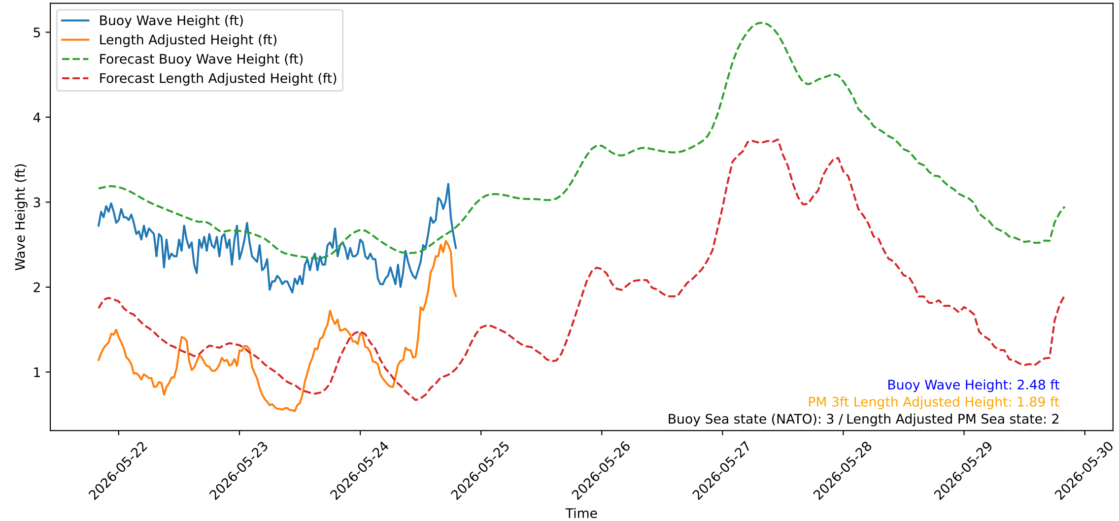
Wave Heights over Time for Red Beach at 2026-05-24 19:40:51
