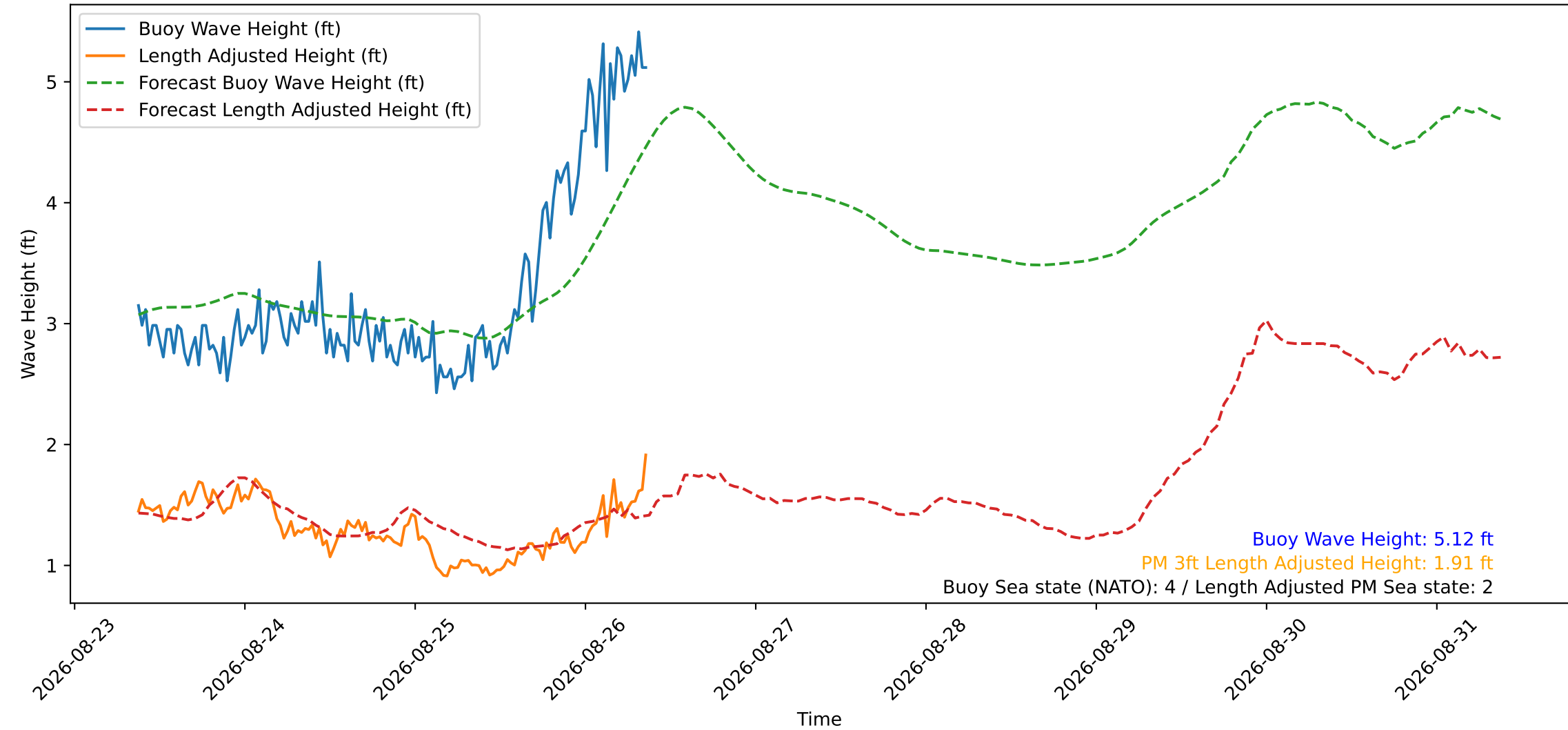
Wave Heights over Time for Oceanside Harbor at 2026-08-26 09:10:30
