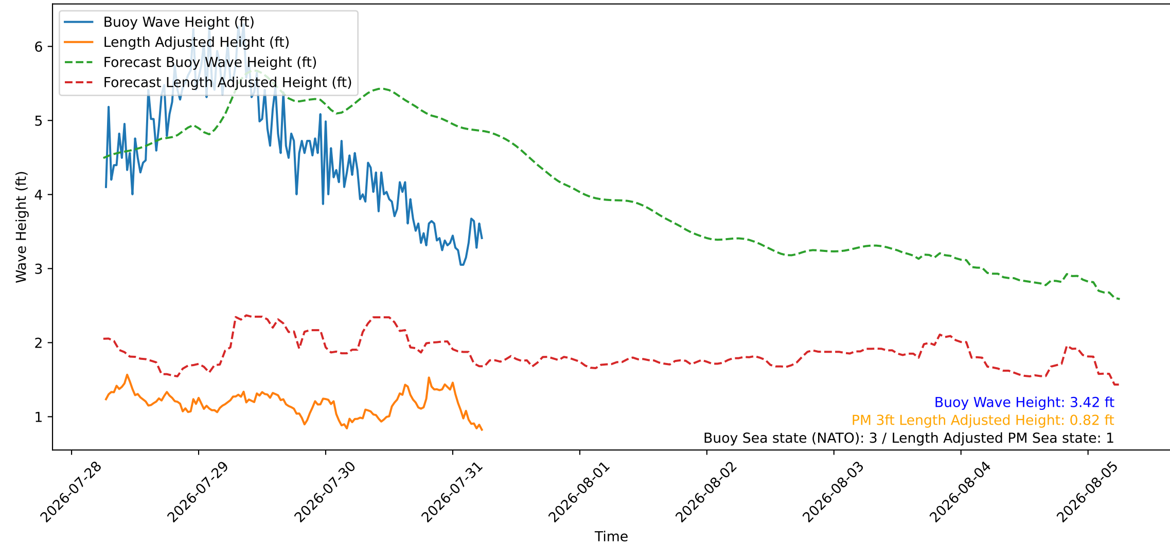
Wave Heights over Time for Green Beach at 2026-07-31 06:21:09
