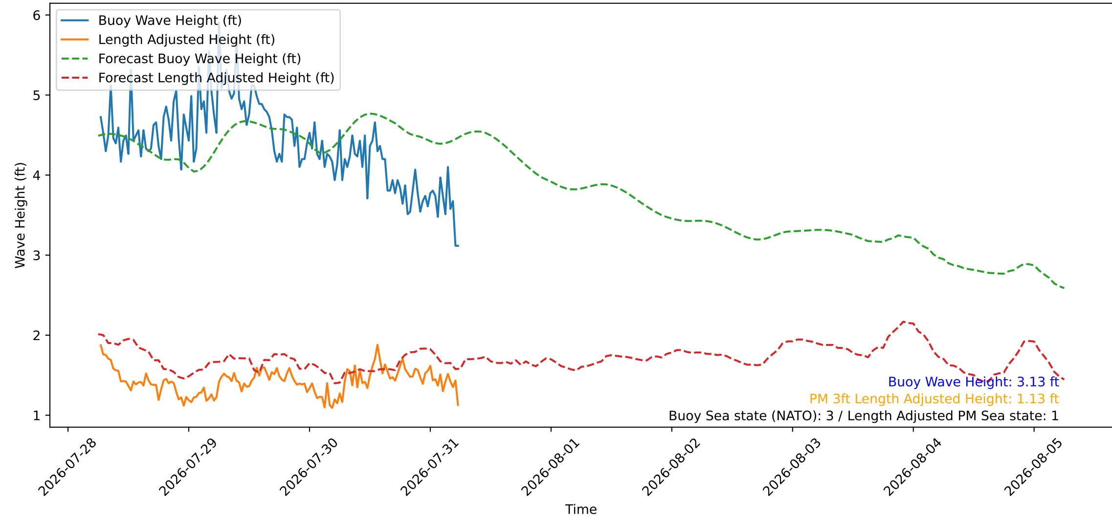
Wave Heights over Time for Oceanside Harbor at 2026-07-31 06:20:26
