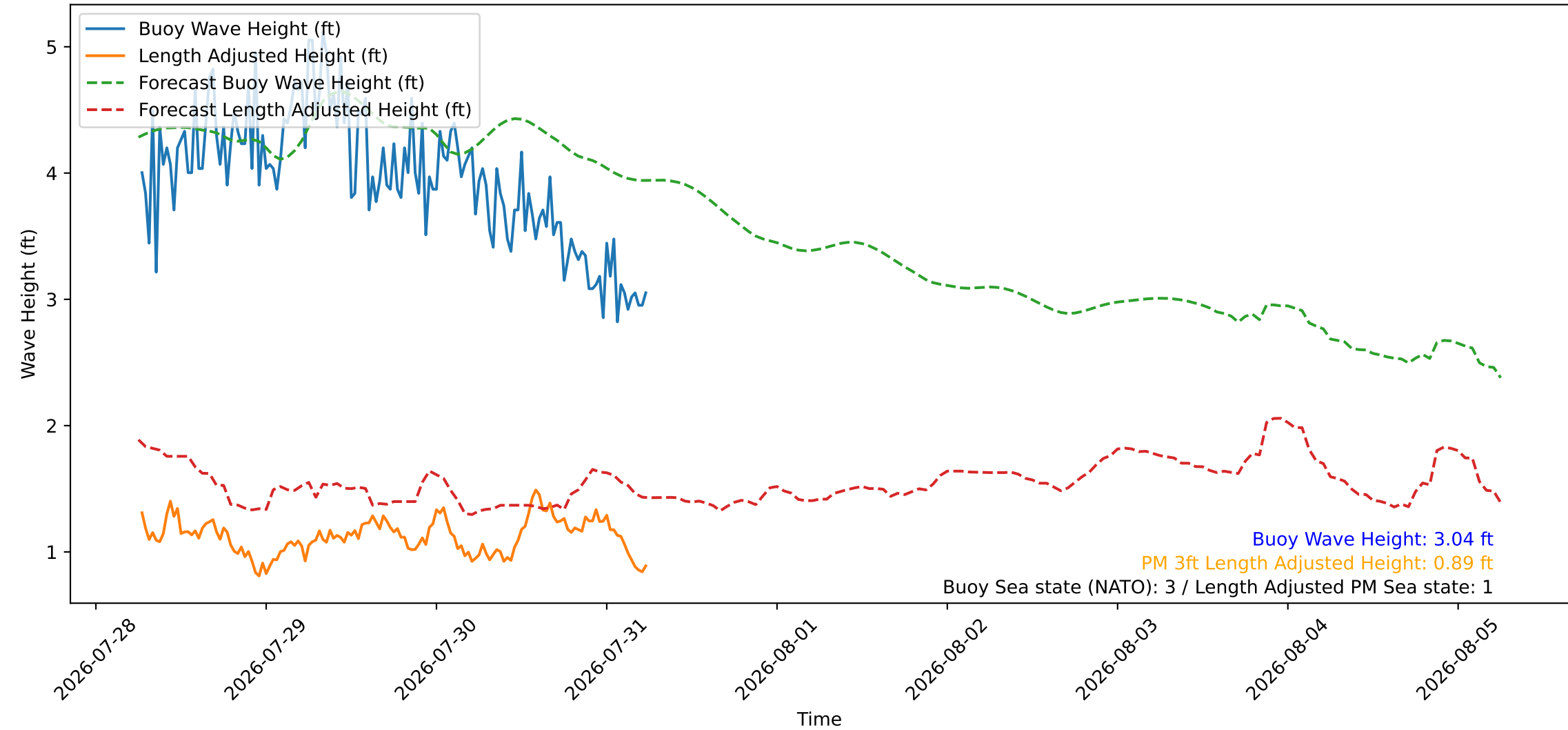
Wave Heights over Time for Red Beach at 2026-07-31 06:20:47
