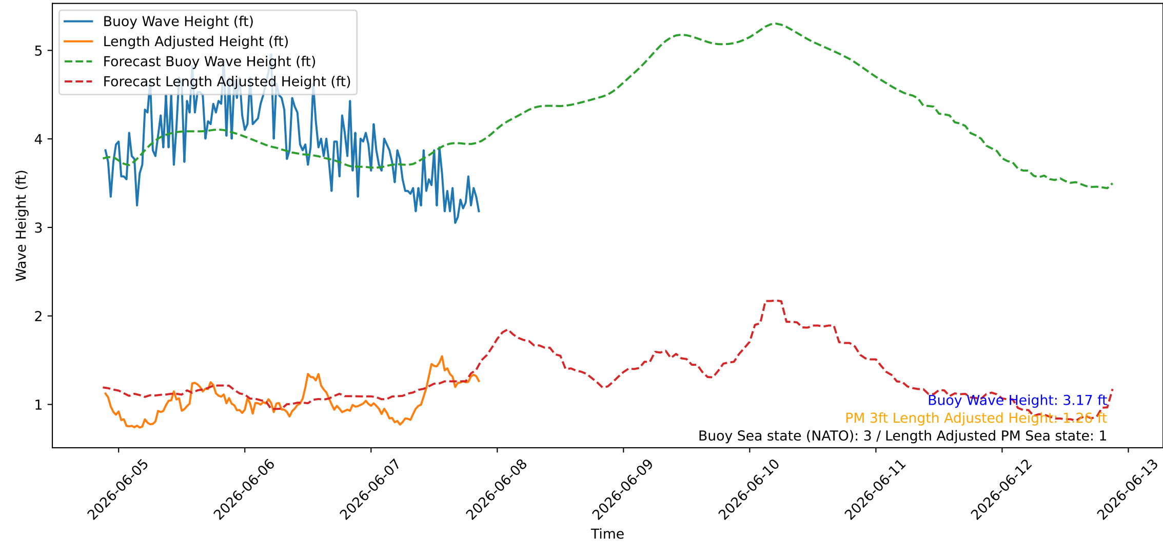
Wave Heights over Time for Red Beach at 2026-06-07 21:20:46
