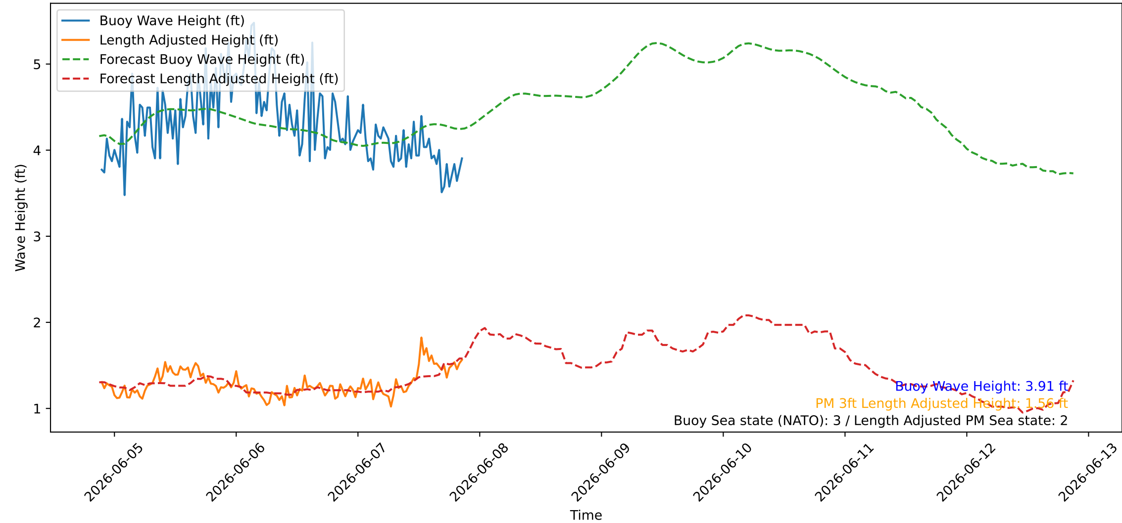
Wave Heights over Time for Oceanside Harbor at 2026-06-07 21:20:25
