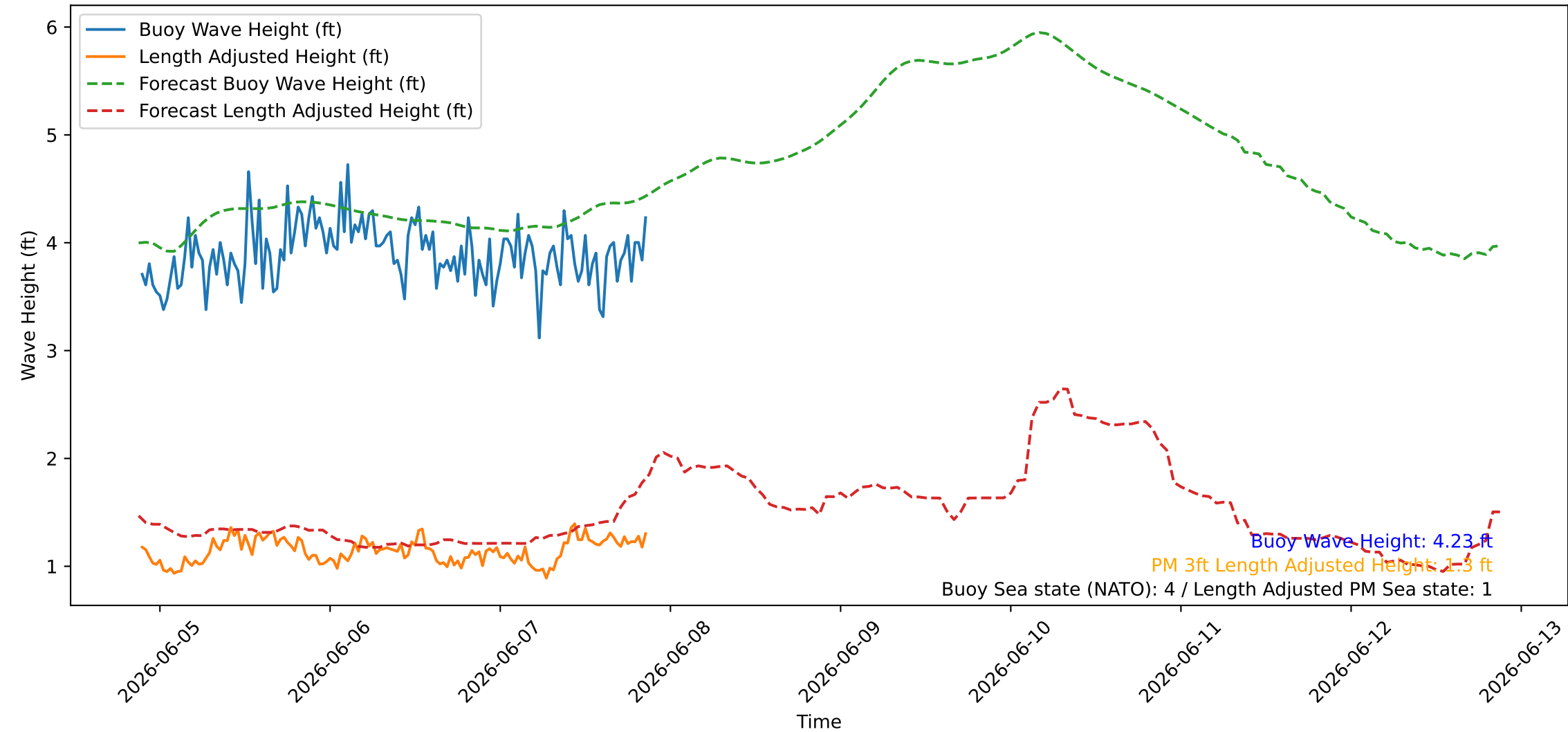
Wave Heights over Time for Green Beach at 2026-06-07 21:21:09
