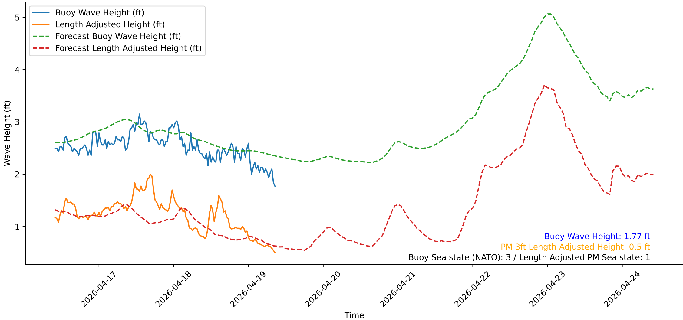
Wave Heights over Time for Red Beach at 2026-04-19 09:30:50
