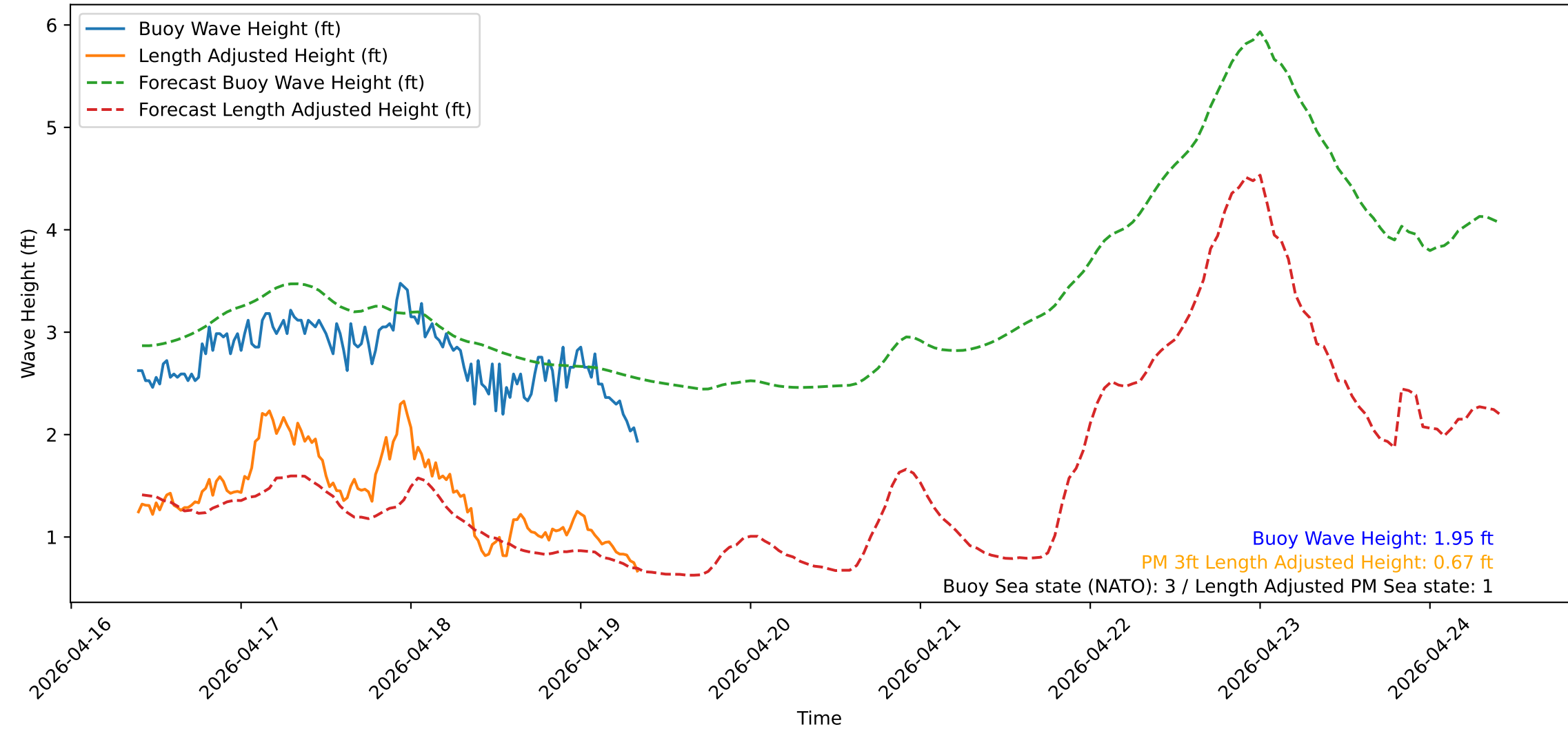
Wave Heights over Time for Green Beach at 2026-04-19 09:31:12
