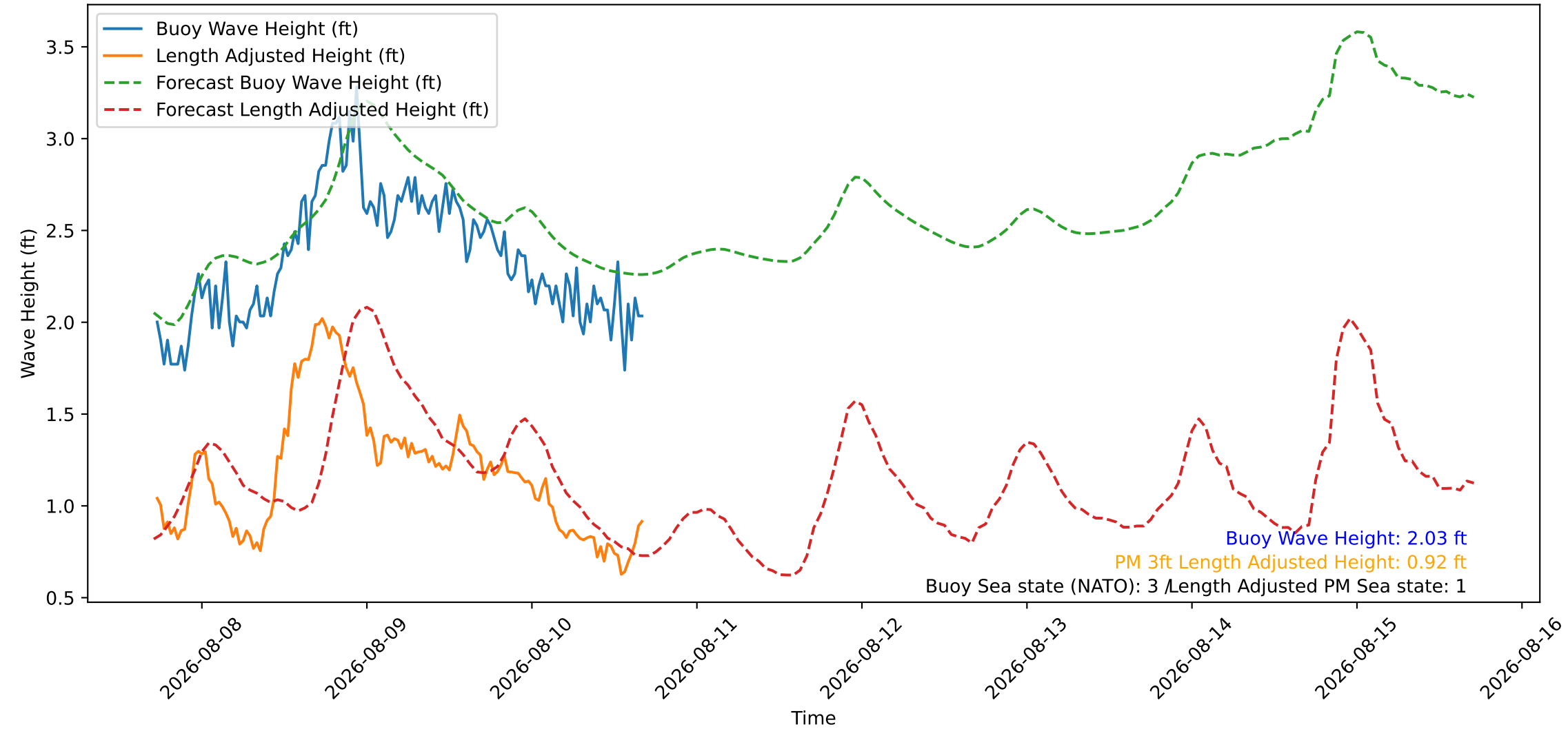
Wave Heights over Time for Red Beach at 2026-08-10 17:20:47
