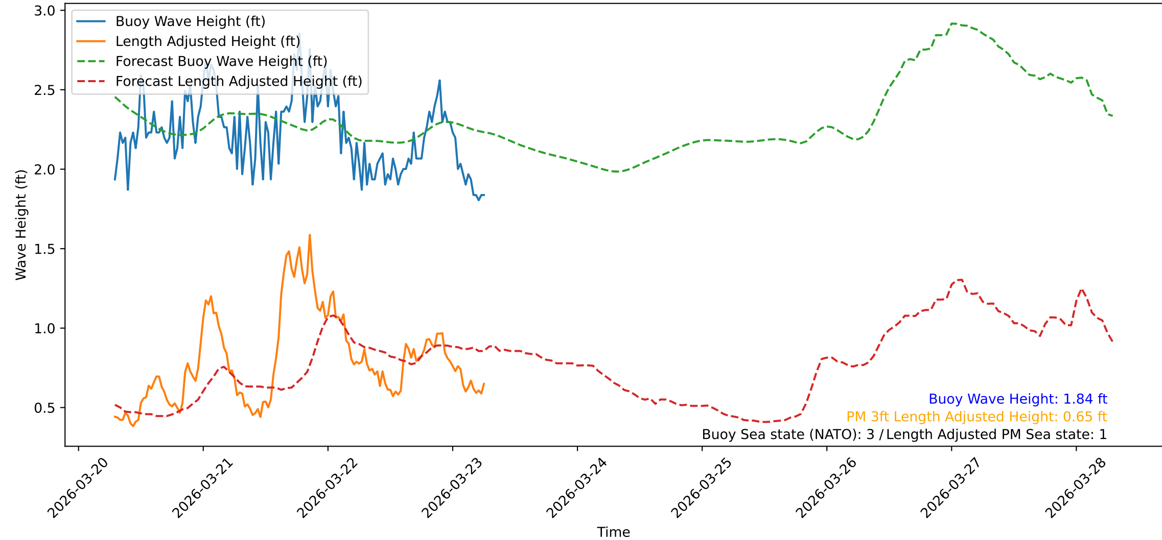
Wave Heights over Time for Red Beach at 2026-03-23 06:50:48
