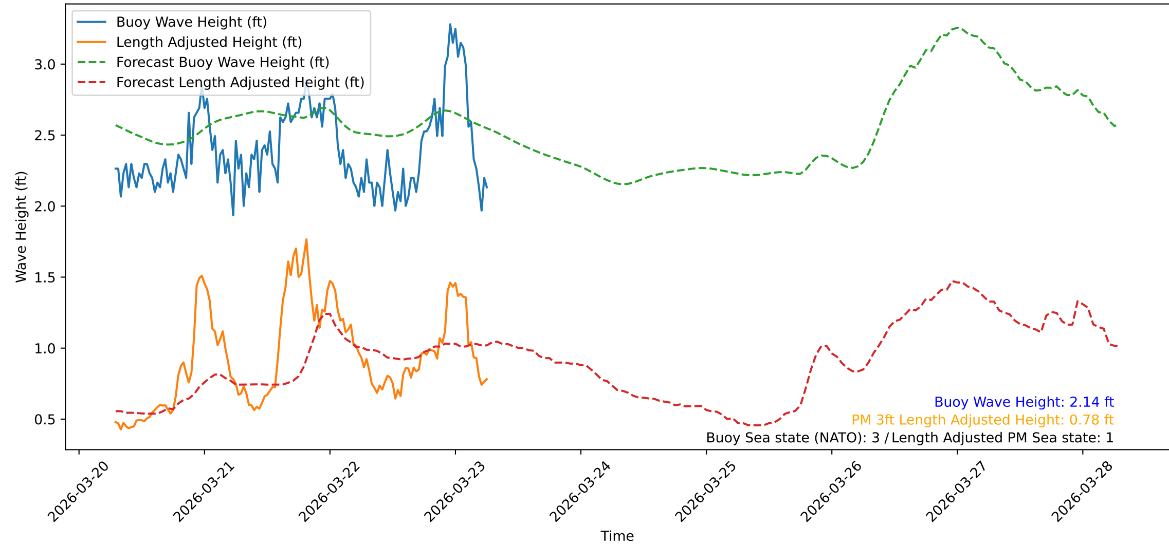
Wave Heights over Time for Green Beach at 2026-03-23 06:51:11
