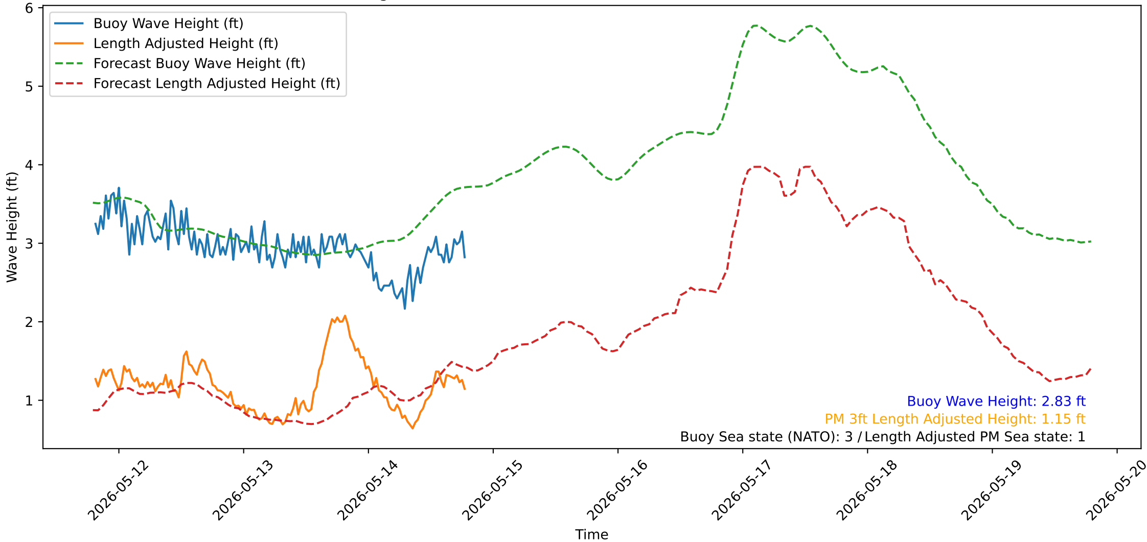
Wave Heights over Time for Oceanside Harbor at 2026-05-14 19:20:32
