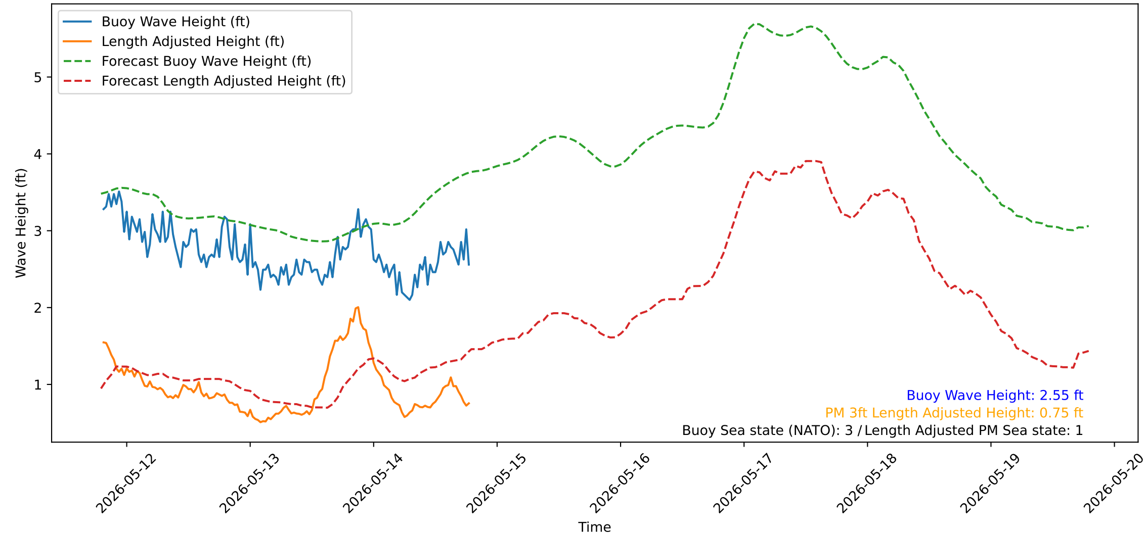
Wave Heights over Time for Green Beach at 2026-05-14 19:21:17
