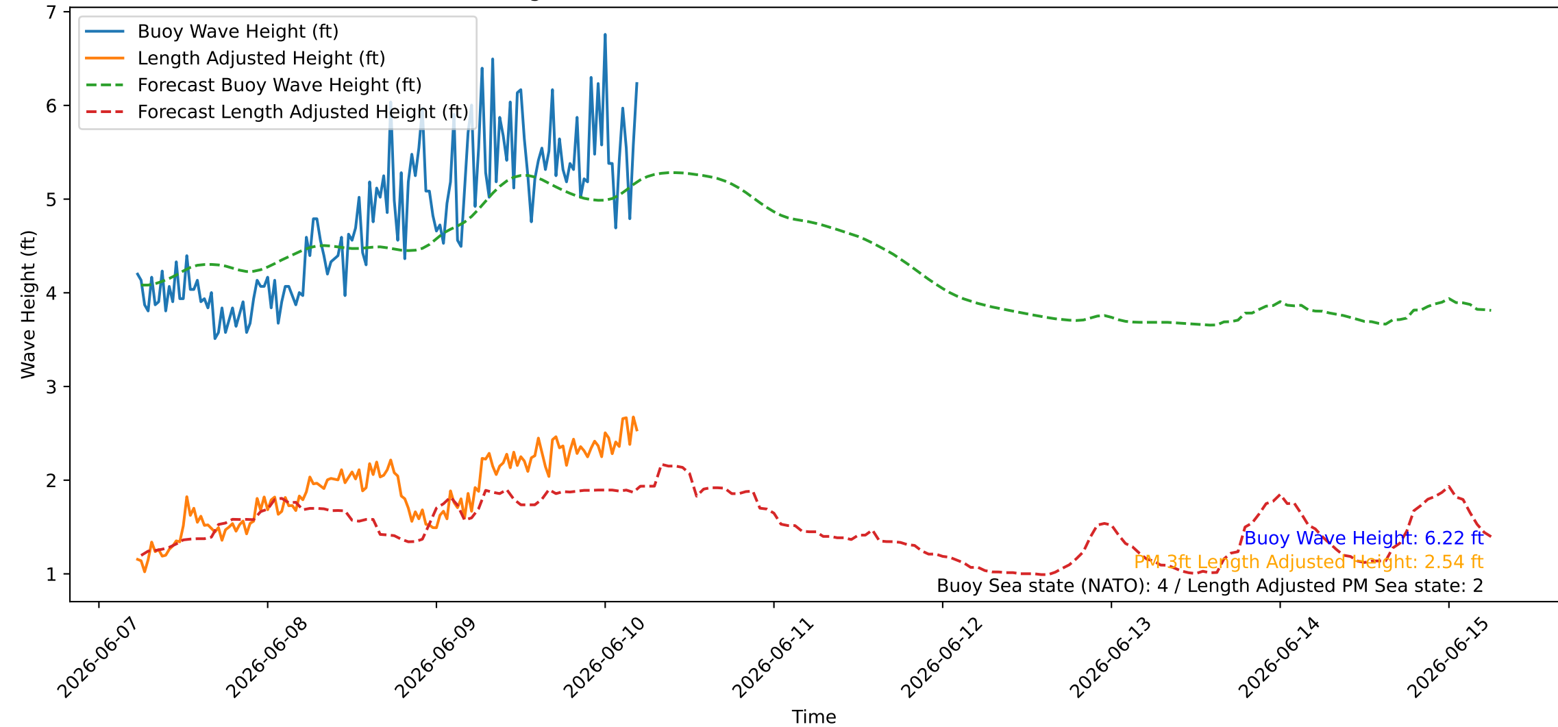
Wave Heights over Time for Oceanside Harbor at 2026-06-10 05:30:27
