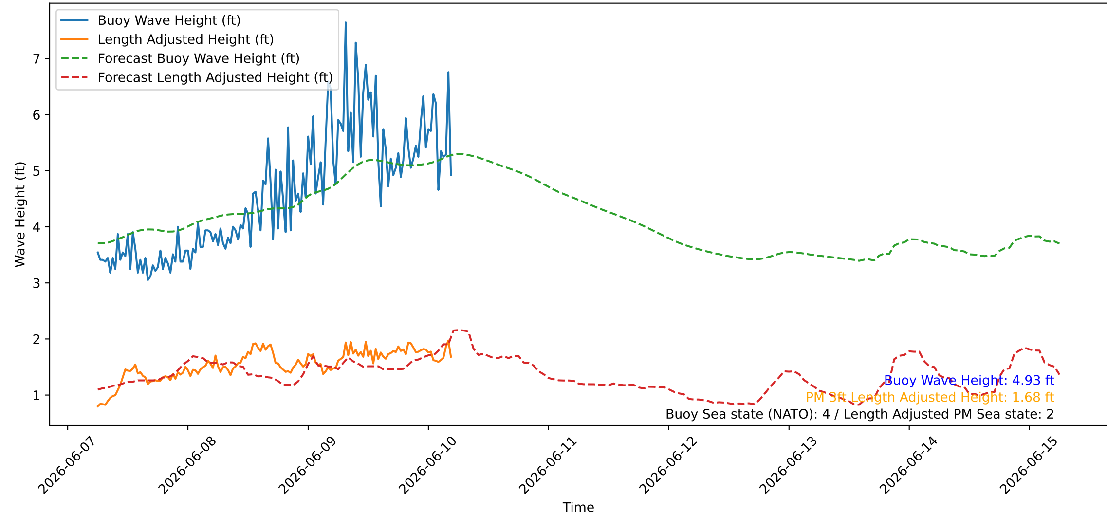
Wave Heights over Time for Red Beach at 2026-06-10 05:30:46
