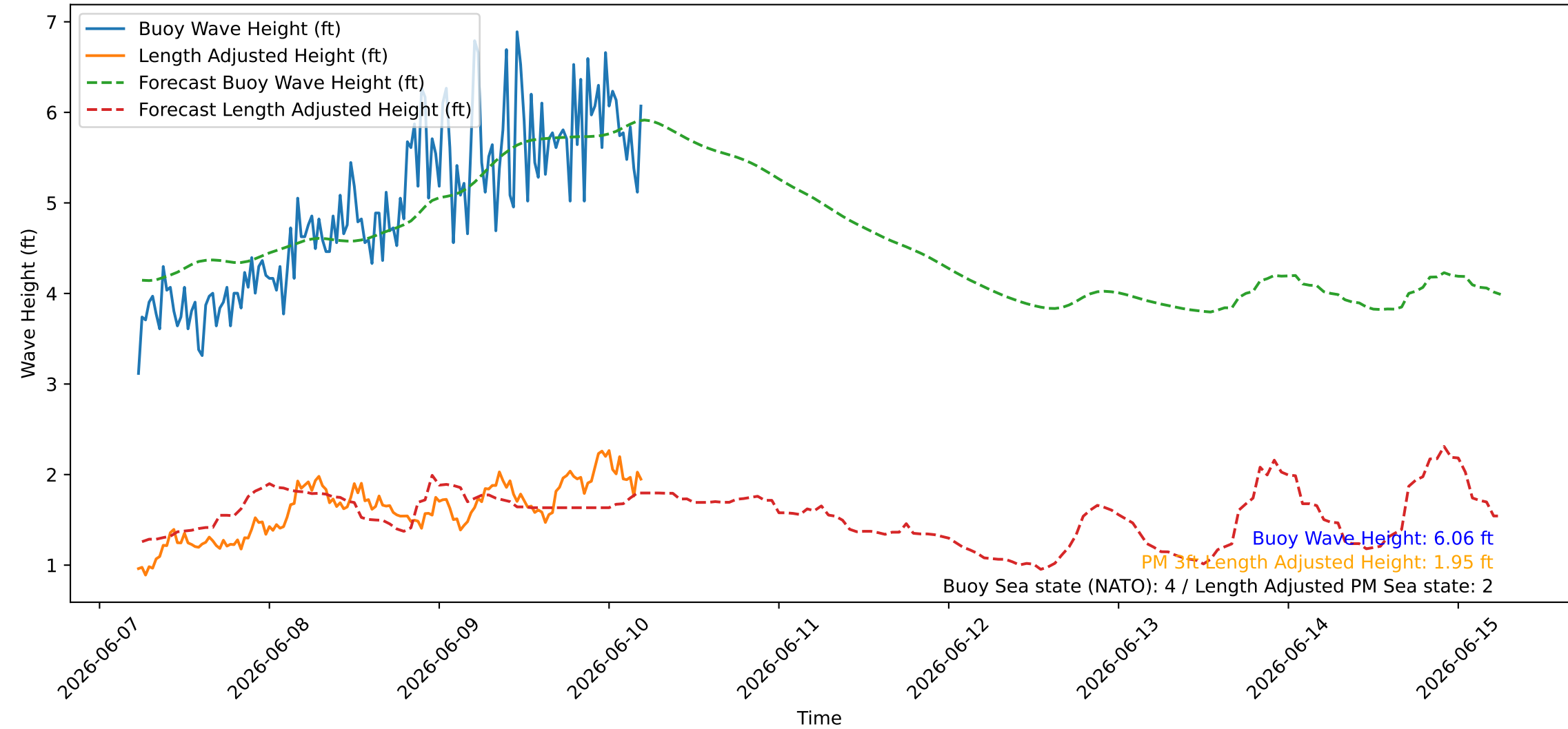
Wave Heights over Time for Green Beach at 2026-06-10 05:31:10
