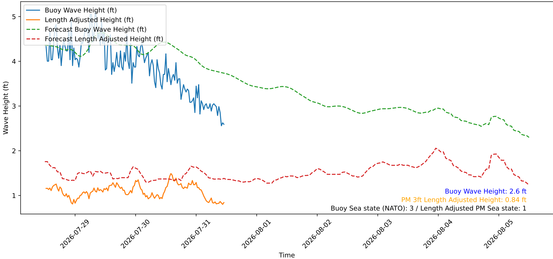
Wave Heights over Time for Red Beach at 2026-07-31 12:00:46
