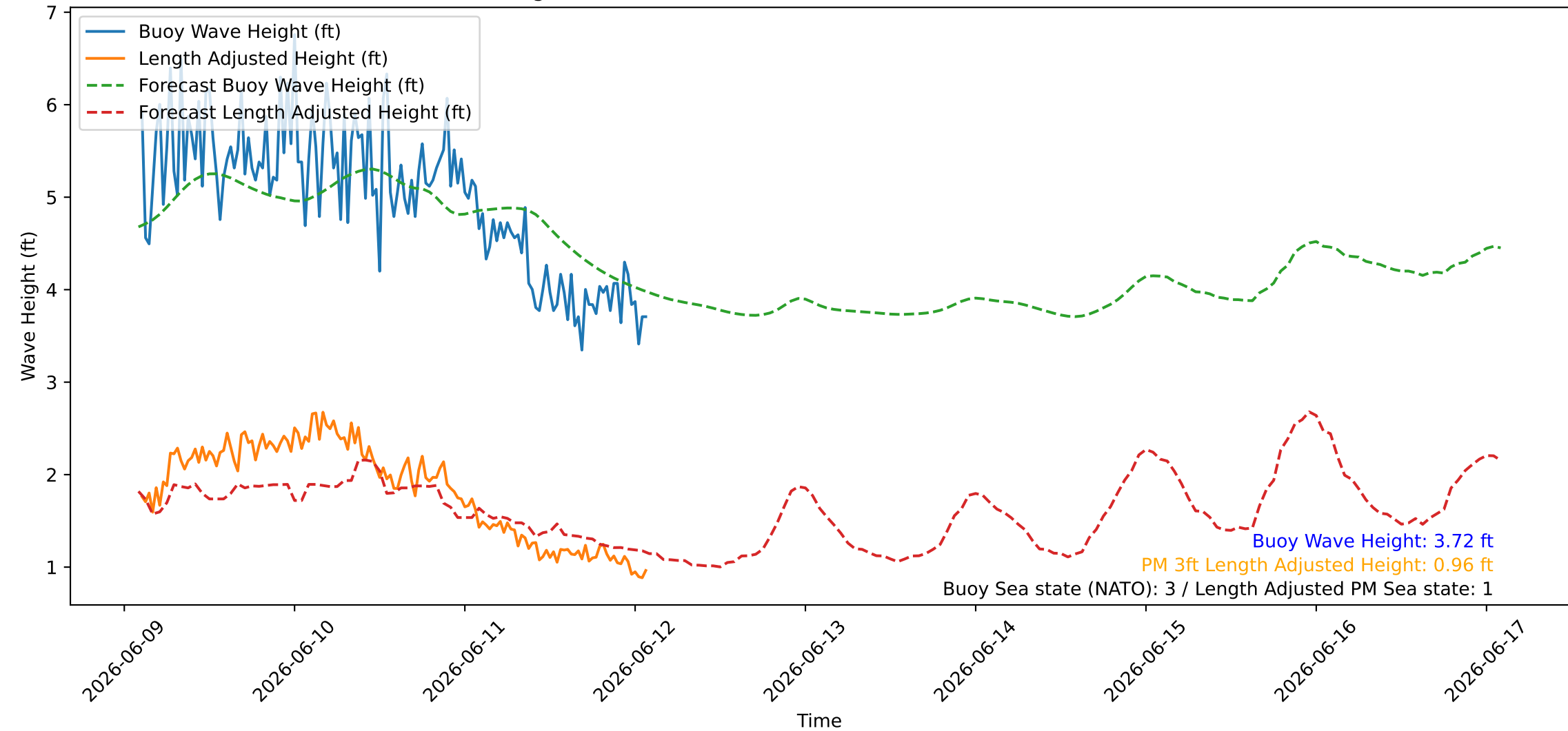
Wave Heights over Time for Oceanside Harbor at 2026-06-12 02:20:26
