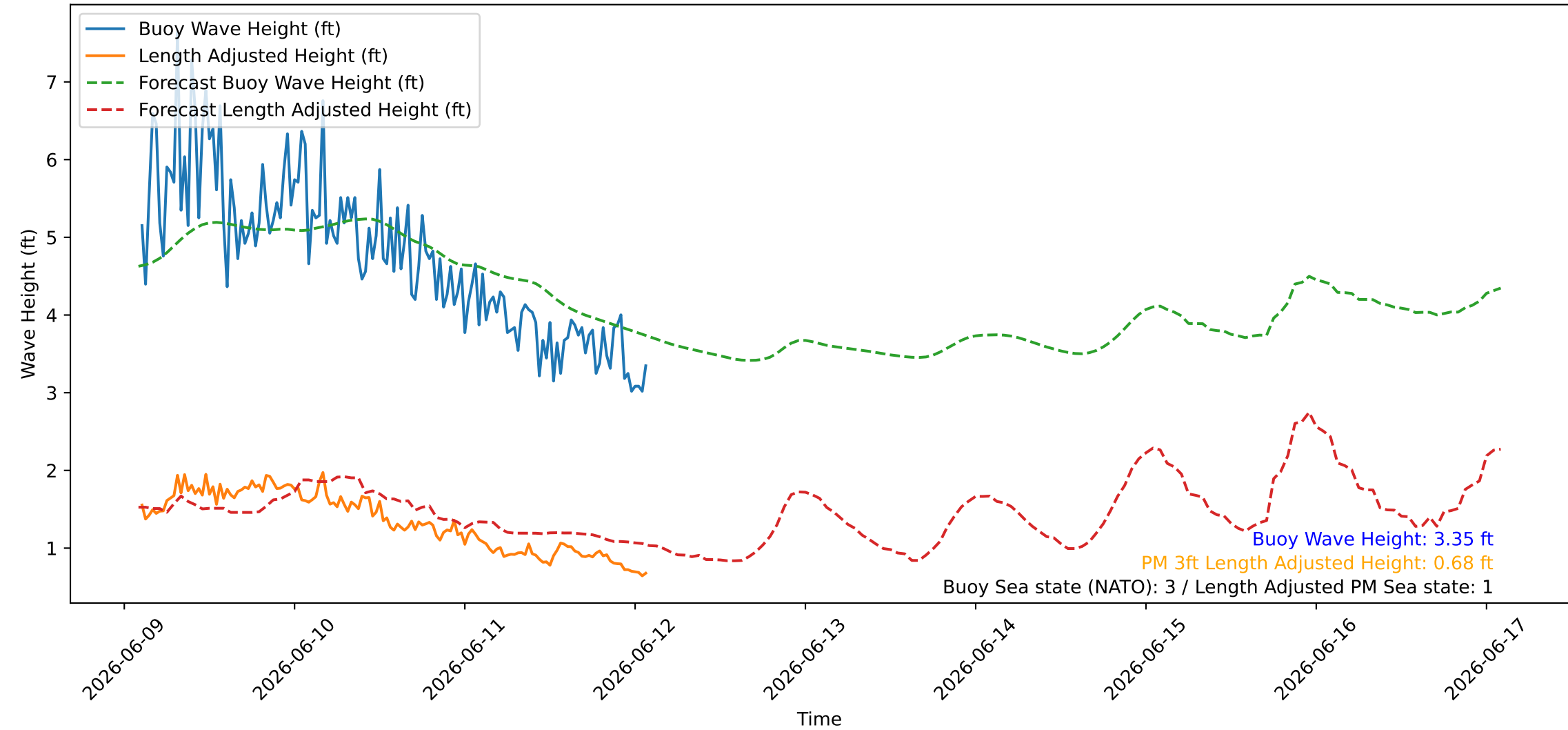
Wave Heights over Time for Red Beach at 2026-06-12 02:20:47
