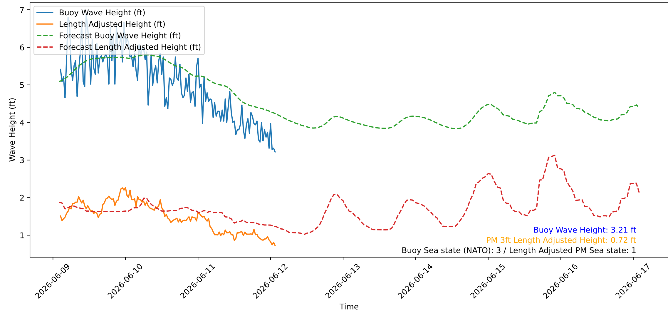
Wave Heights over Time for Green Beach at 2026-06-12 02:21:10
