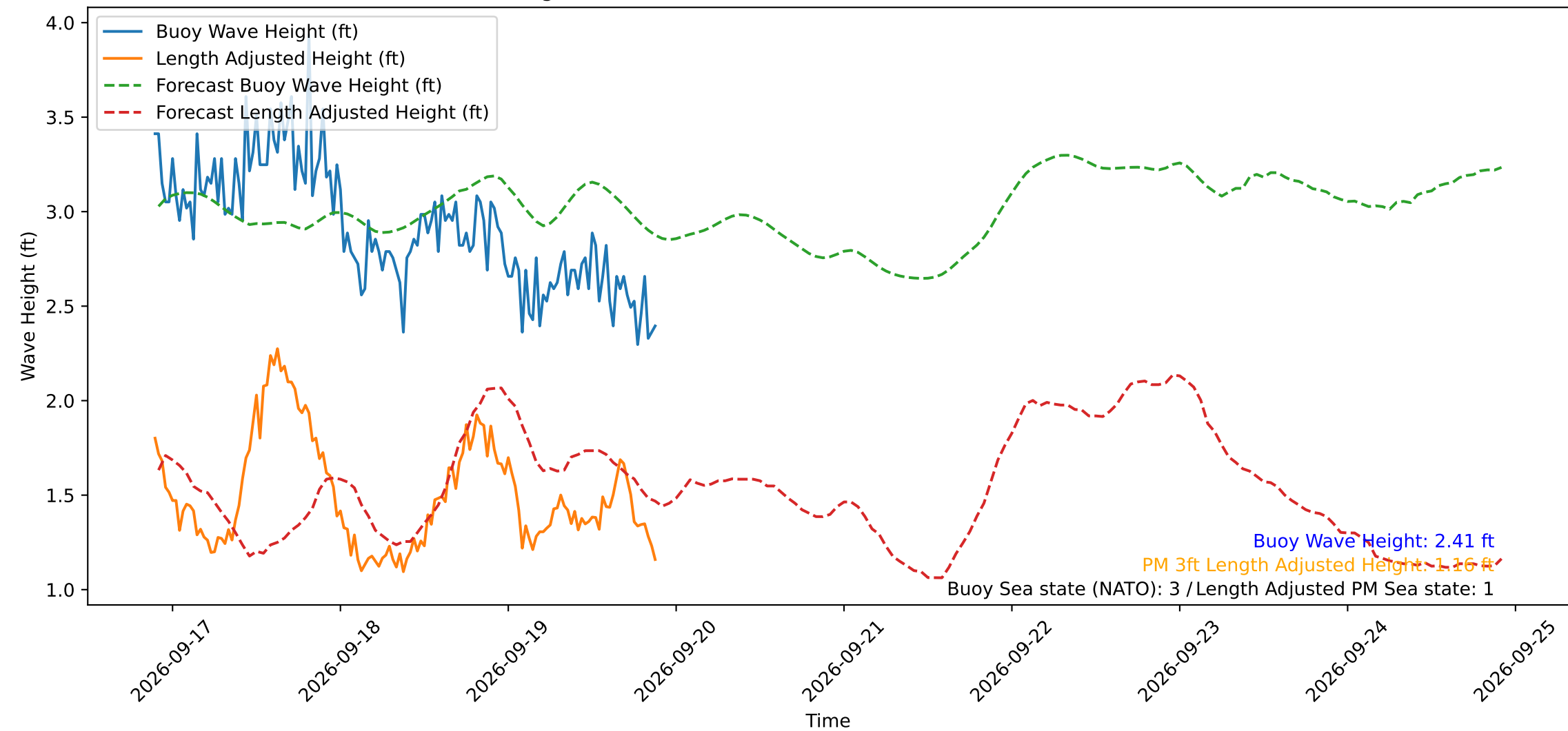
Wave Heights over Time for Oceanside Harbor at 2026-09-19 21:30:30
