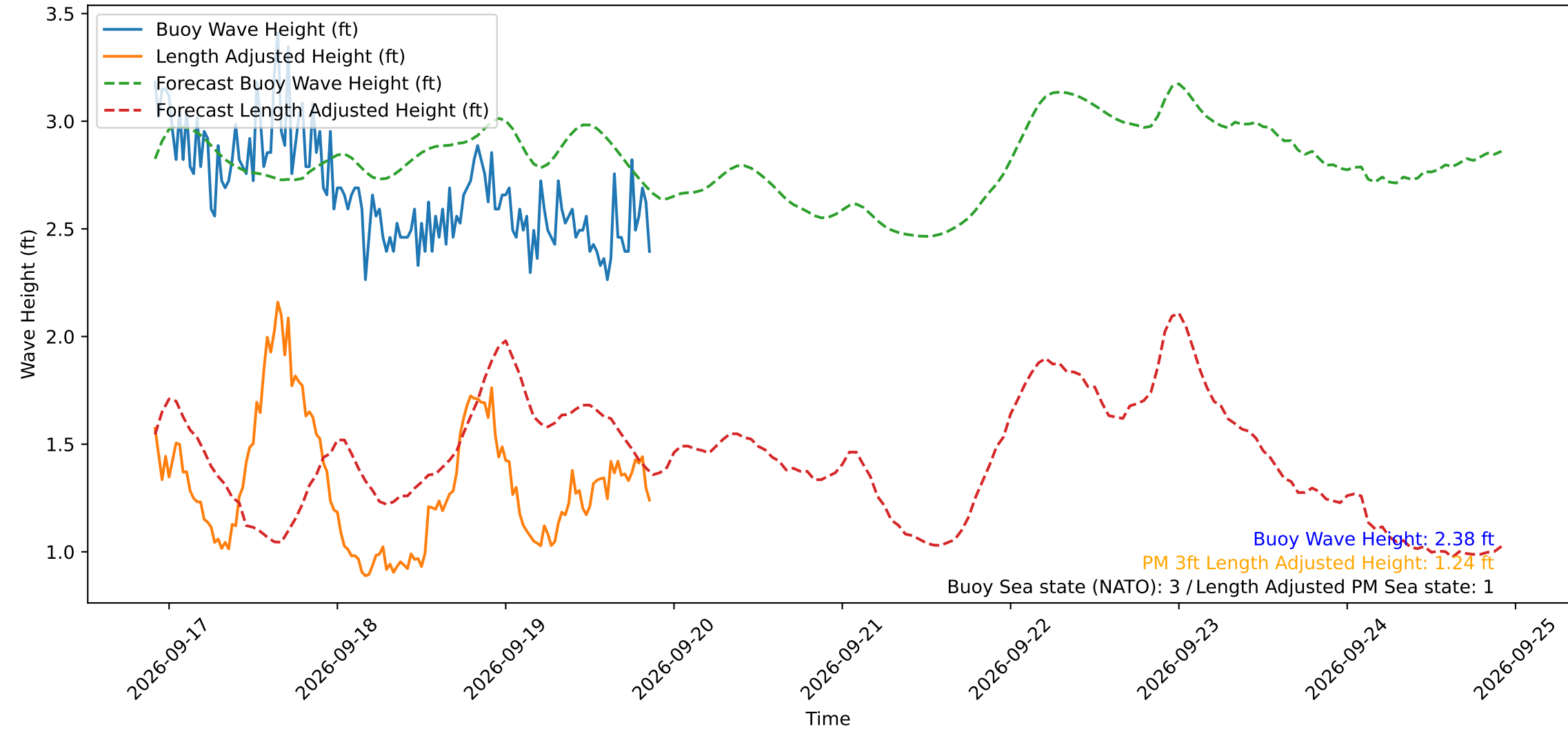
Wave Heights over Time for Red Beach at 2026-09-19 21:30:49
