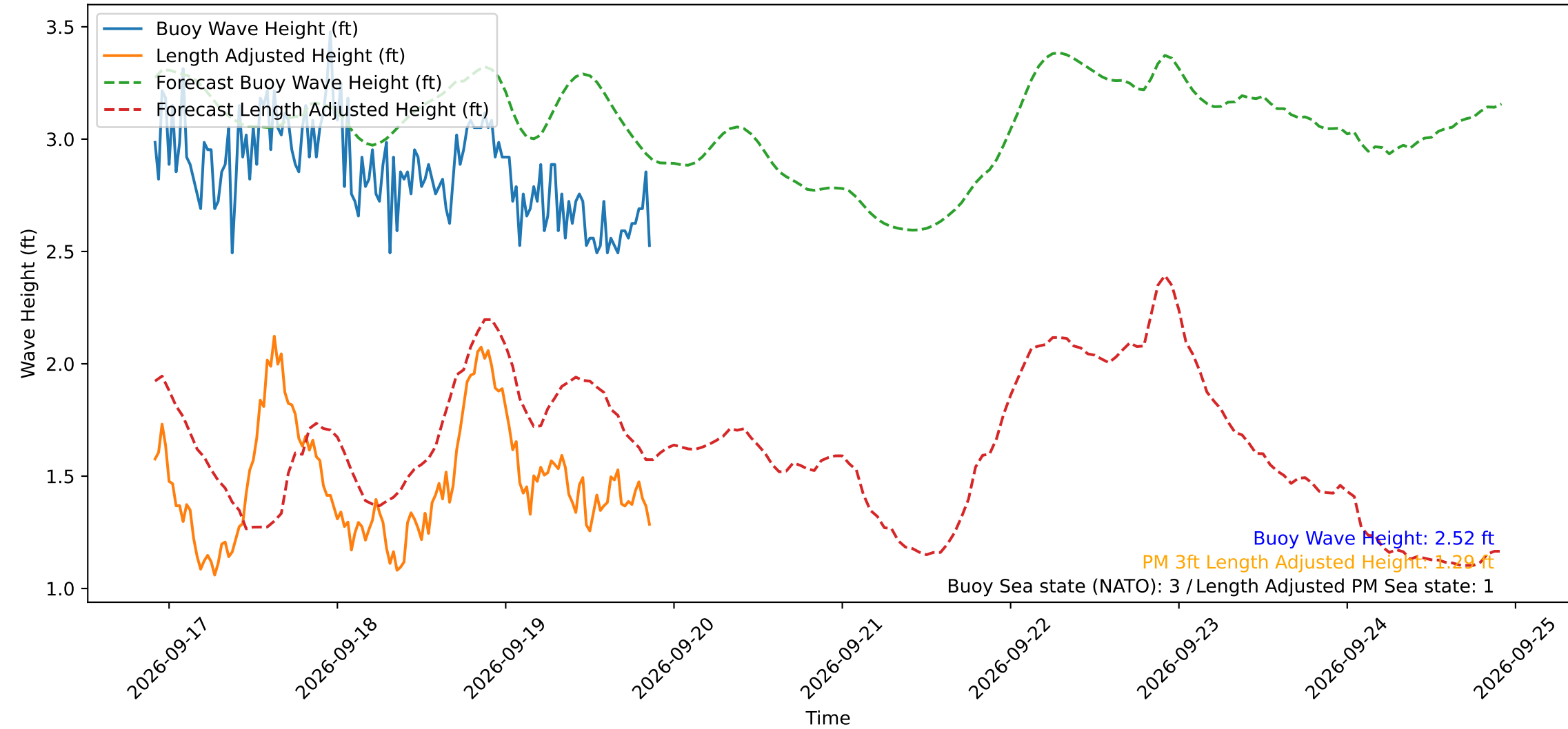
Wave Heights over Time for Green Beach at 2026-09-19 21:31:11
