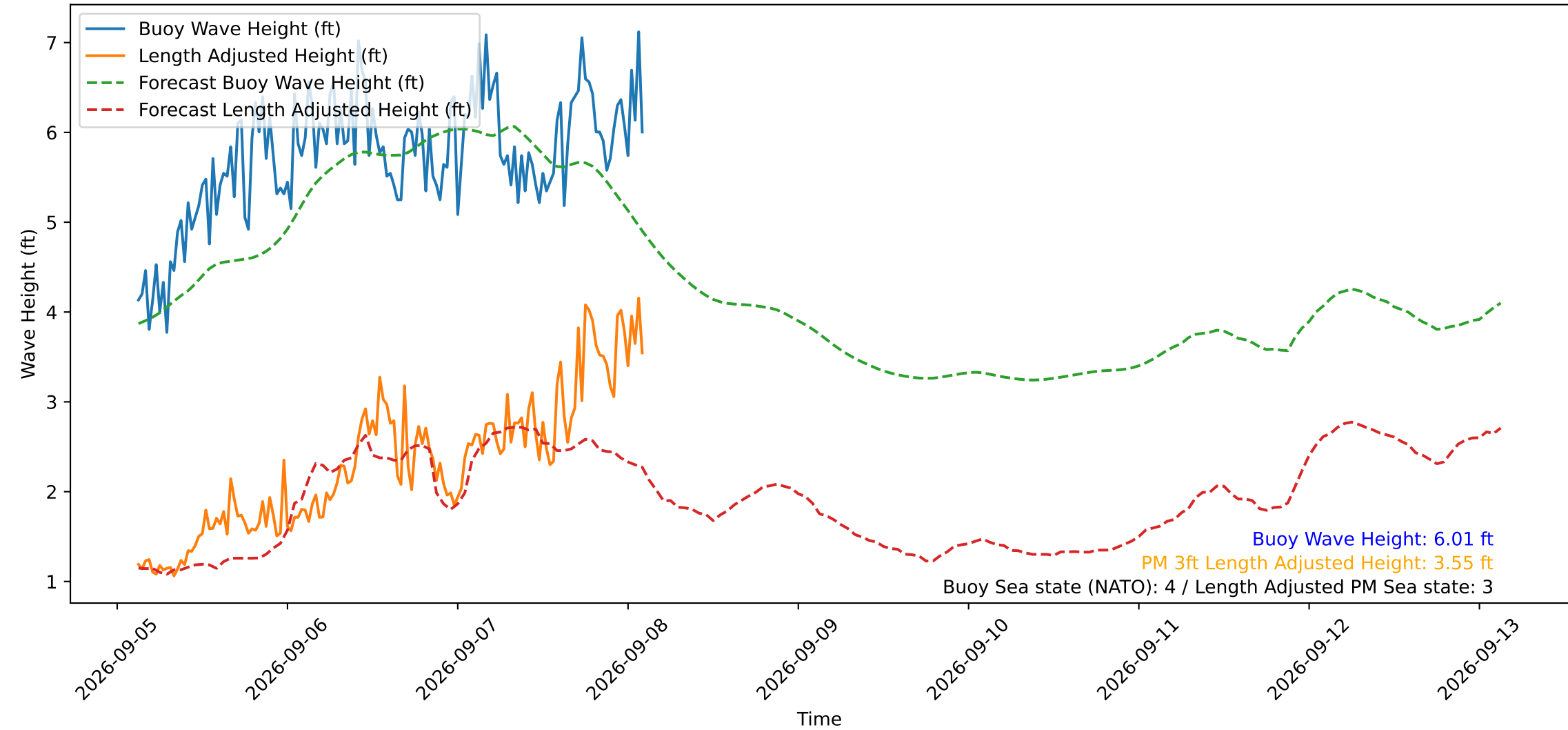
Wave Heights over Time for Oceanside Harbor at 2026-09-08 02:50:29
